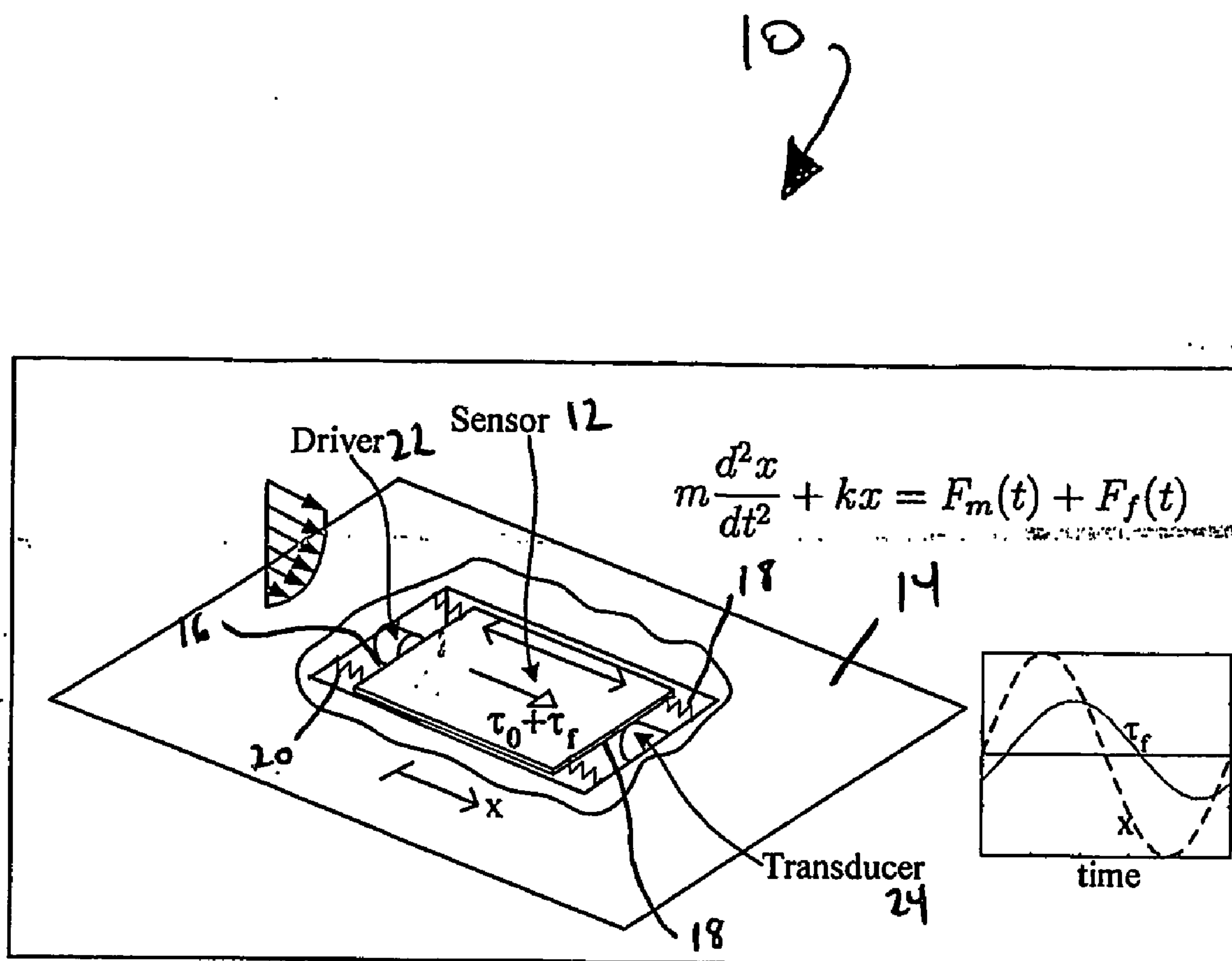
Fig. 1 - Schematic of dynamic resonant shear stress sensor with the governing equation and a time history of the fluctuating shear force on the sensor (from a simulation). A cutaway view of the sensor is shown to display components below the surface.
