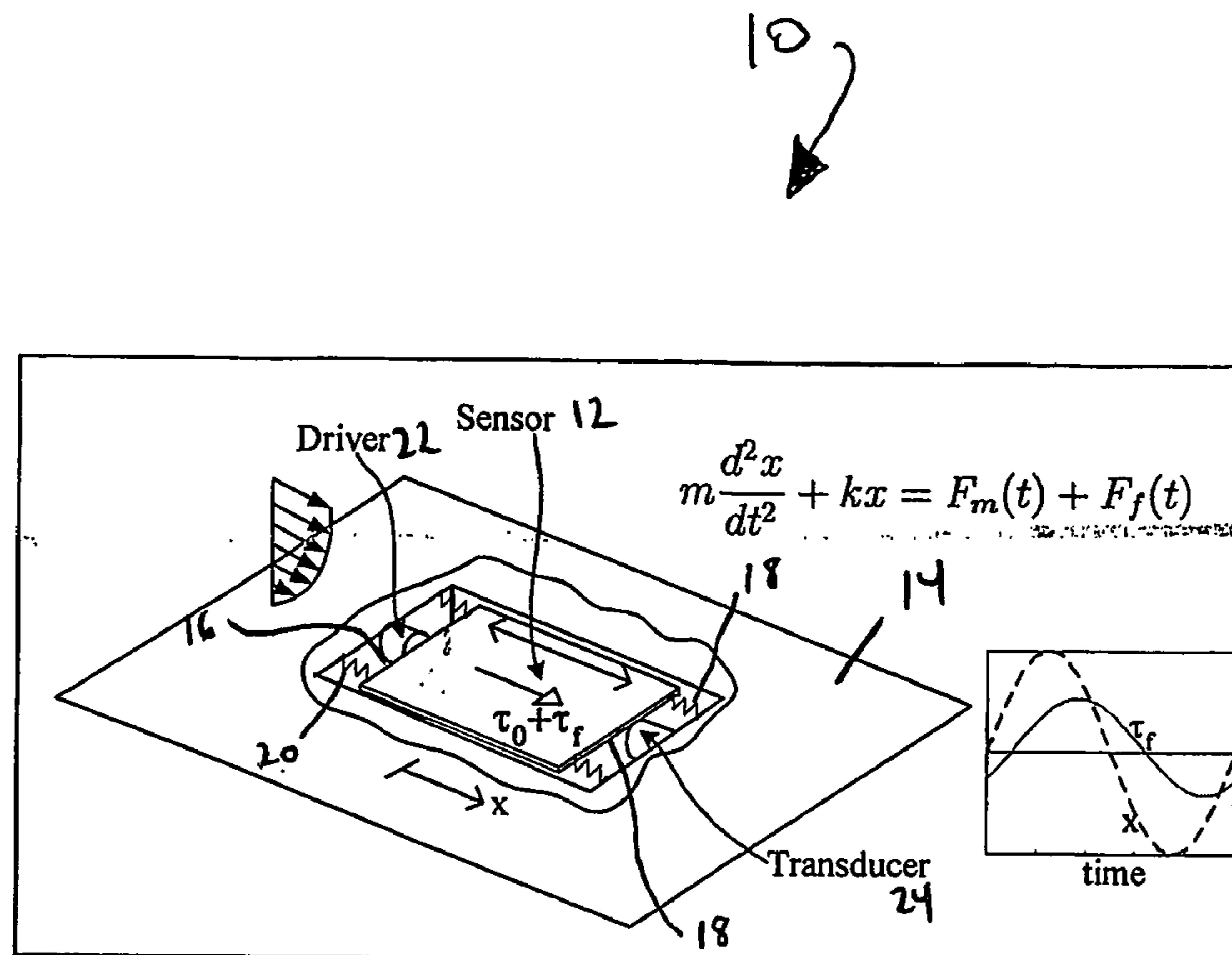
Schematic of dynamic resonant shear stress sensor with the governing equation and a time history of the fluctuating shear force on the sensor (from a simulation). A cutaway view of the sensor is shown to display components below the surface.
