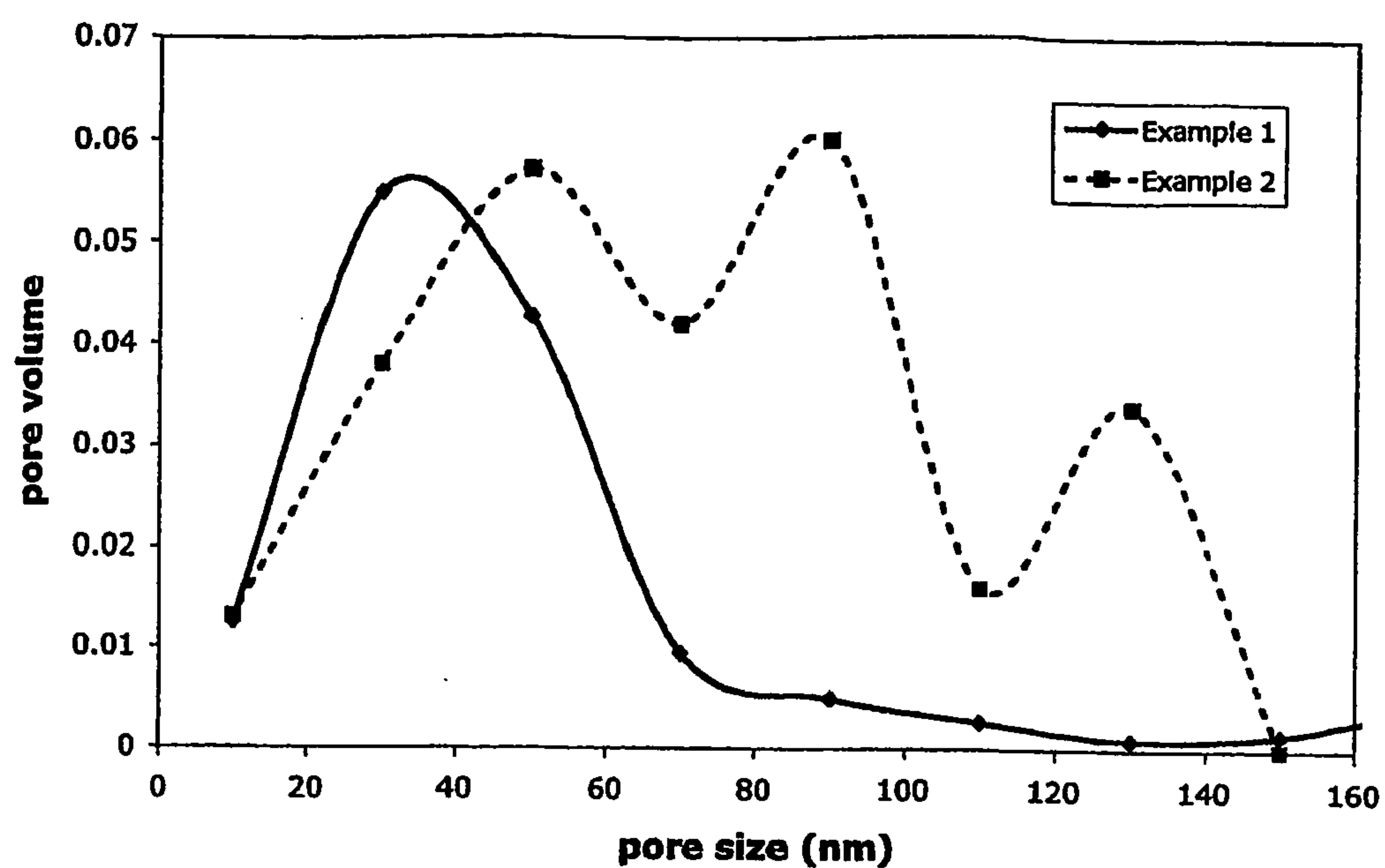
Figure 1. Pore size distributions for the metal oxides produced in examples 1 and 2.
