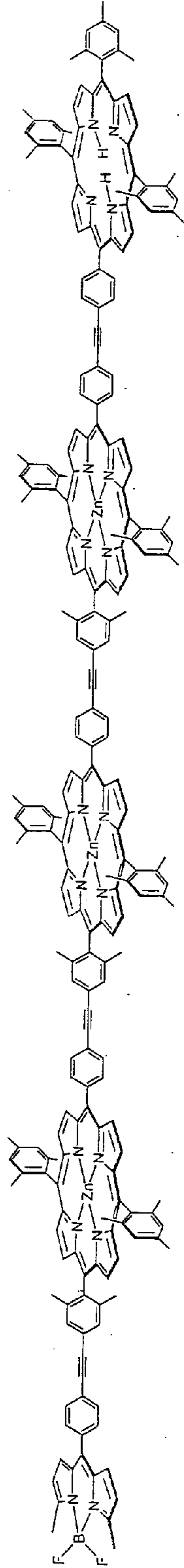
Figure H.2. Example of a porphyrin molecular wire where metalloporphyrins and/or free base porphyrins are joined via diphenylethyne. ...
