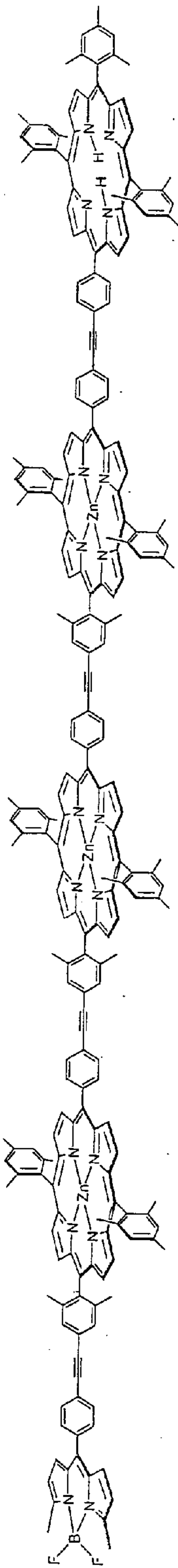
Figure H.2. Example of a porphyrin molecular wire where metalloporphyrins and/or free base porphyrins are joined via diphenylethyne. ...
