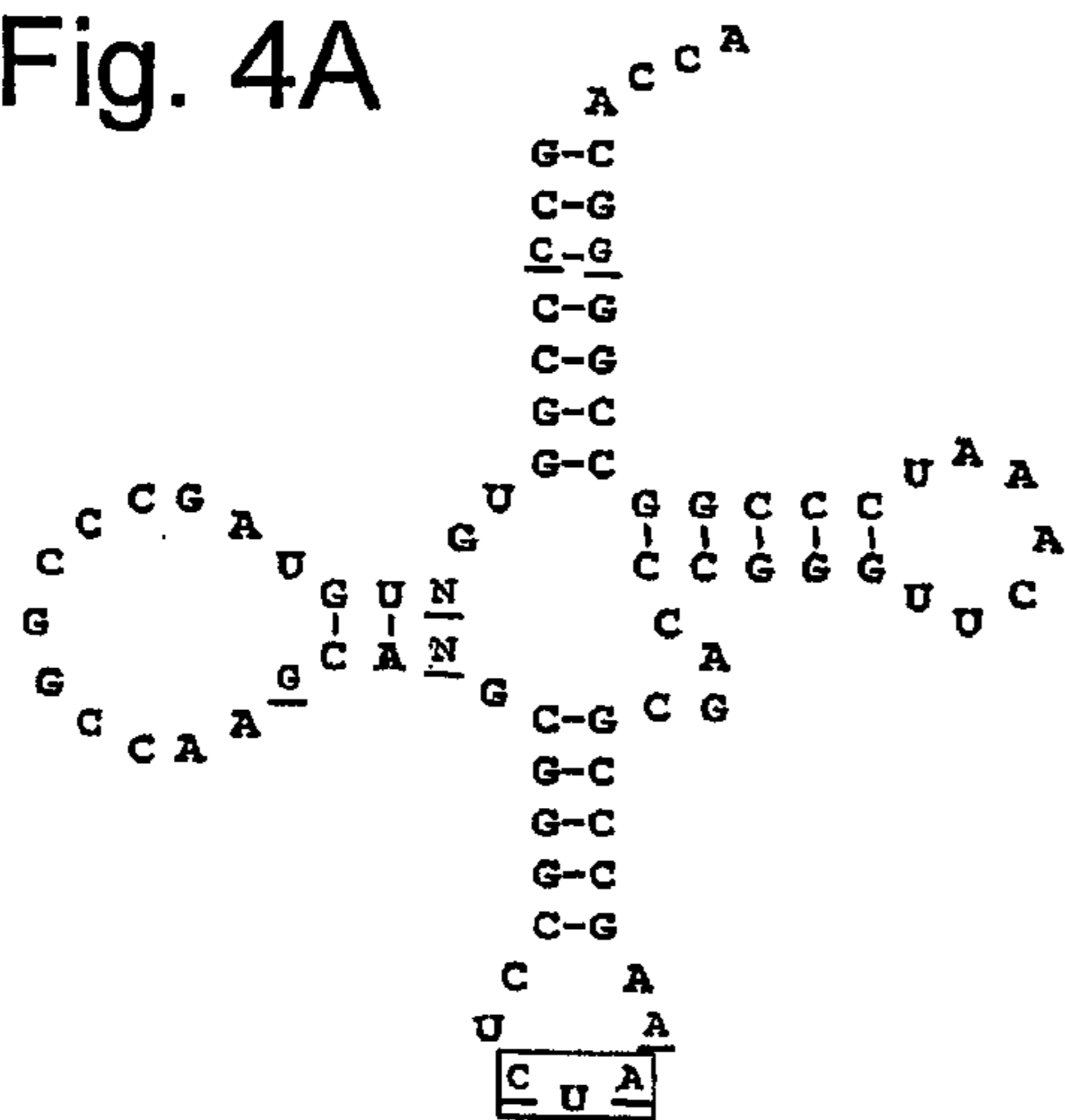
AE(NN) tRNA library
