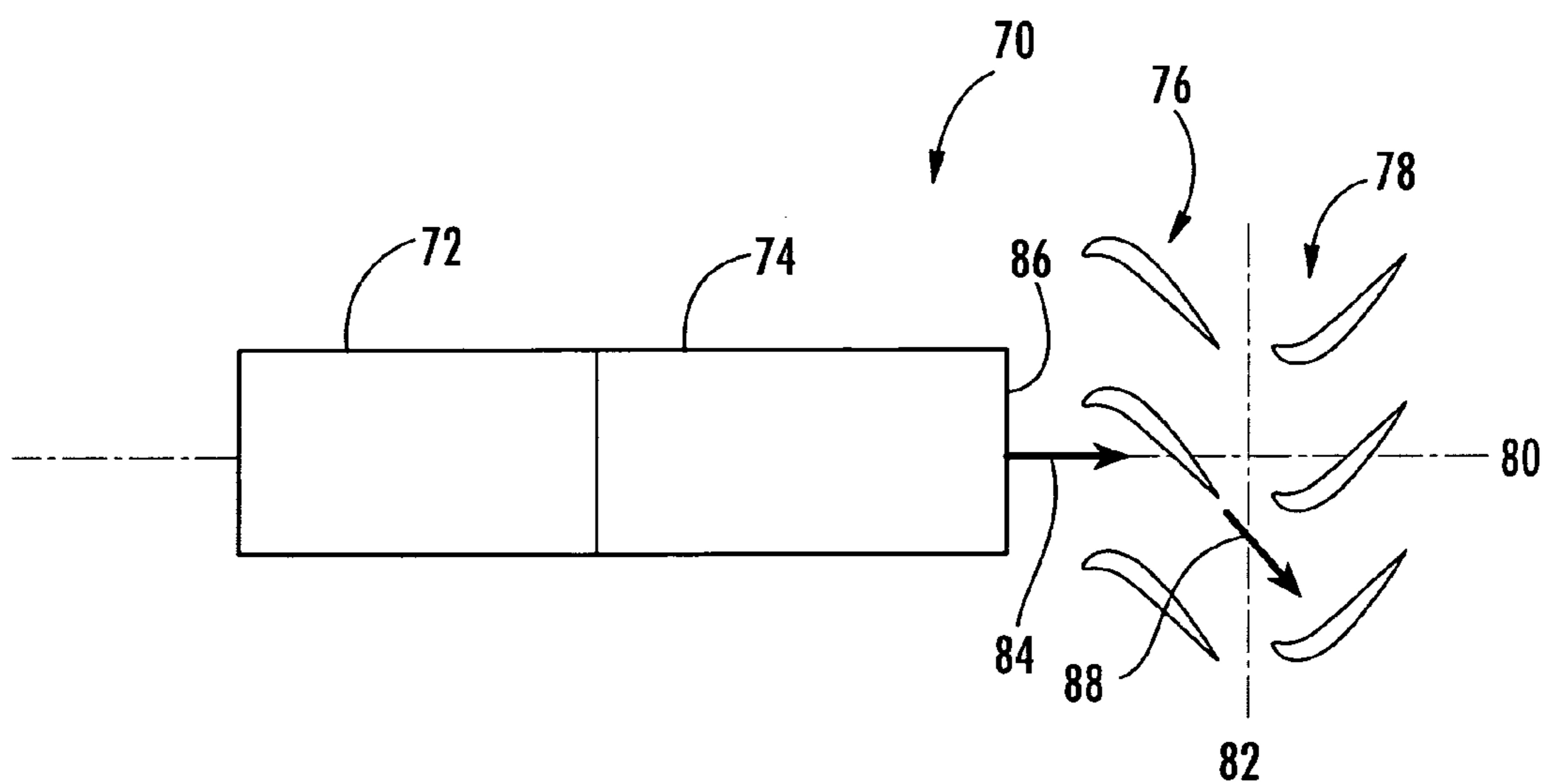
FIG. 3 (PRIOR ART)
