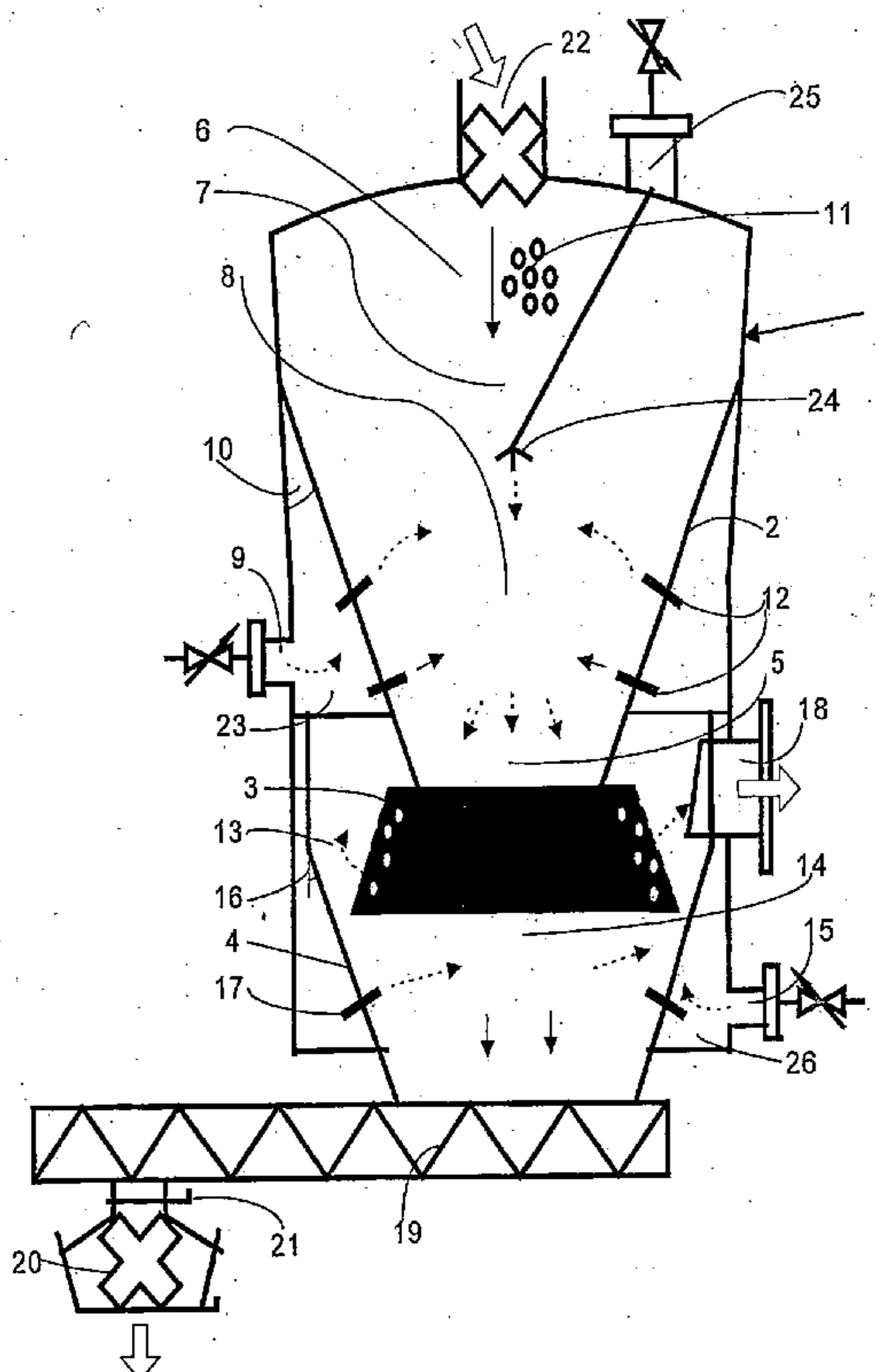
Gasifier (1)
