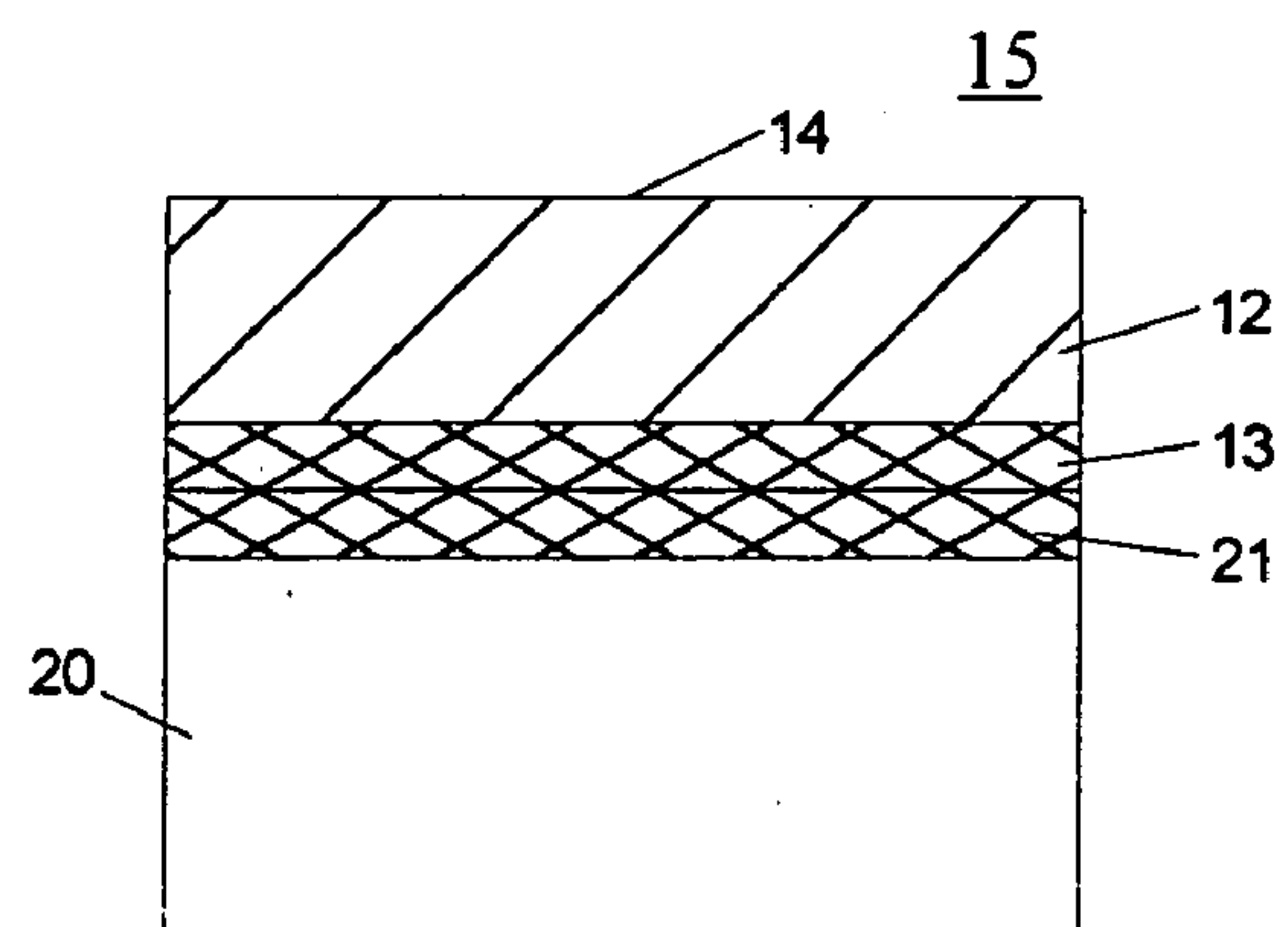
FIG. 2H: Polish Wafer
