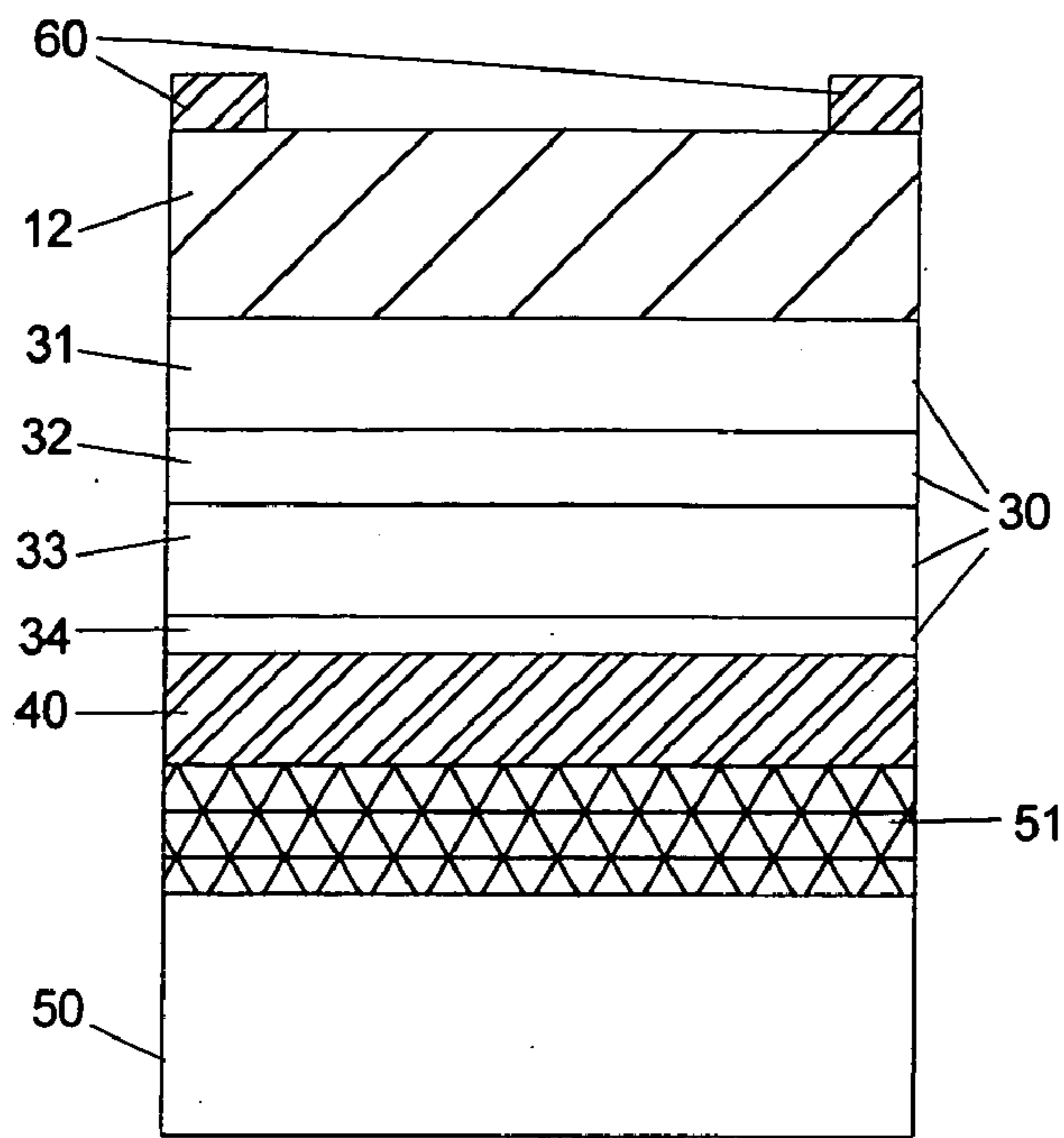
FIG. 20: Ohmic Contact Formation
