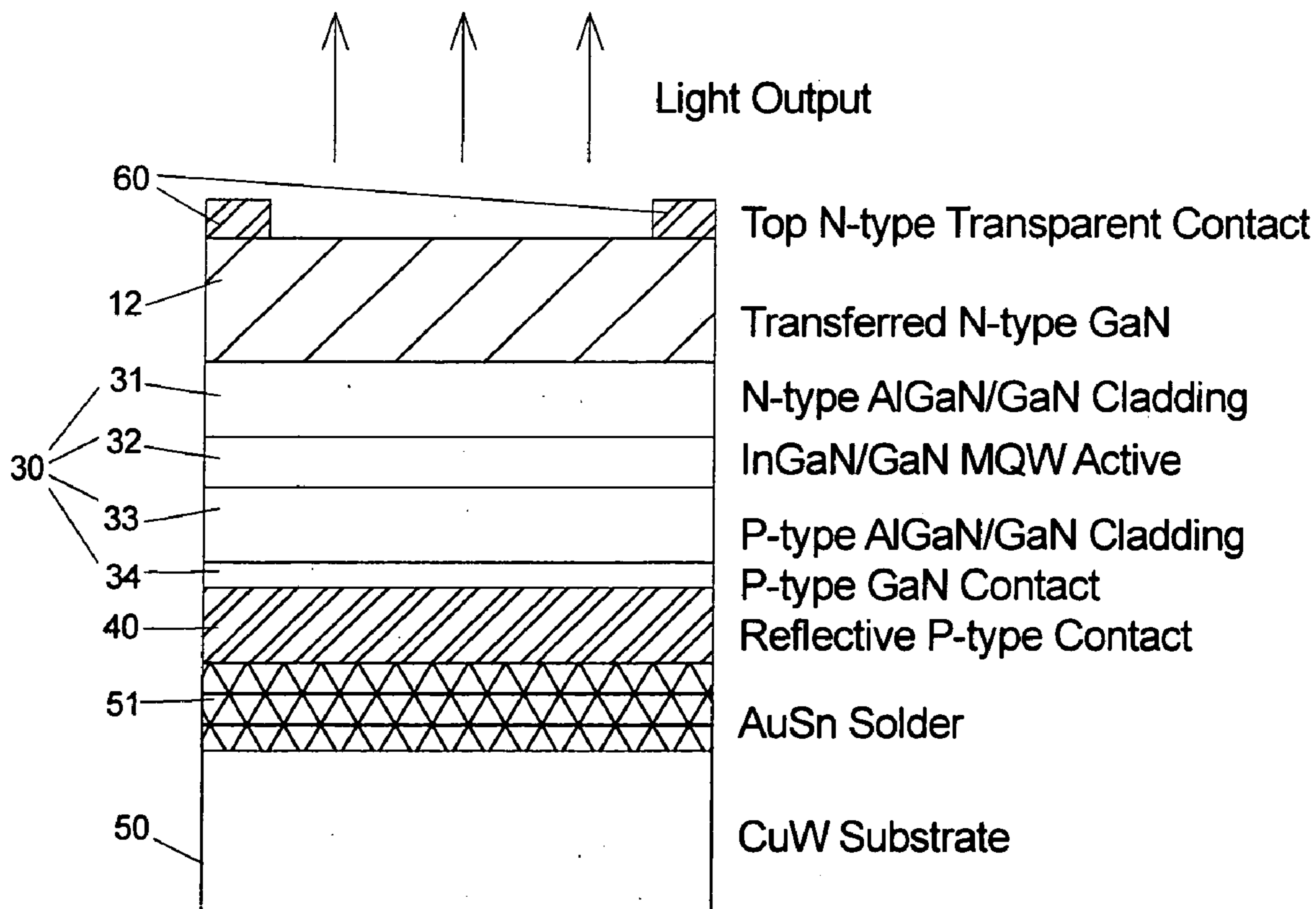
Completed LED Device
