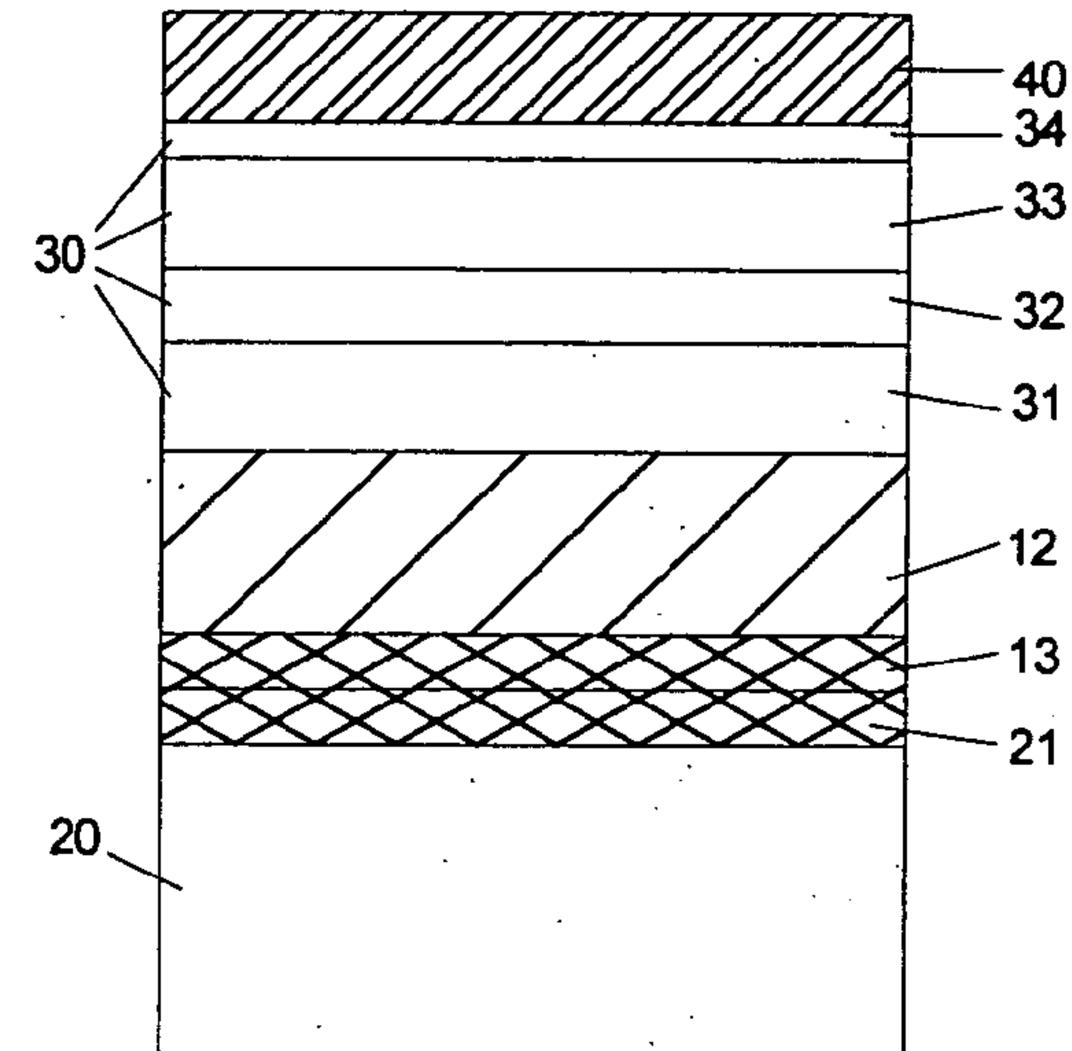
FIG. 2J: Ohmic Contact Formation
