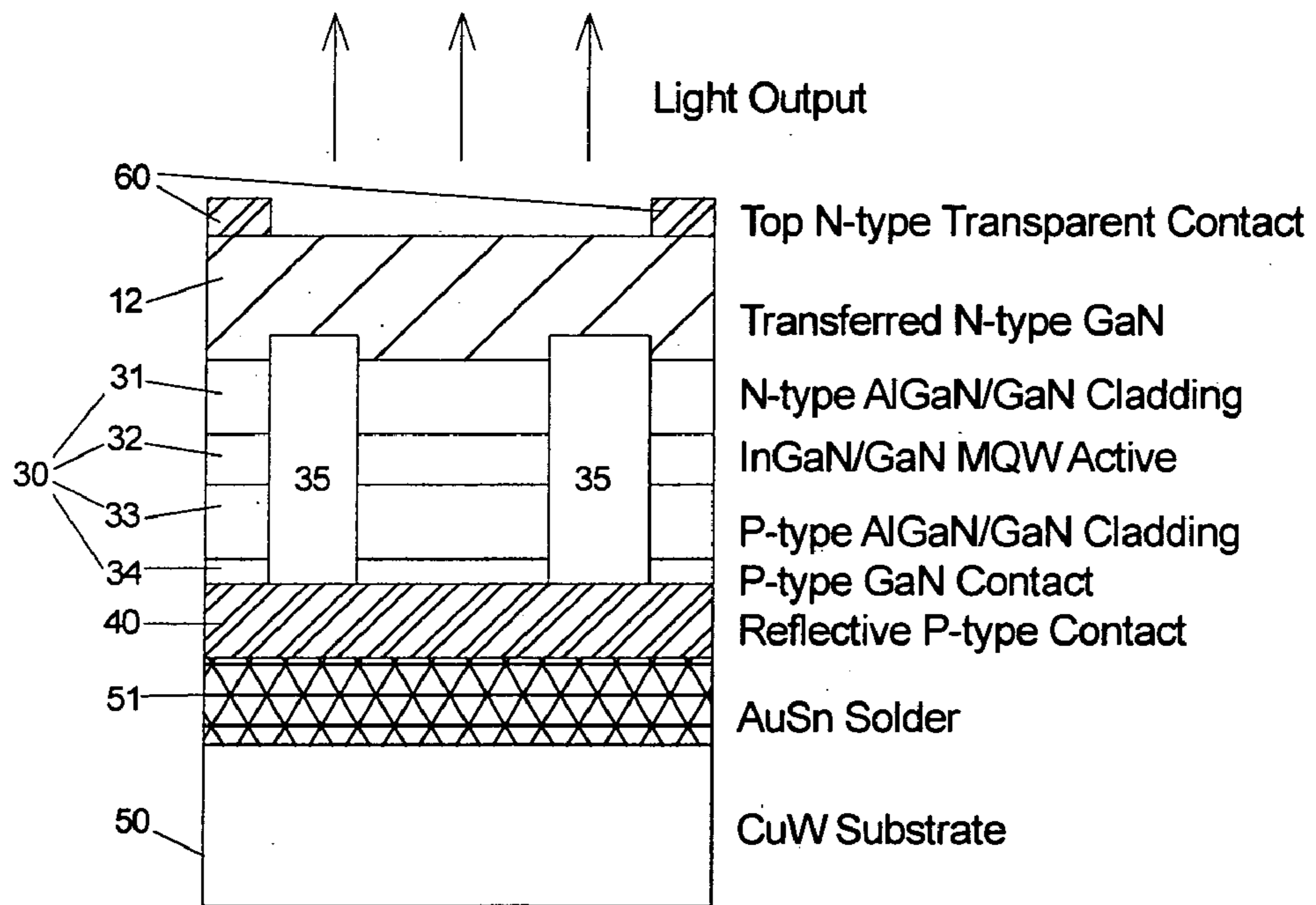
FIG. 6: Completed LED Device
