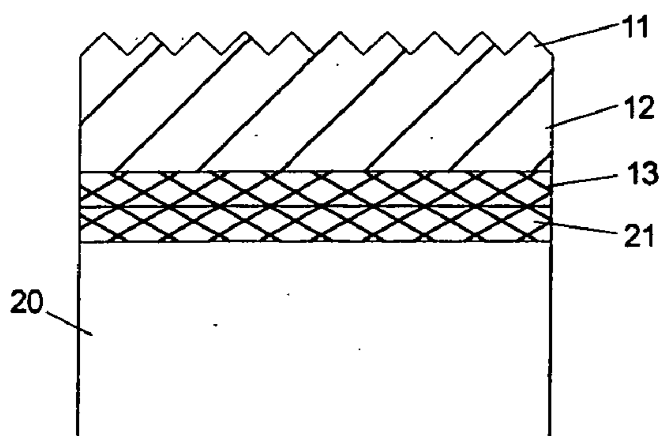
FIG. 2G: Exfoliate GaN Film
