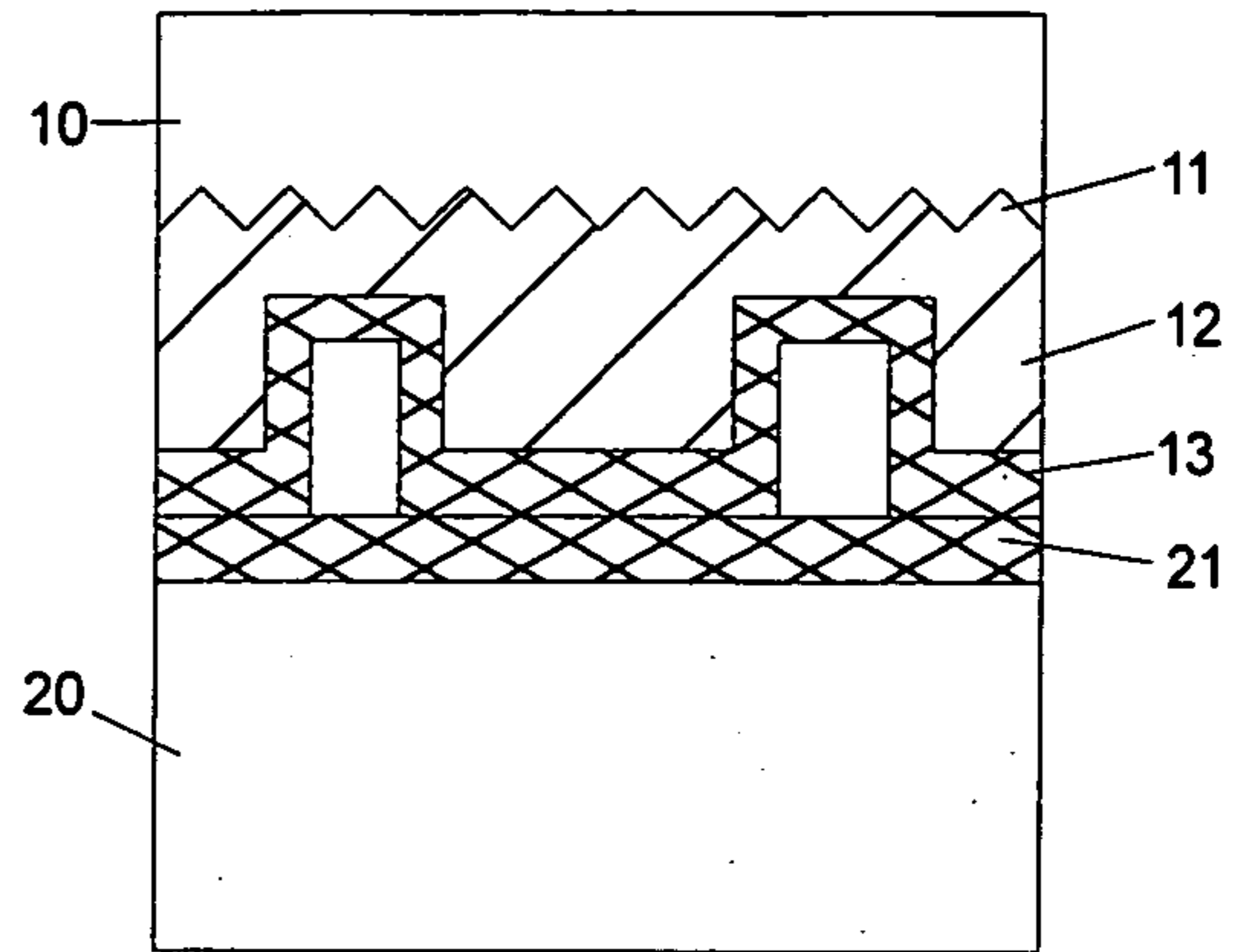
FIG. 3C: Bond Wafer
