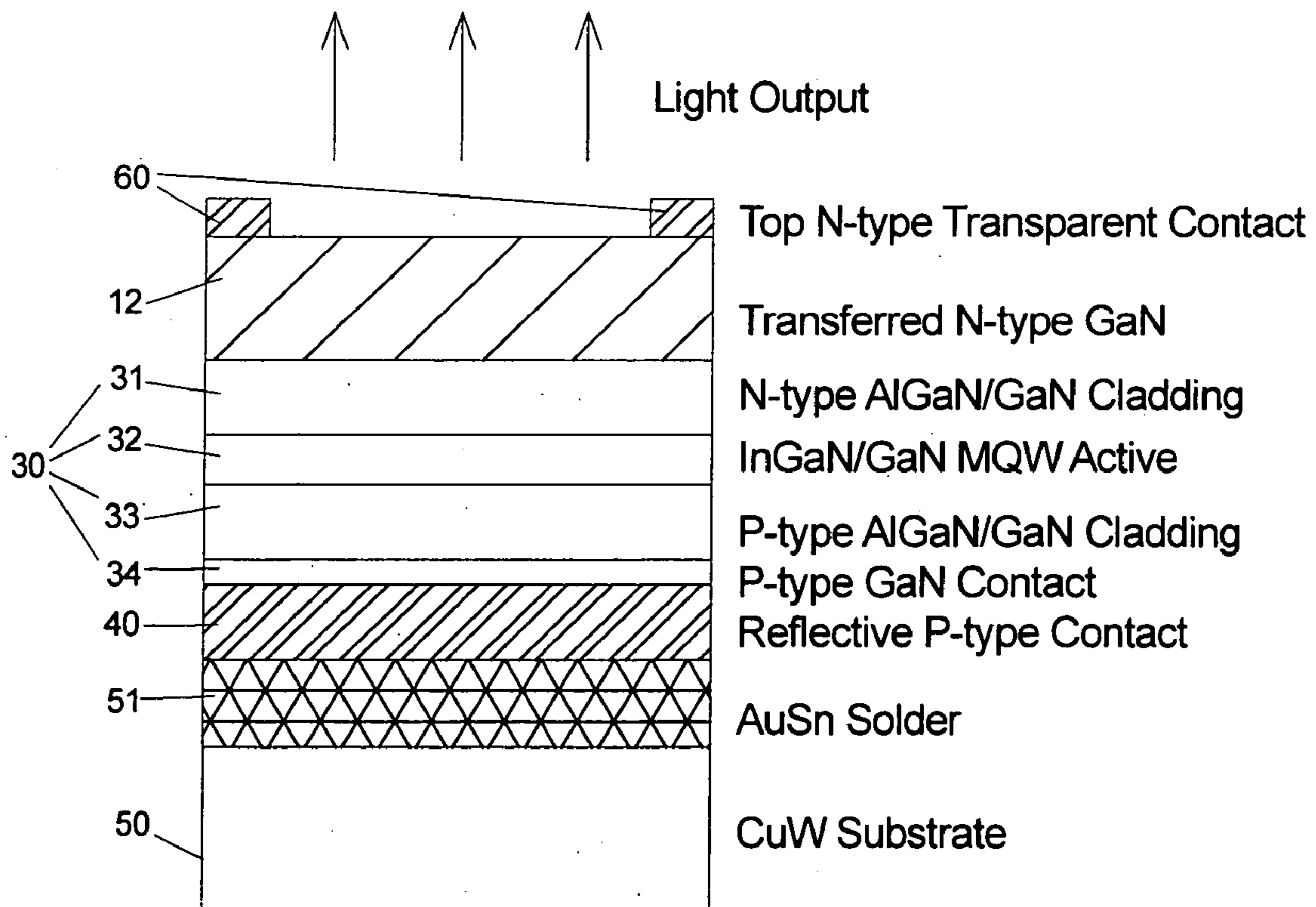
FIG. 1: Completed LED Device
