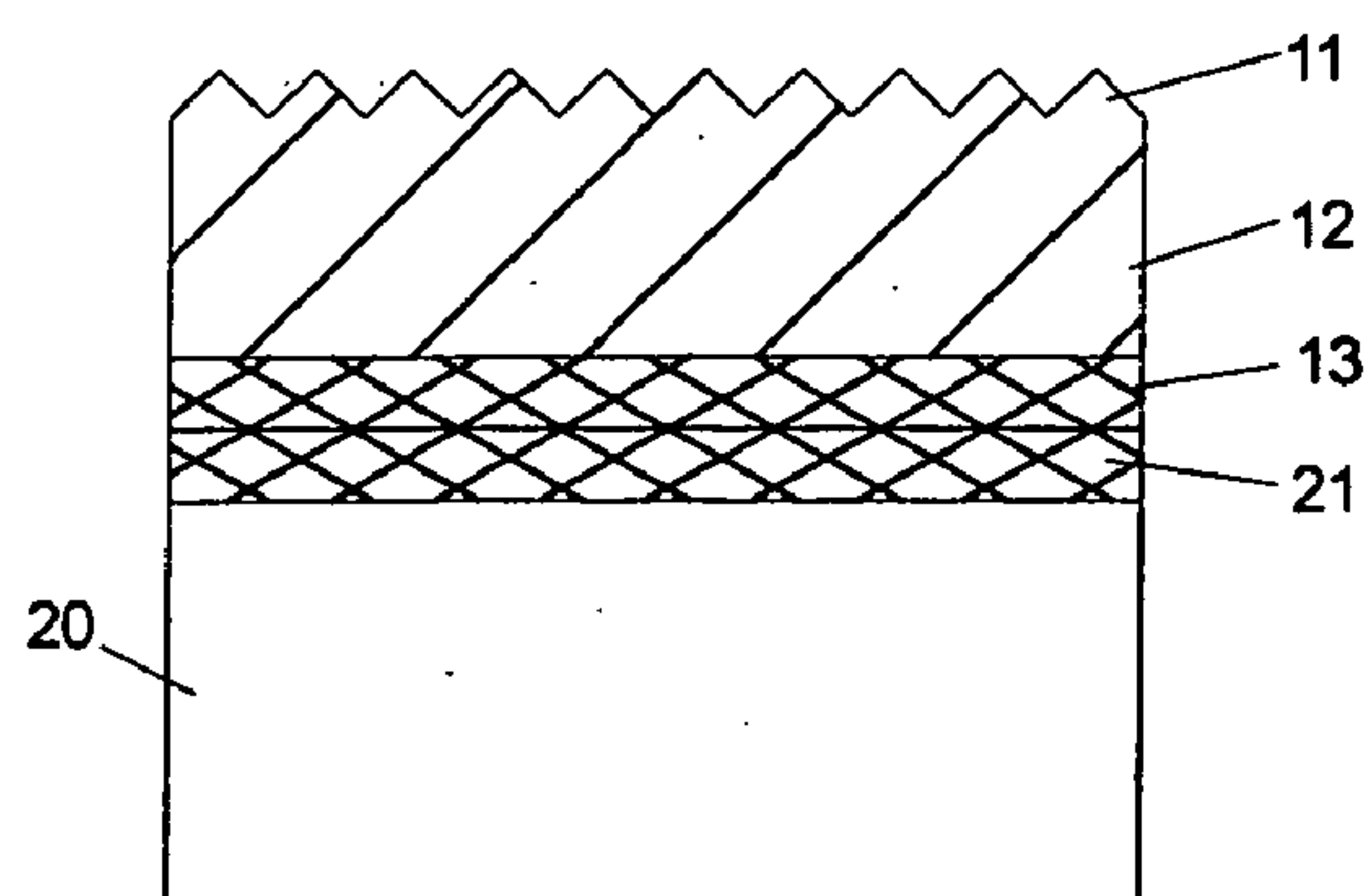
FIG. 2G: Exfoliate GaN Film
