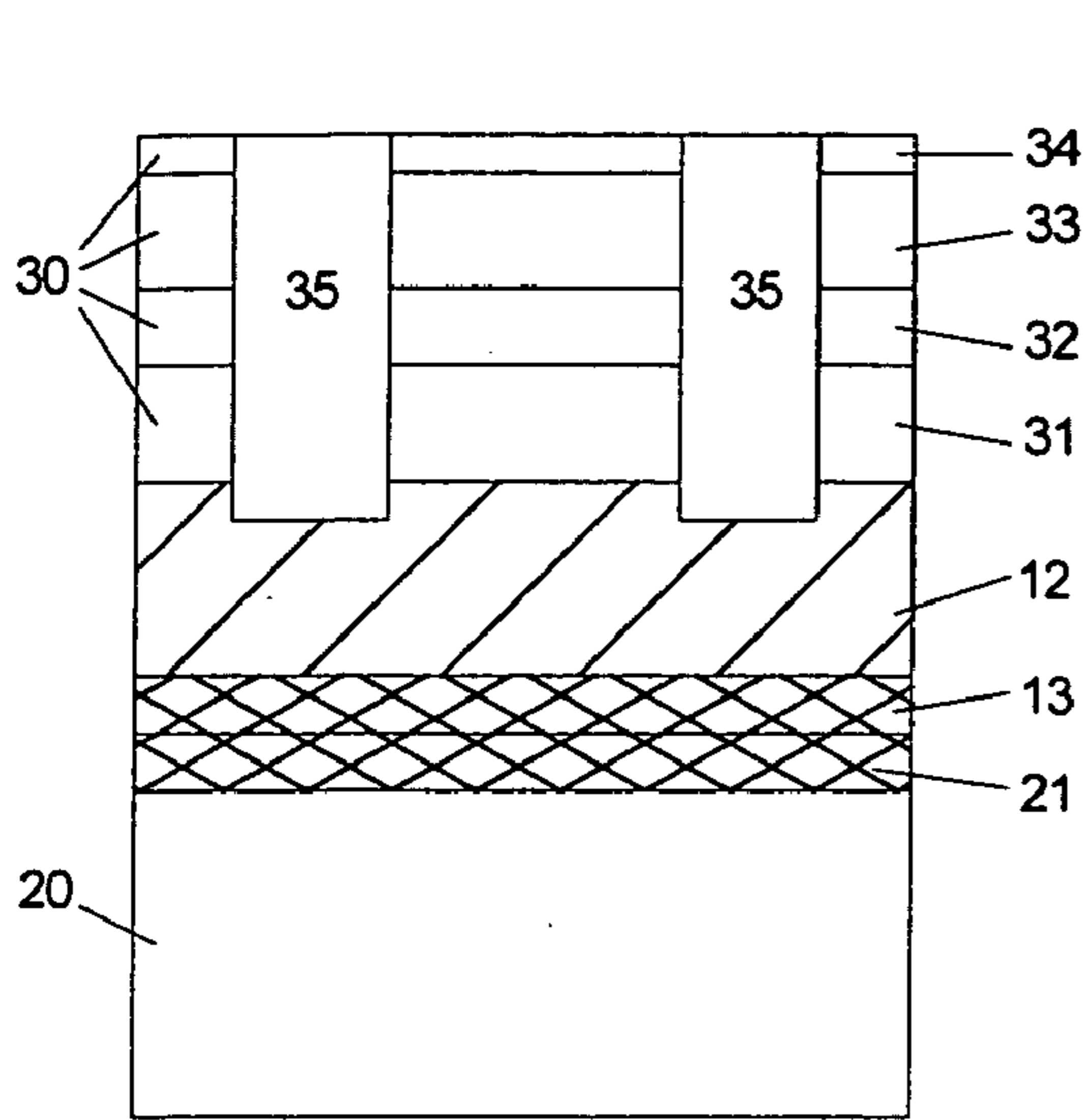
FIG. 5A: RIE Etch and Refill
