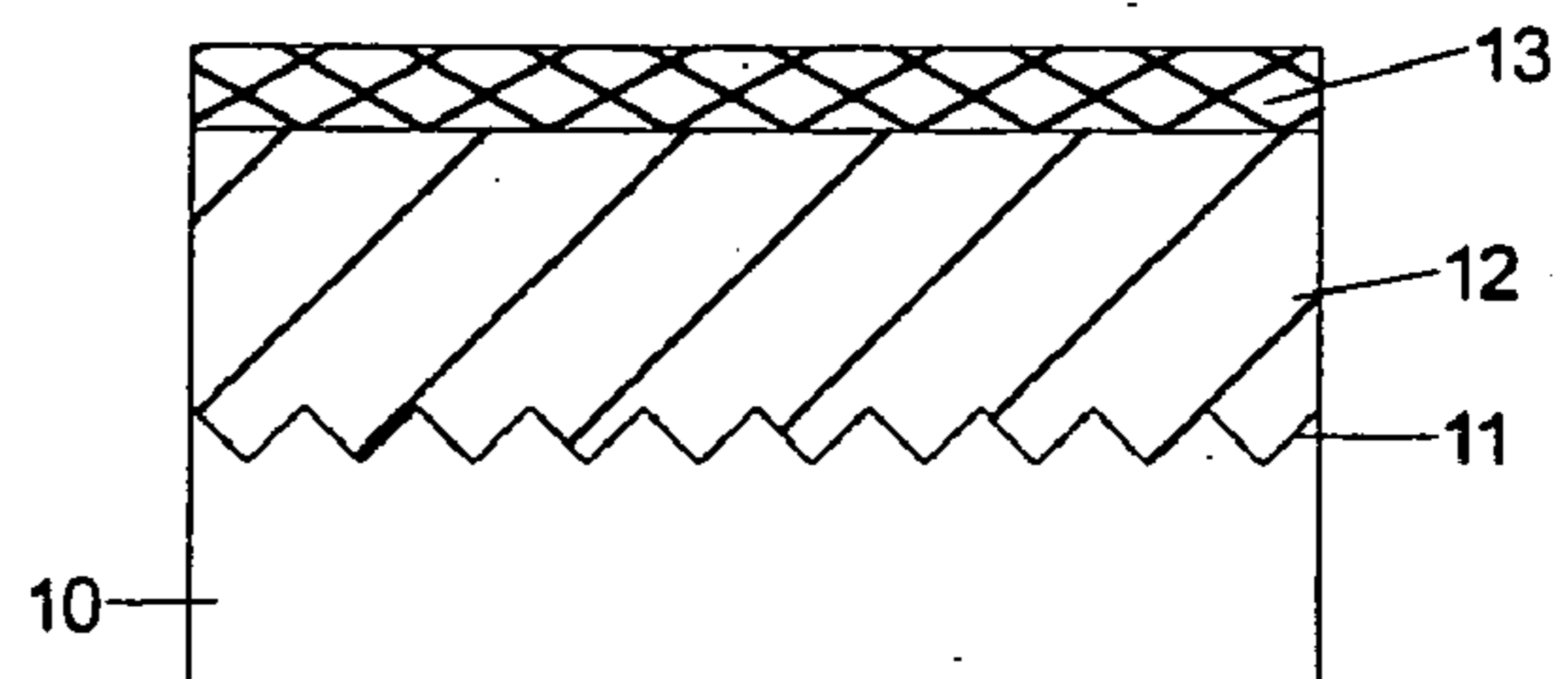
FIG. 2D: SiO 2 Deposition
