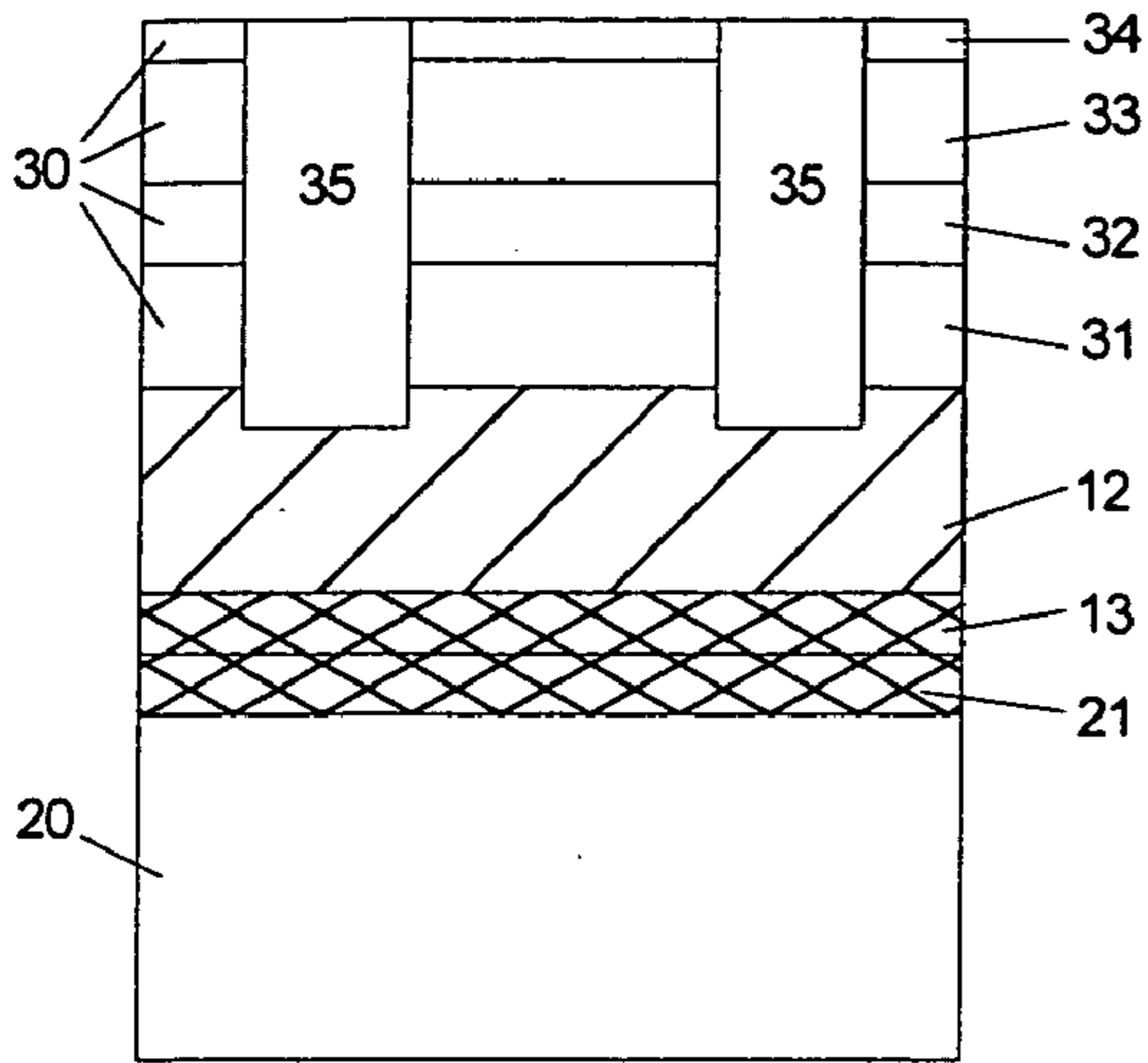
FIG. 5A: RIE Etch and Refill
