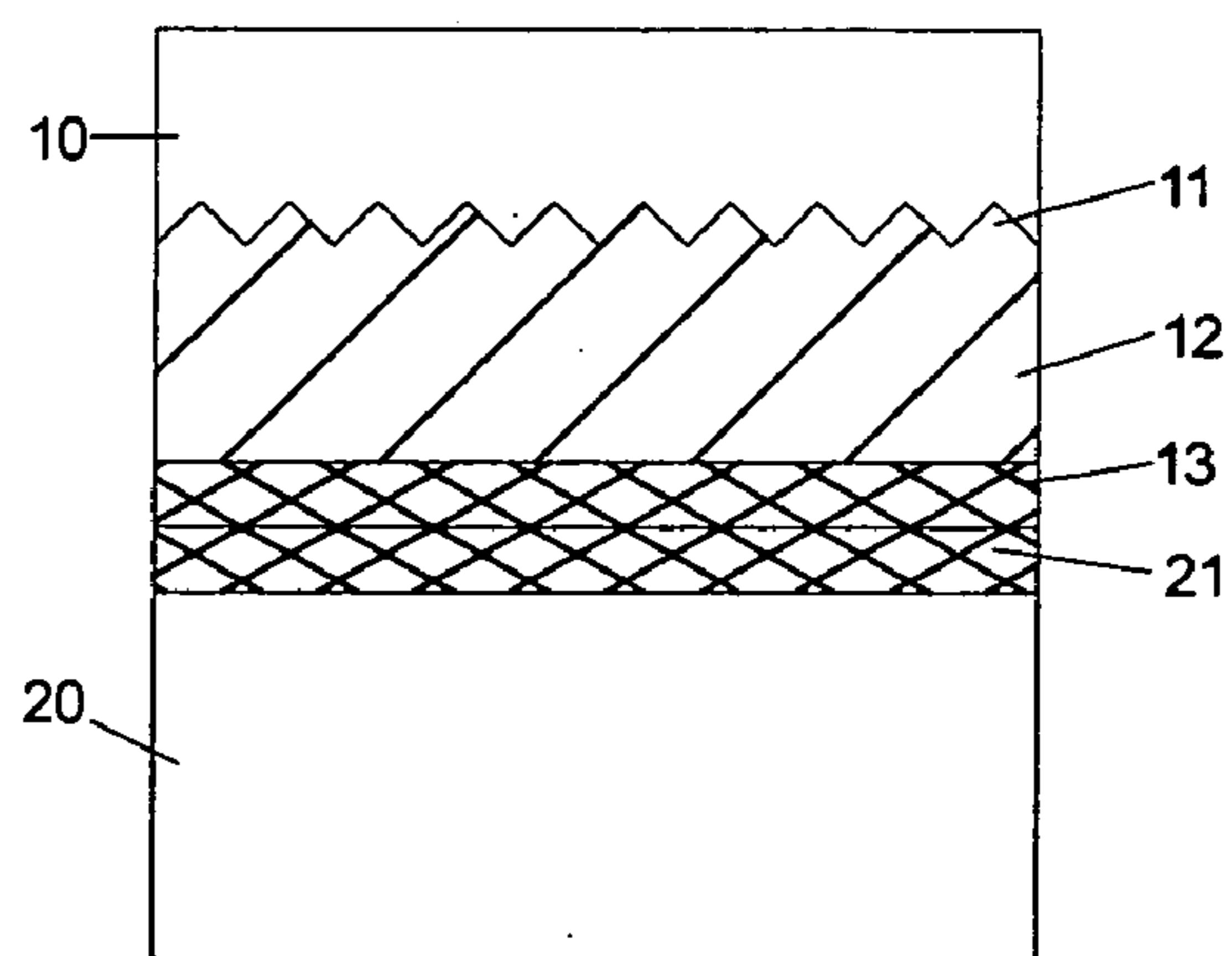
FIG. 2F: Bond Wafer
