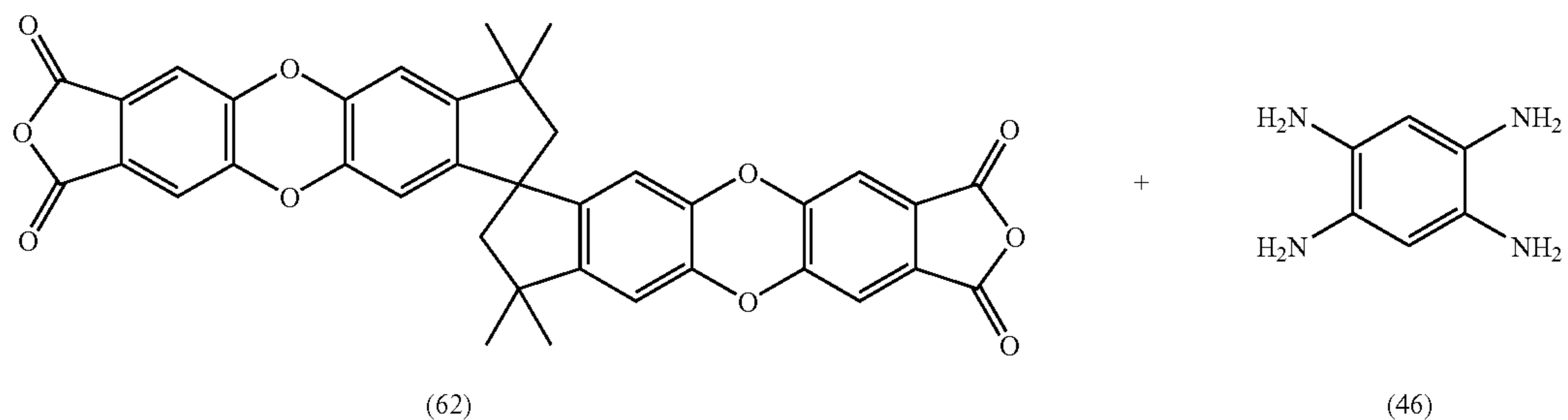
Reaction Scheme F
