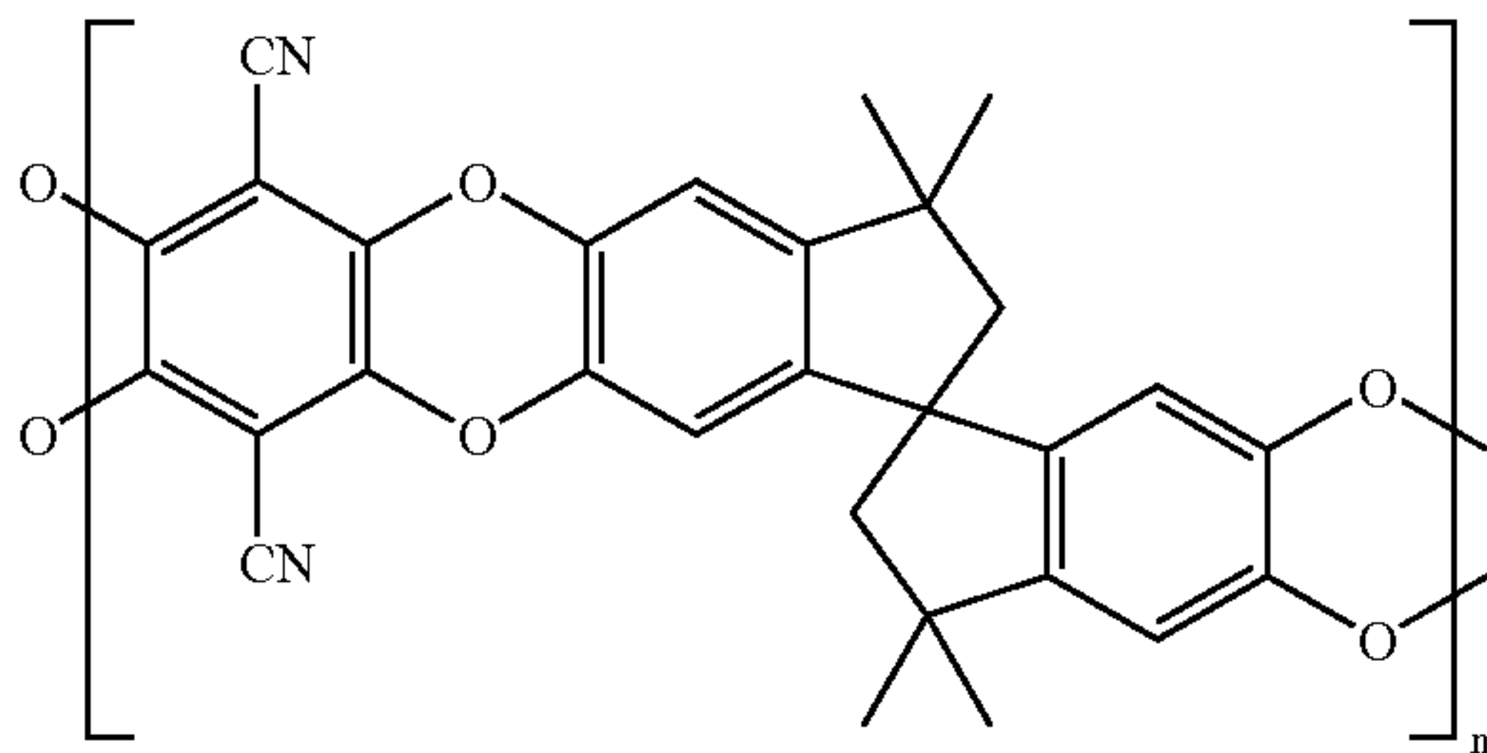
Polydioxane A (1)
