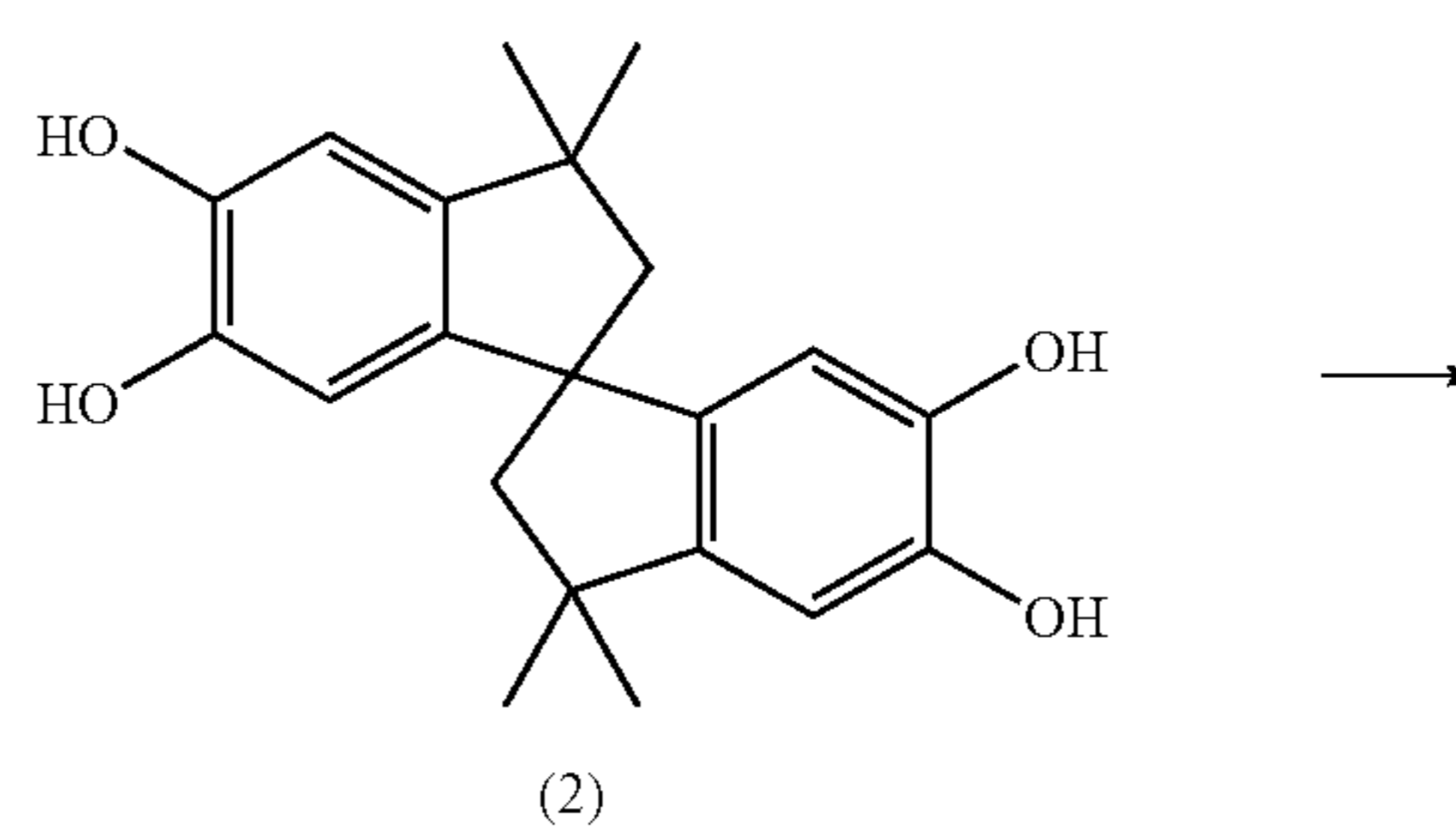
Reaction scheme G
