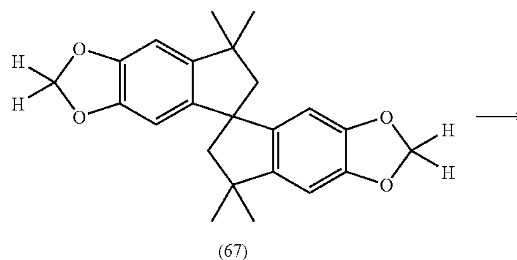
Reaction scheme H
