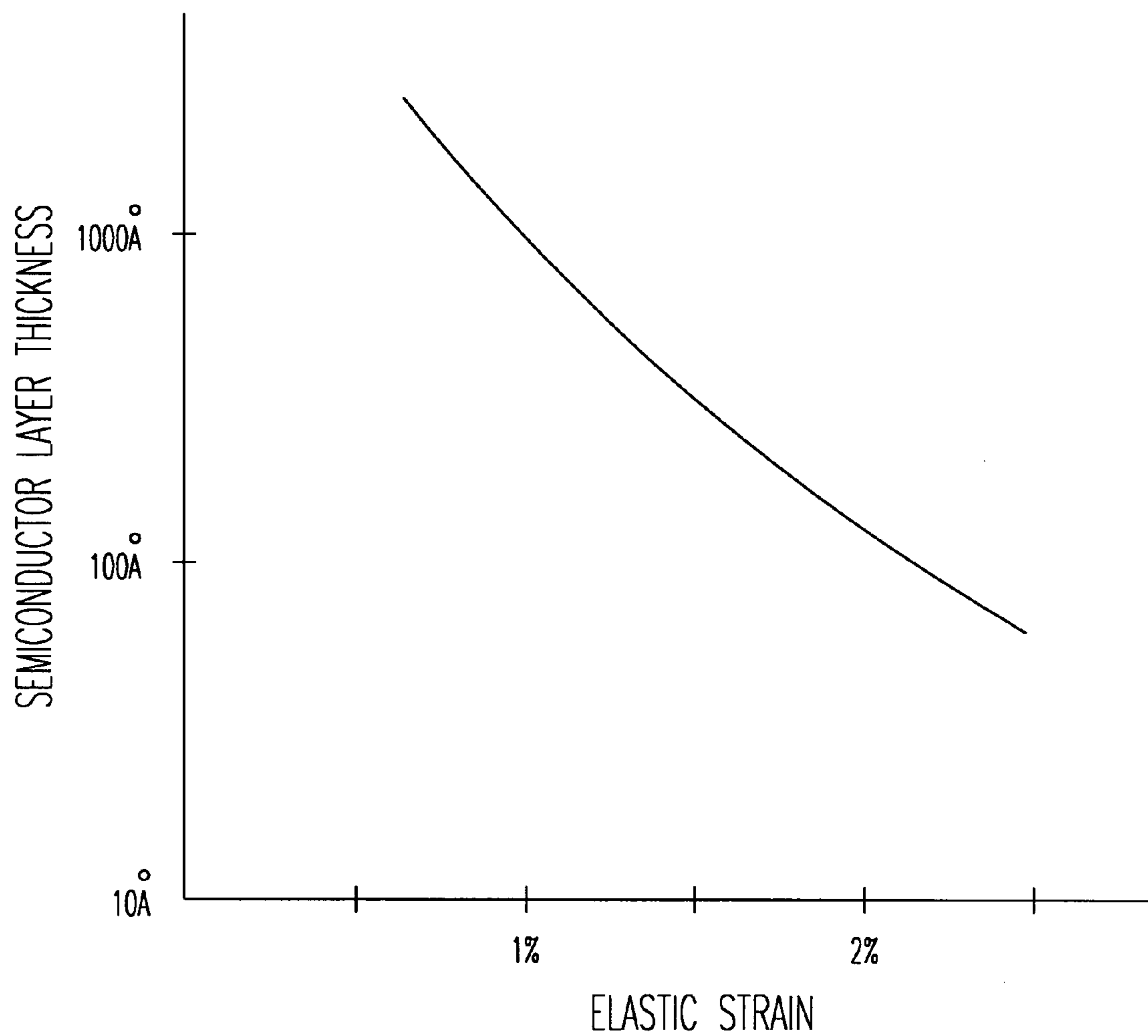
FIG. 3 (PRIOR ART)
