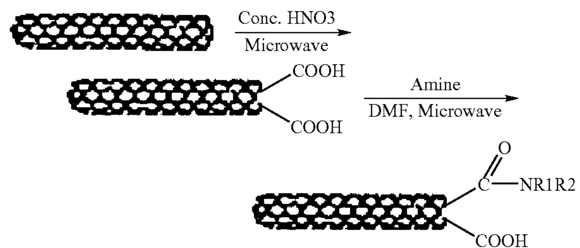
[0054] Scheme 1, amidation of SWNTs,
