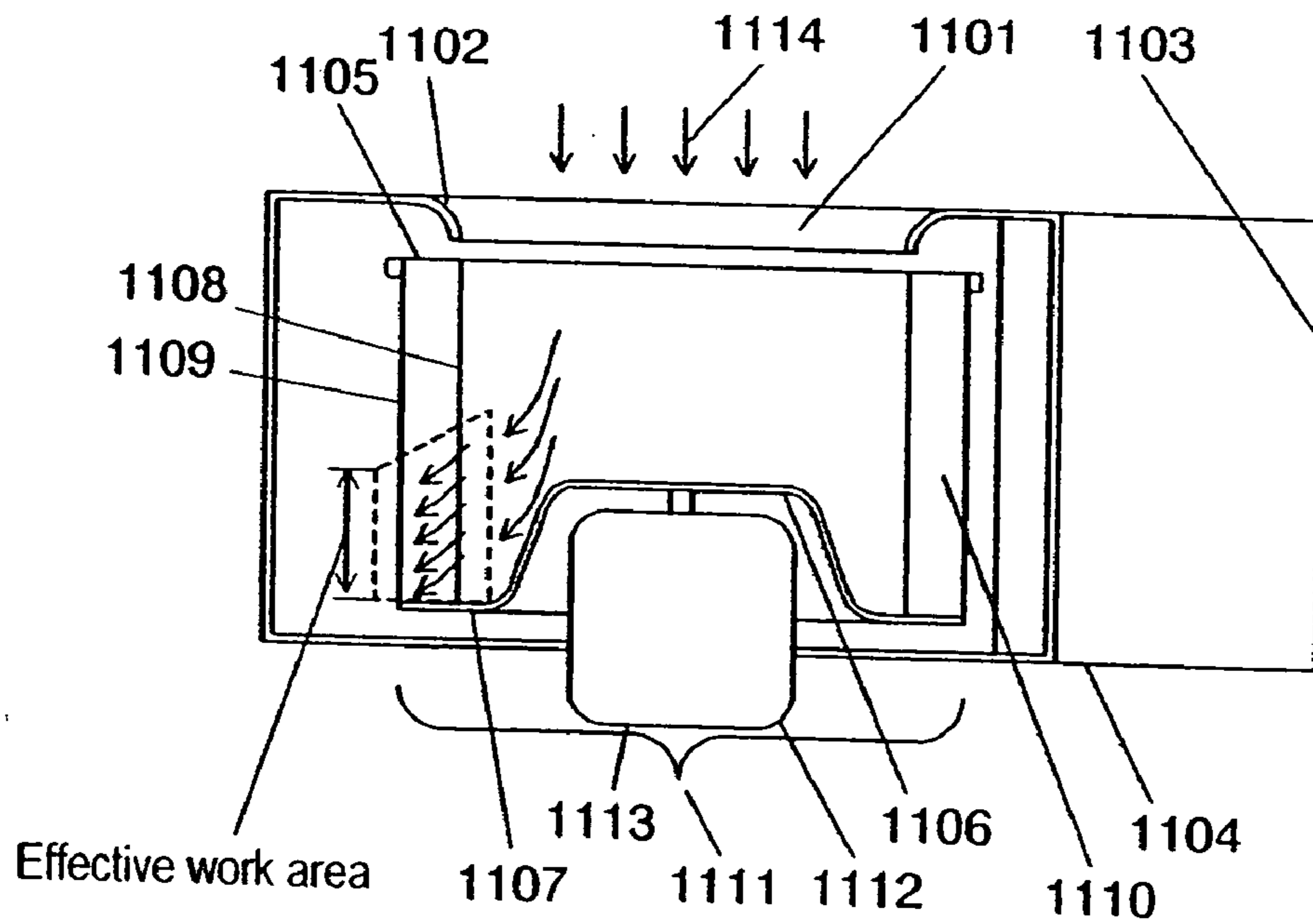
FIG. 17 PRIOR ART
