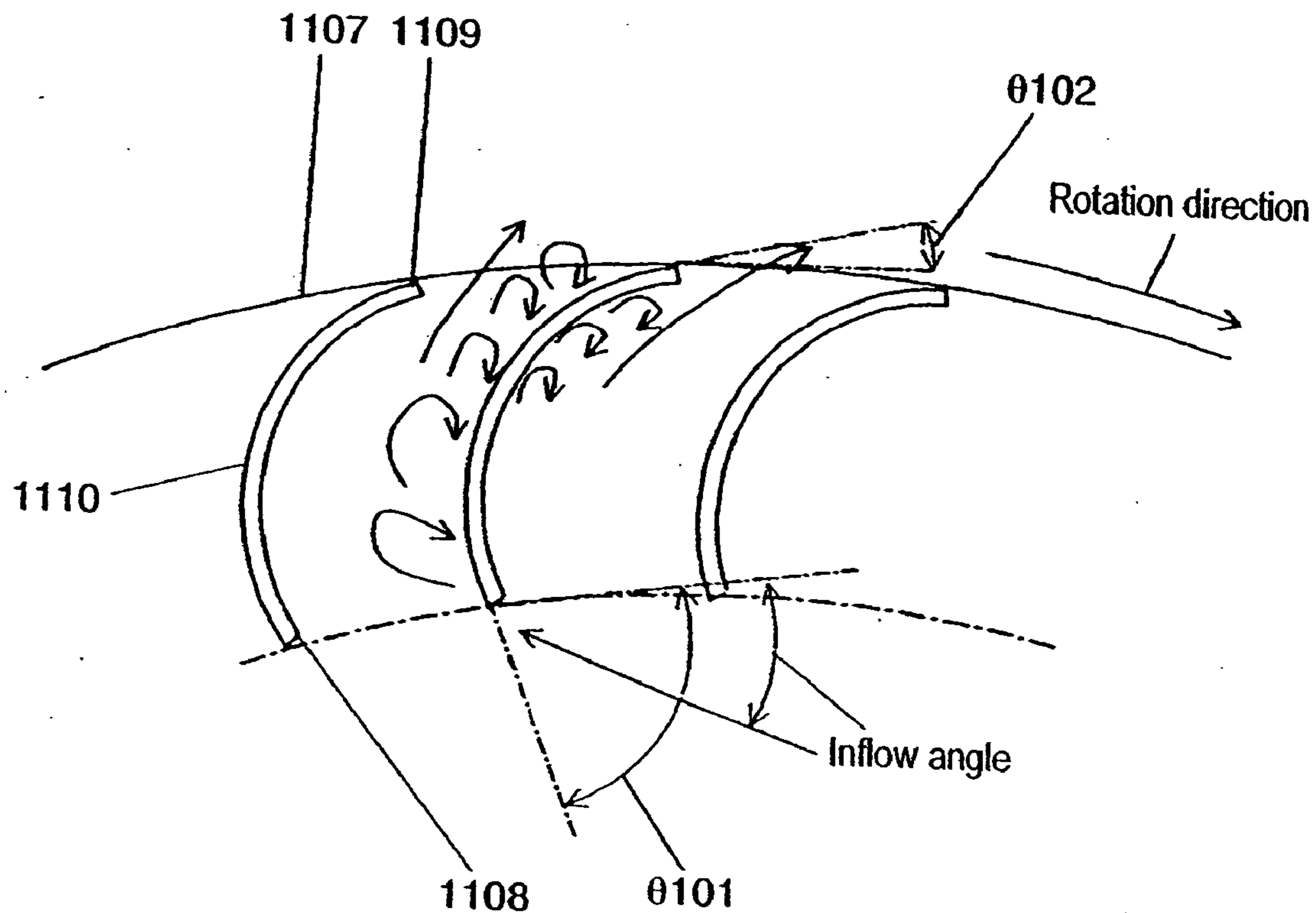
FIG. 18 PRIOR ART
