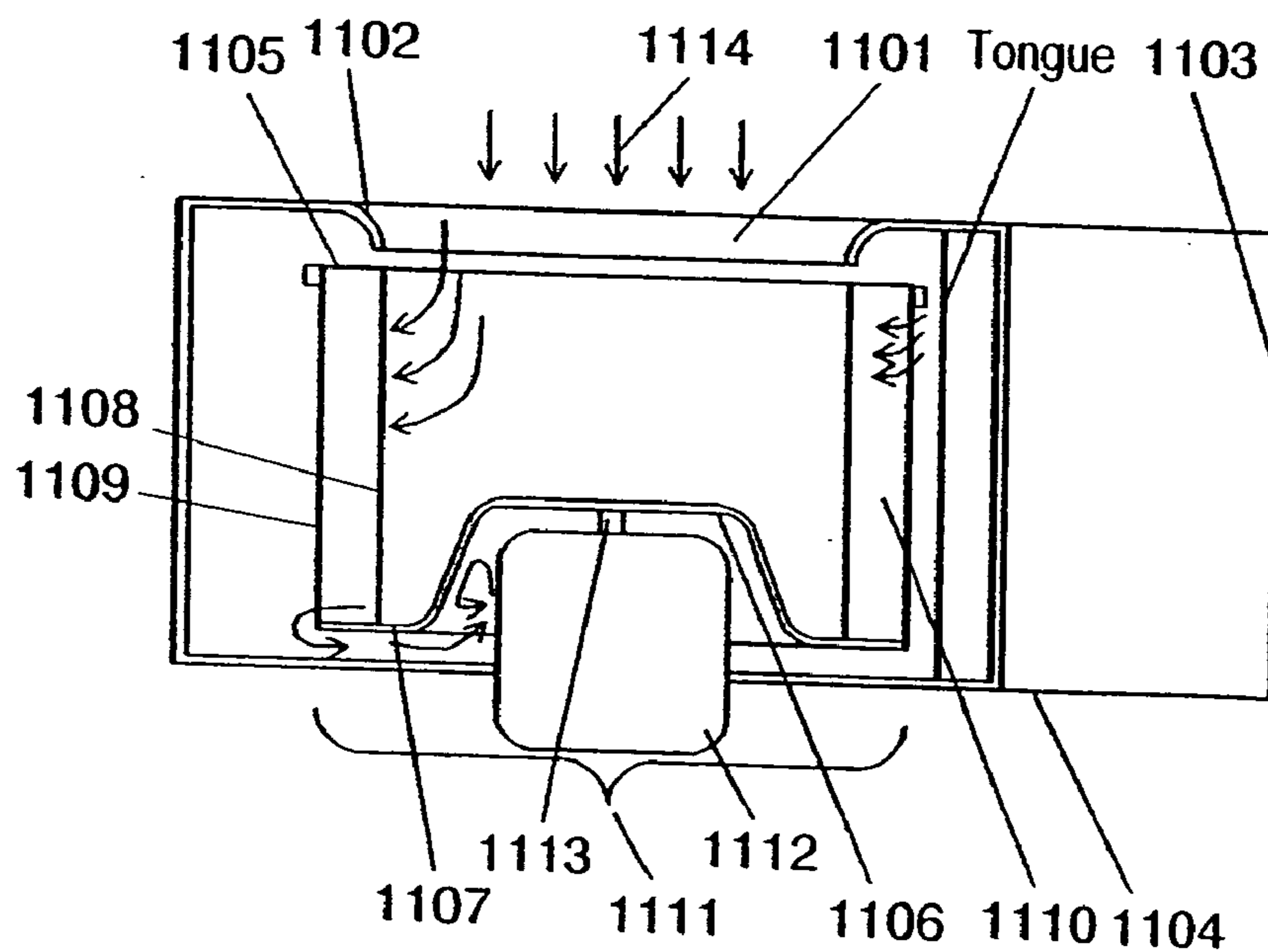
FIG. 19 PRIOR ART
