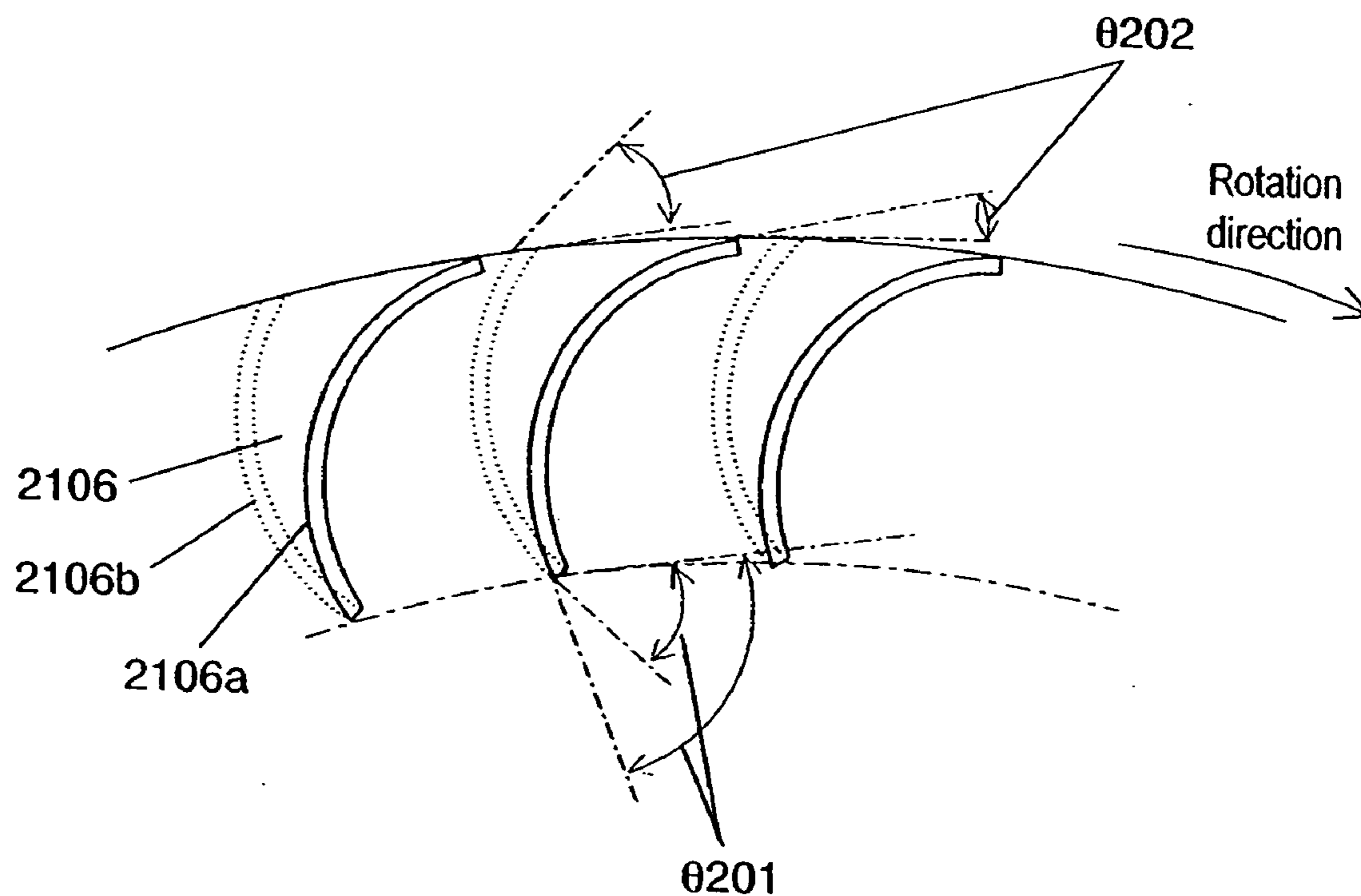
FIG. 31 PRIOR ART
