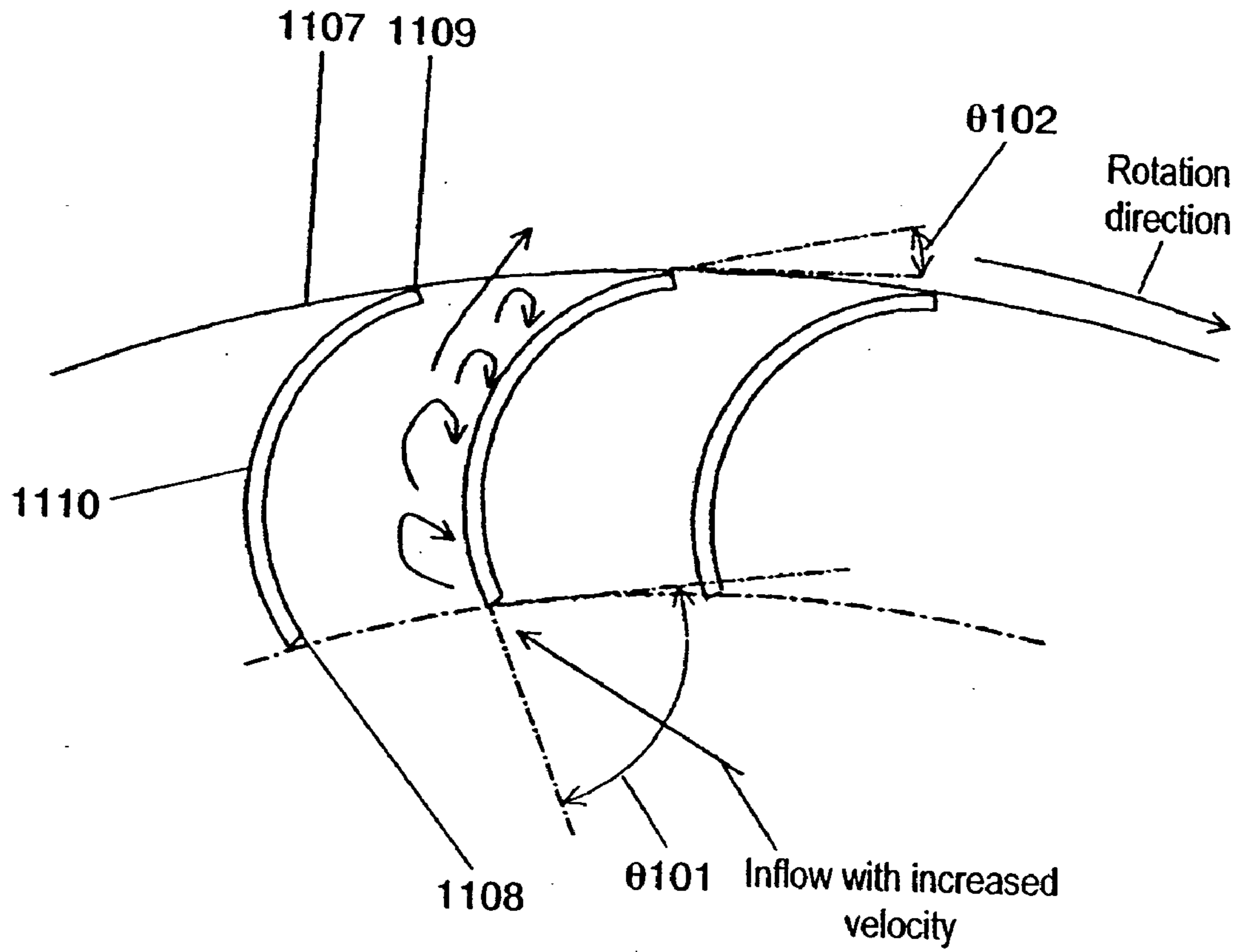
FIG. 16 PRIOR ART
