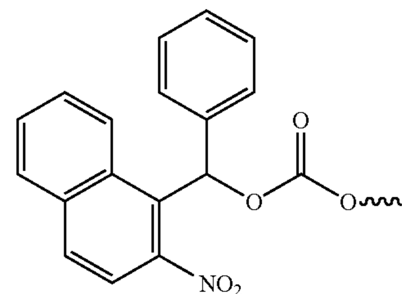
(2-nitro-naphthalen-1-yl)- phenylmethoxycarbonyl (NNPOC)
