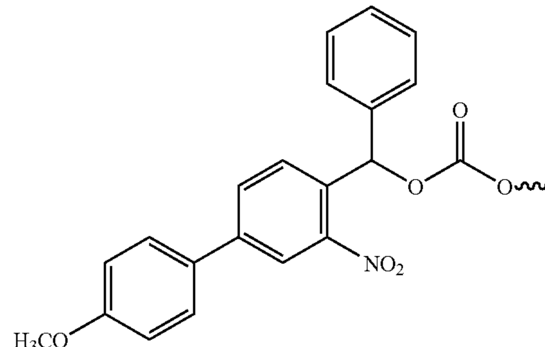
(4'-methoxy-3-nitro-biphenyl-4-yl)- phenylmethoxycarbonyl (MBPMOC)
