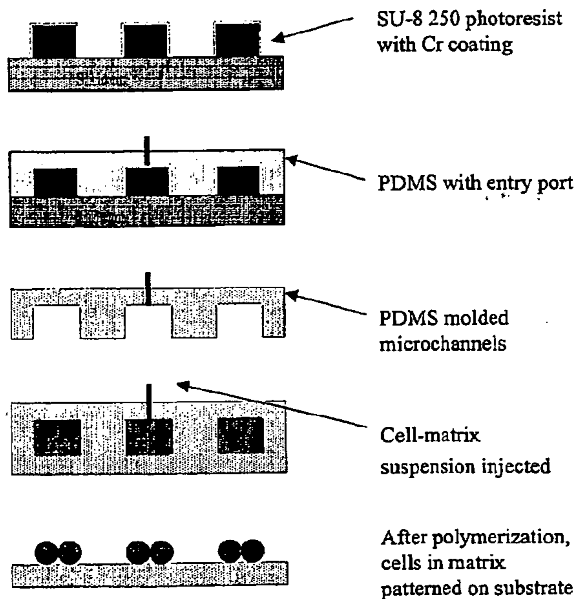
Fig 2. Flow chart of preparing cell patterns on the substrate using microfabrication and microfluidic techniques
