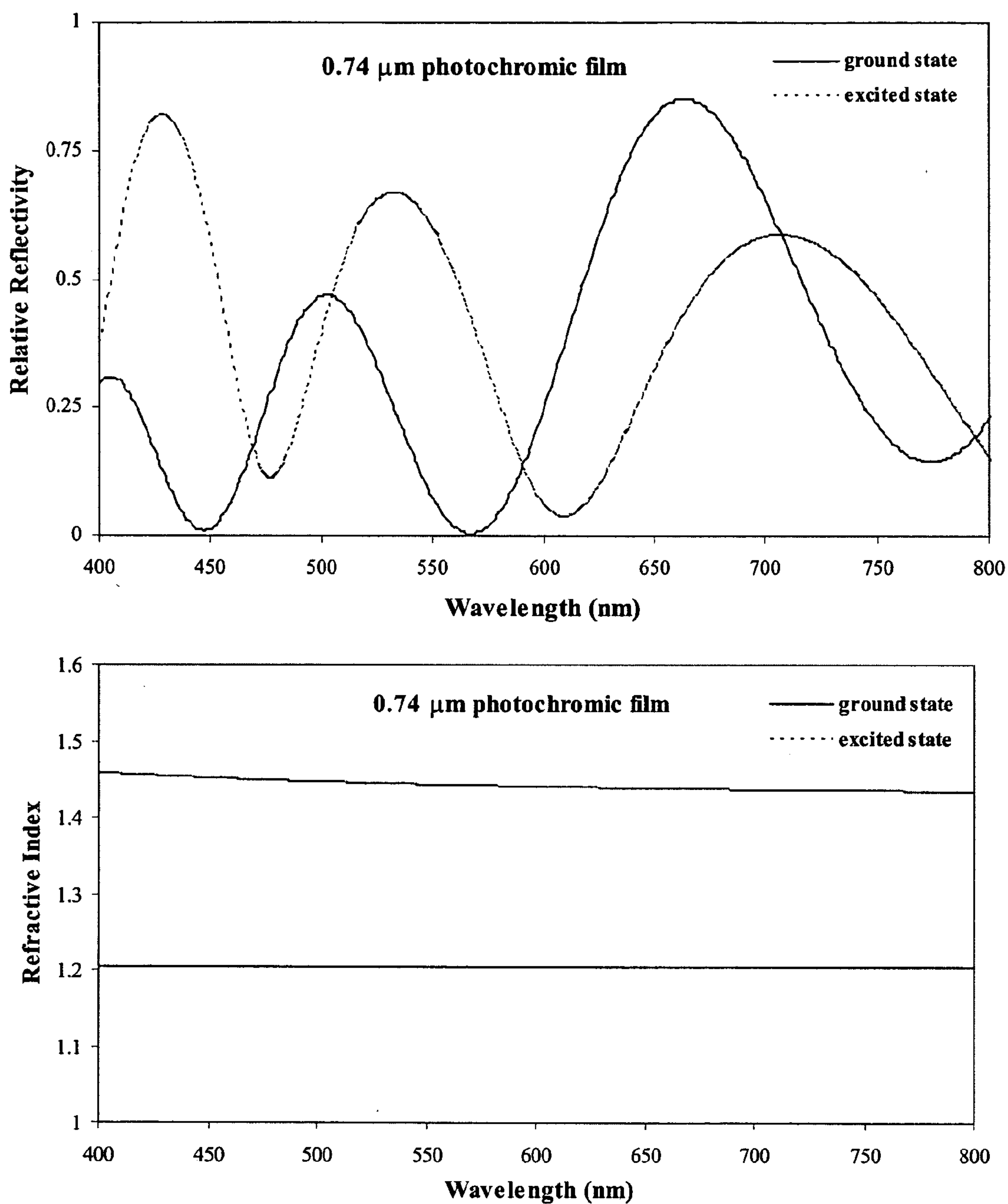
Figure 56. Examples of the observed reflectance spectra and the calculated refractive indices for the mesostructured silica/ \text{EO}_{106}\text{PO}_{70}\text{EO}_{106} optical film containing the spiropyran dye in the ground state (blue, solid trace) and the excited state (red, dashed trace).
