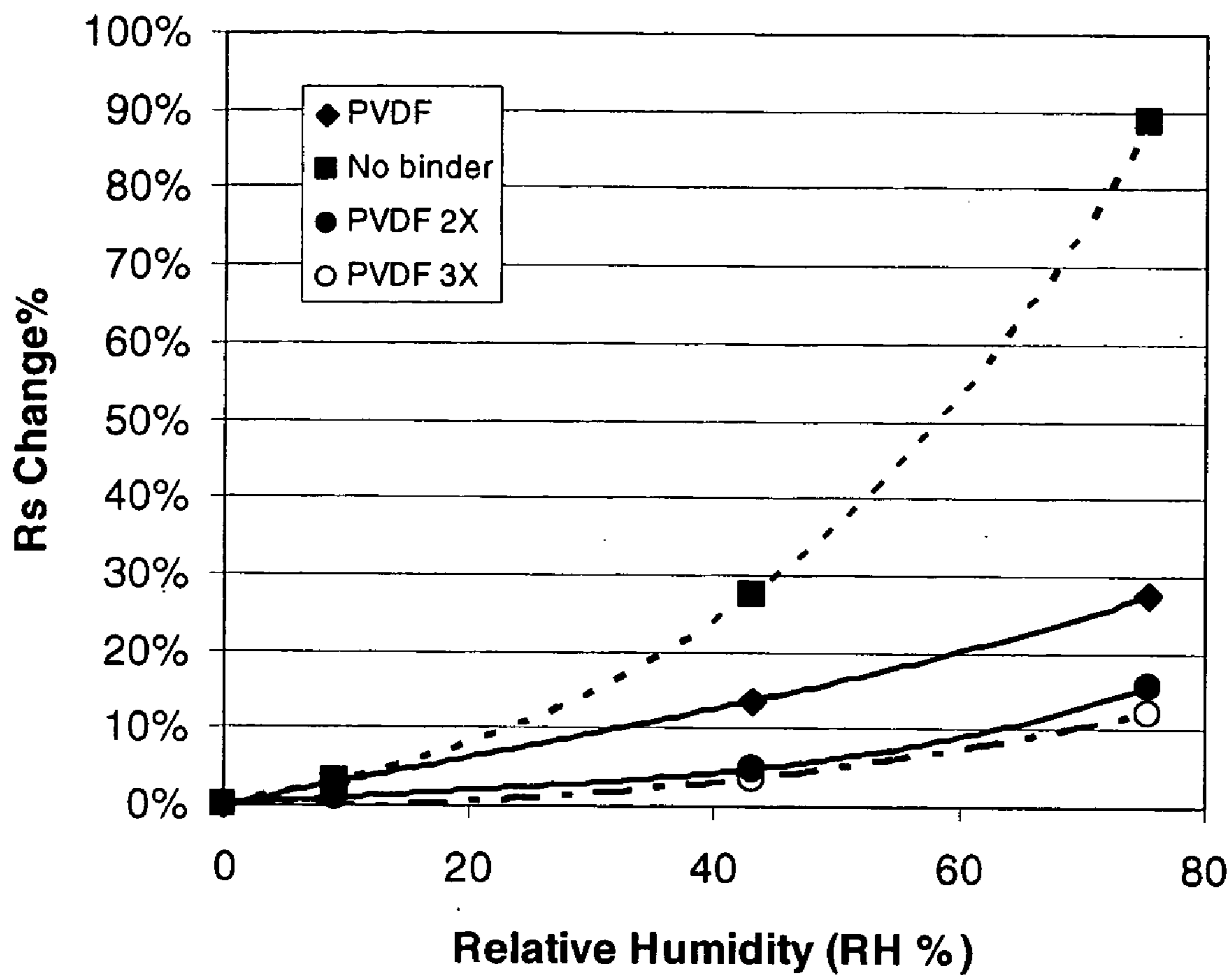
Moisture Effect (Using PVDF vs Bare CNT)
