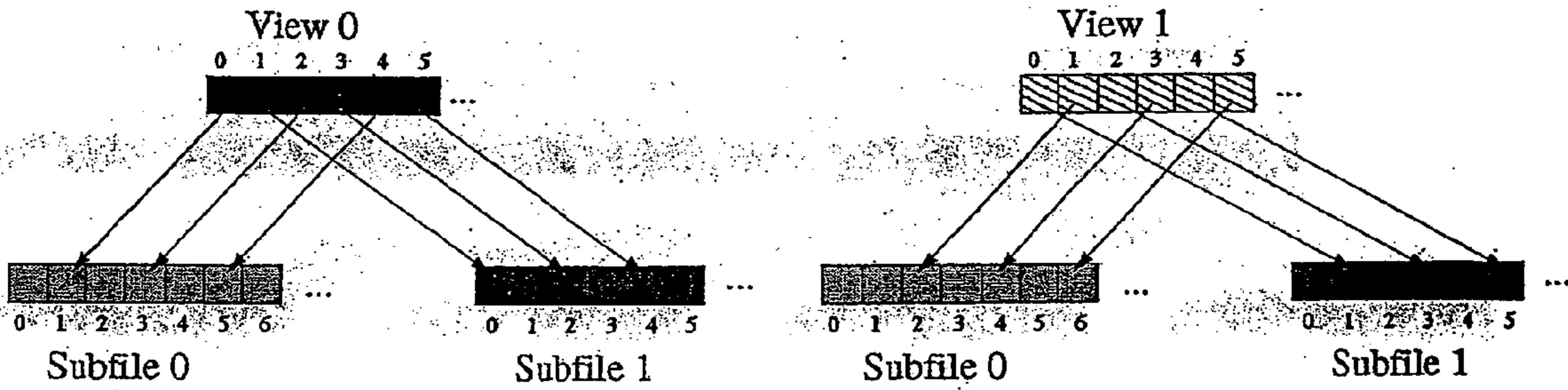
(c) Direct mapping between logical and physical partitioning
