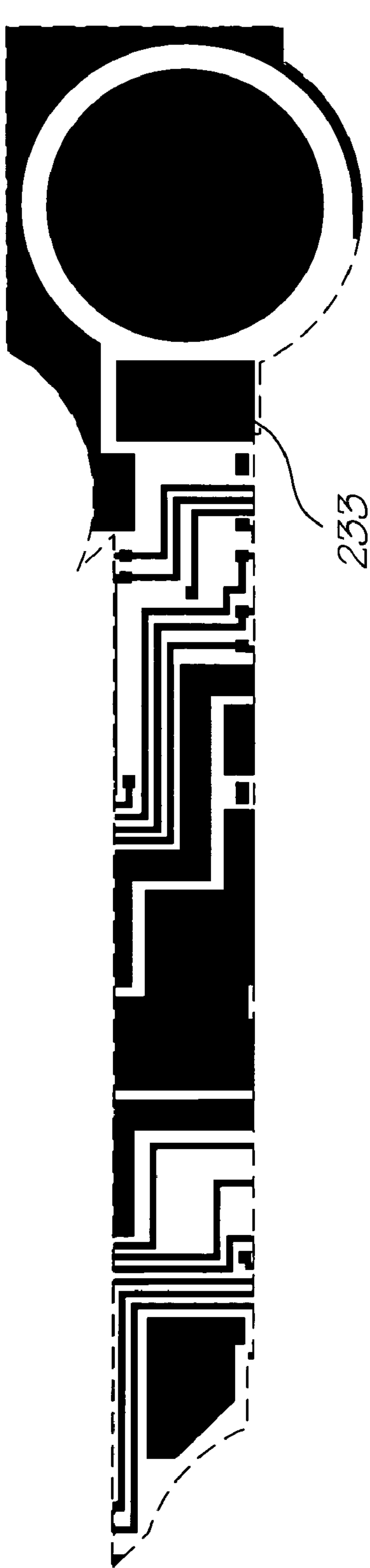
Metal 2 mask
