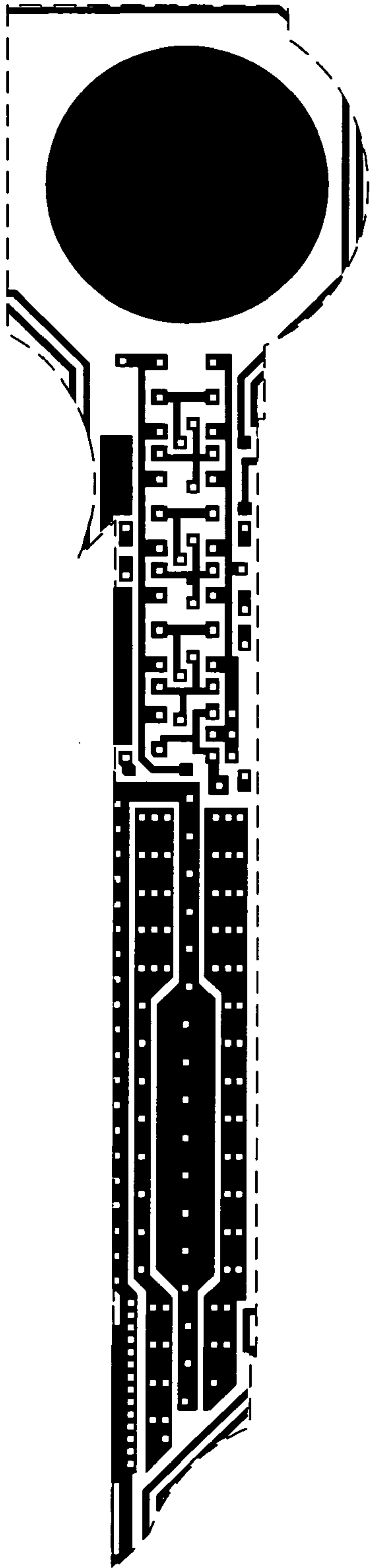
Metal 1 mask
