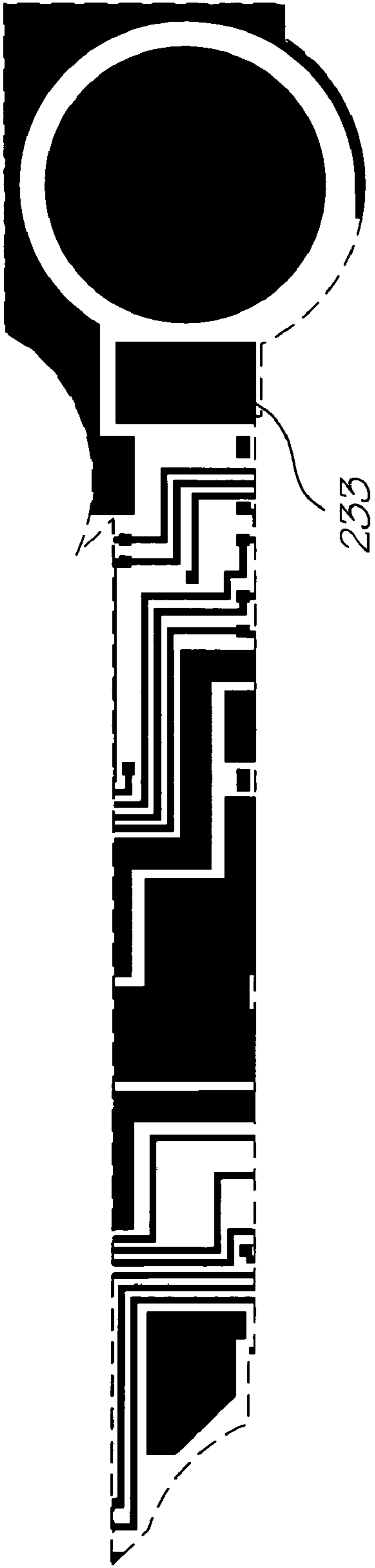
Metal 2 mask
