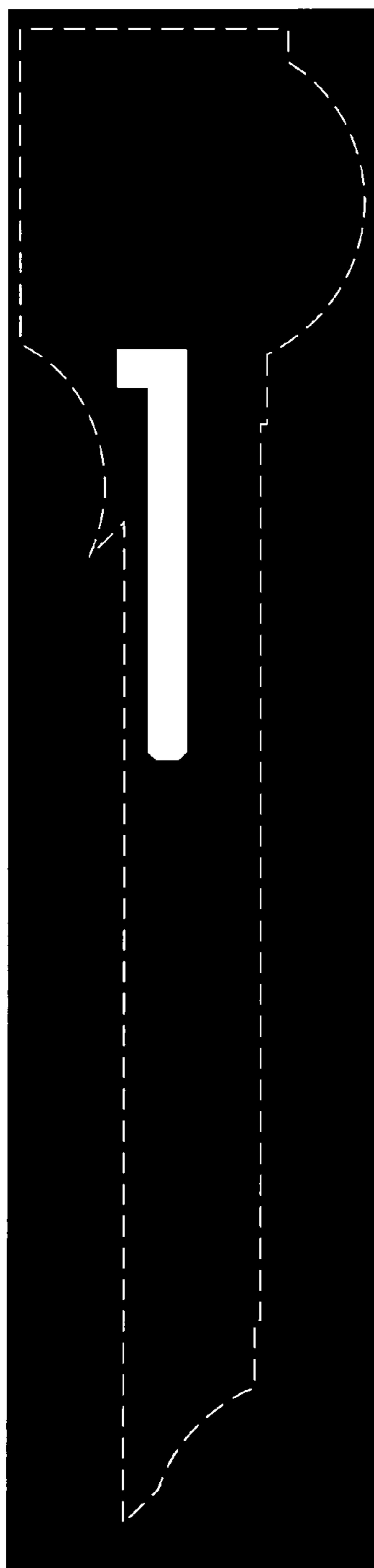
N-Well mask
