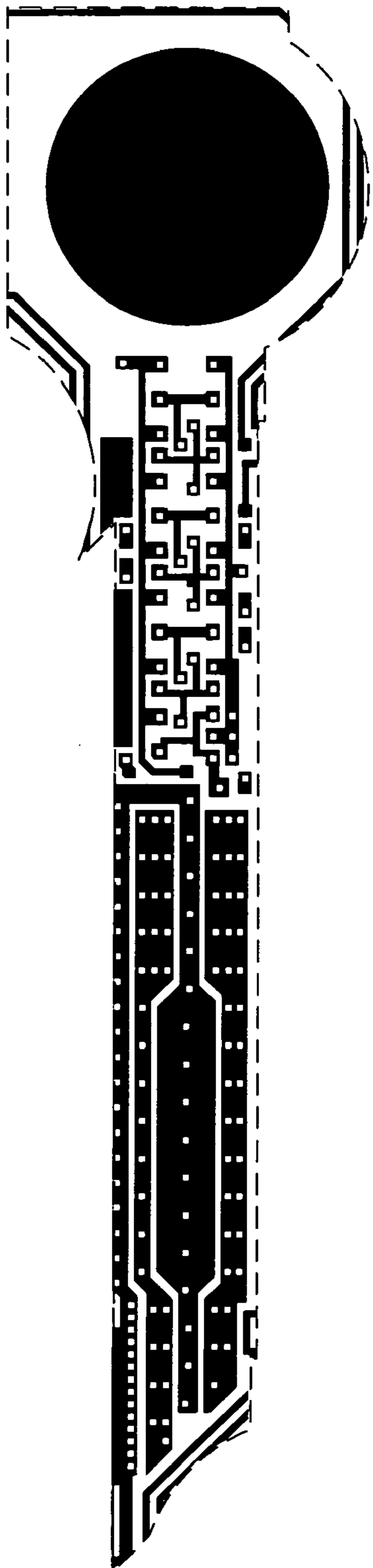
Metal 1 mask
