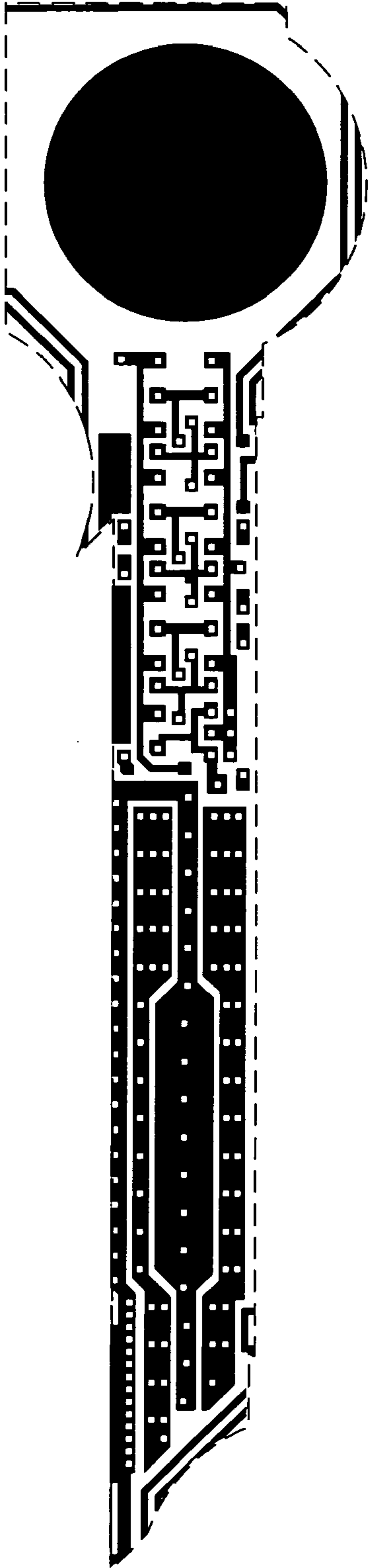
Metal 1 mask
