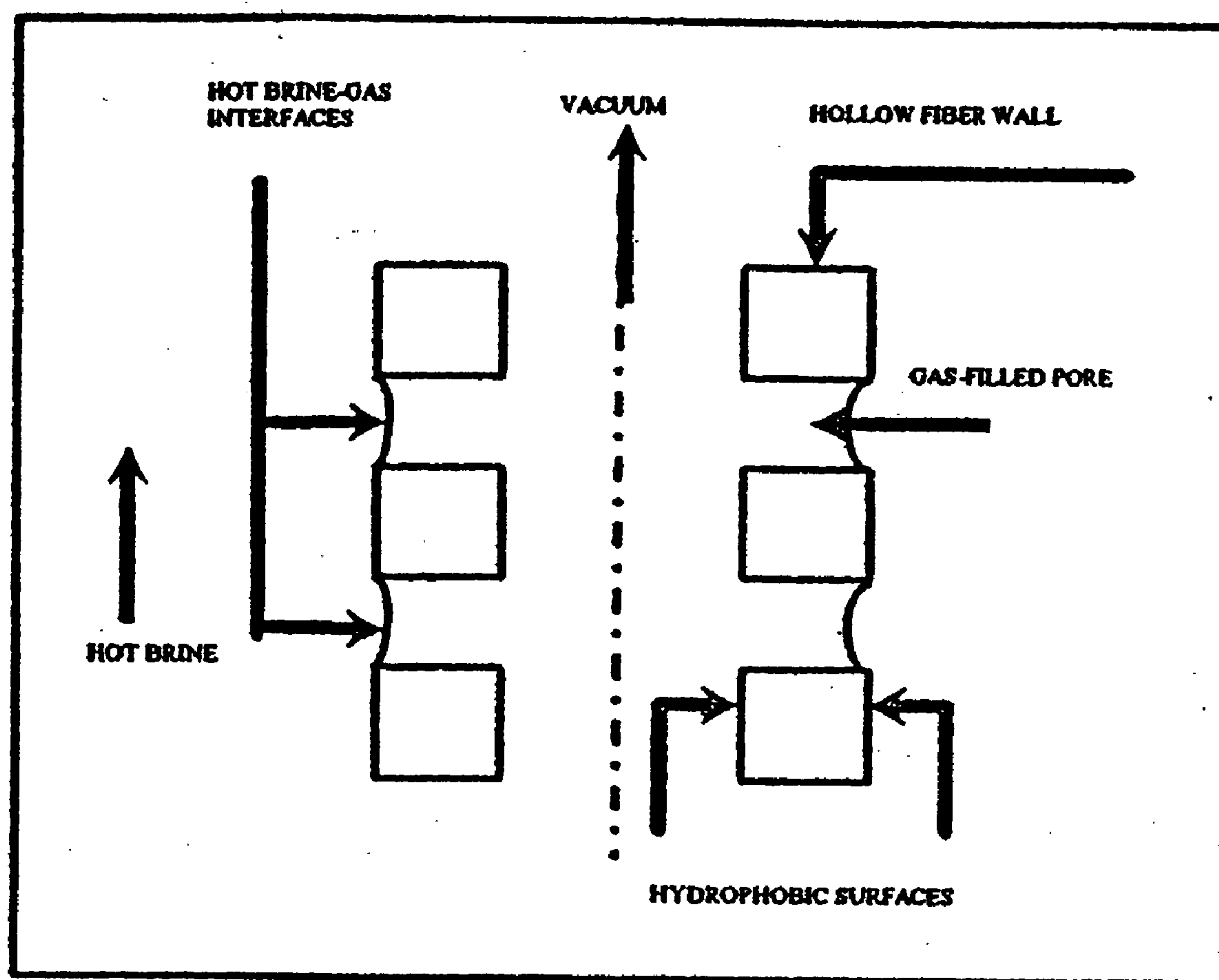
Fig. 1b. Conventional Vacuum Membrane distillation
