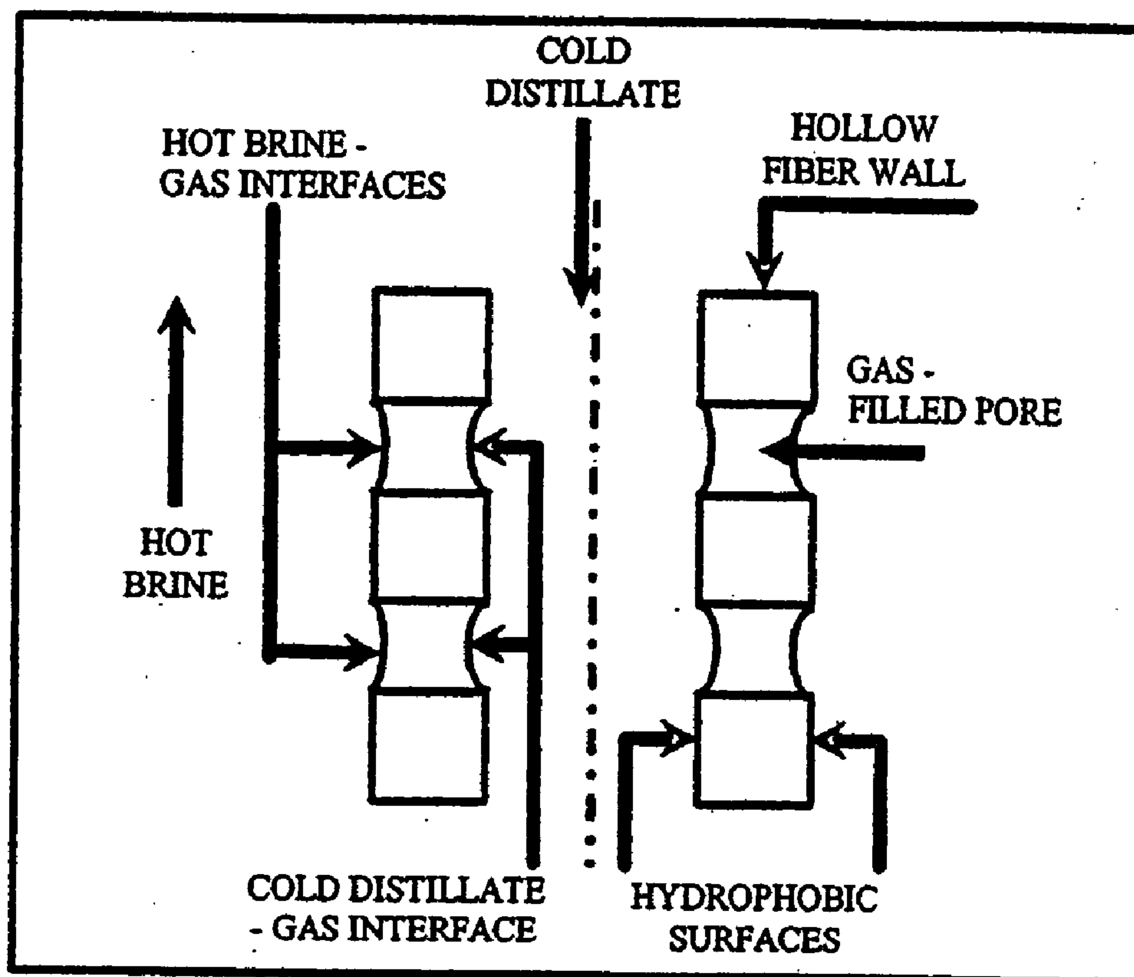
Conventional direct contact membrane distillation
