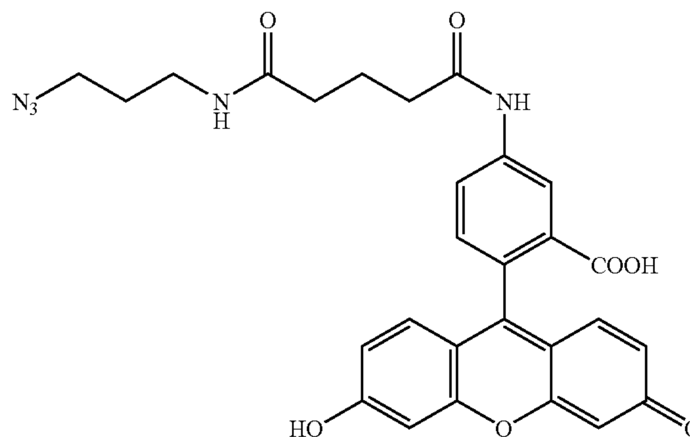
Azido Dye 3 (Compound 3)
