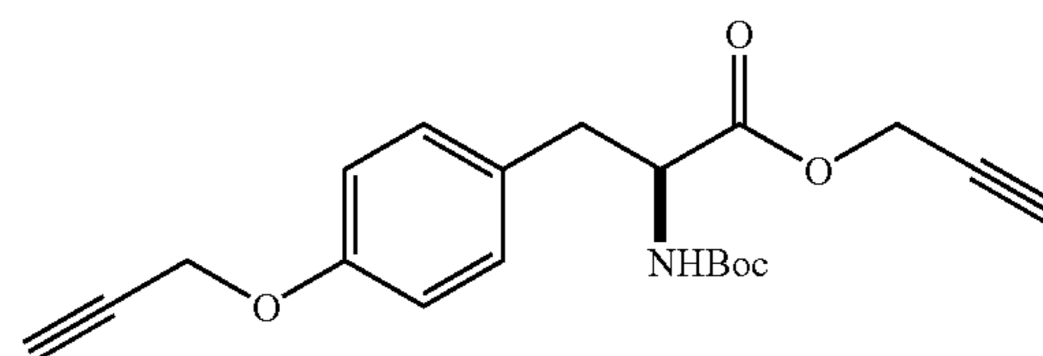
2-tert-butoxycarbonylamino-3-[4-(prop-2-ynyloxy)phenyl]-propionic acid propargyl ester (Compound 4)
