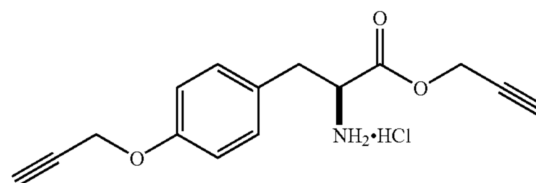
2-amino-3-[4-(prop-2-ynyloxy)phenyl]-propionic acid propargyl ester (Compound 5)
