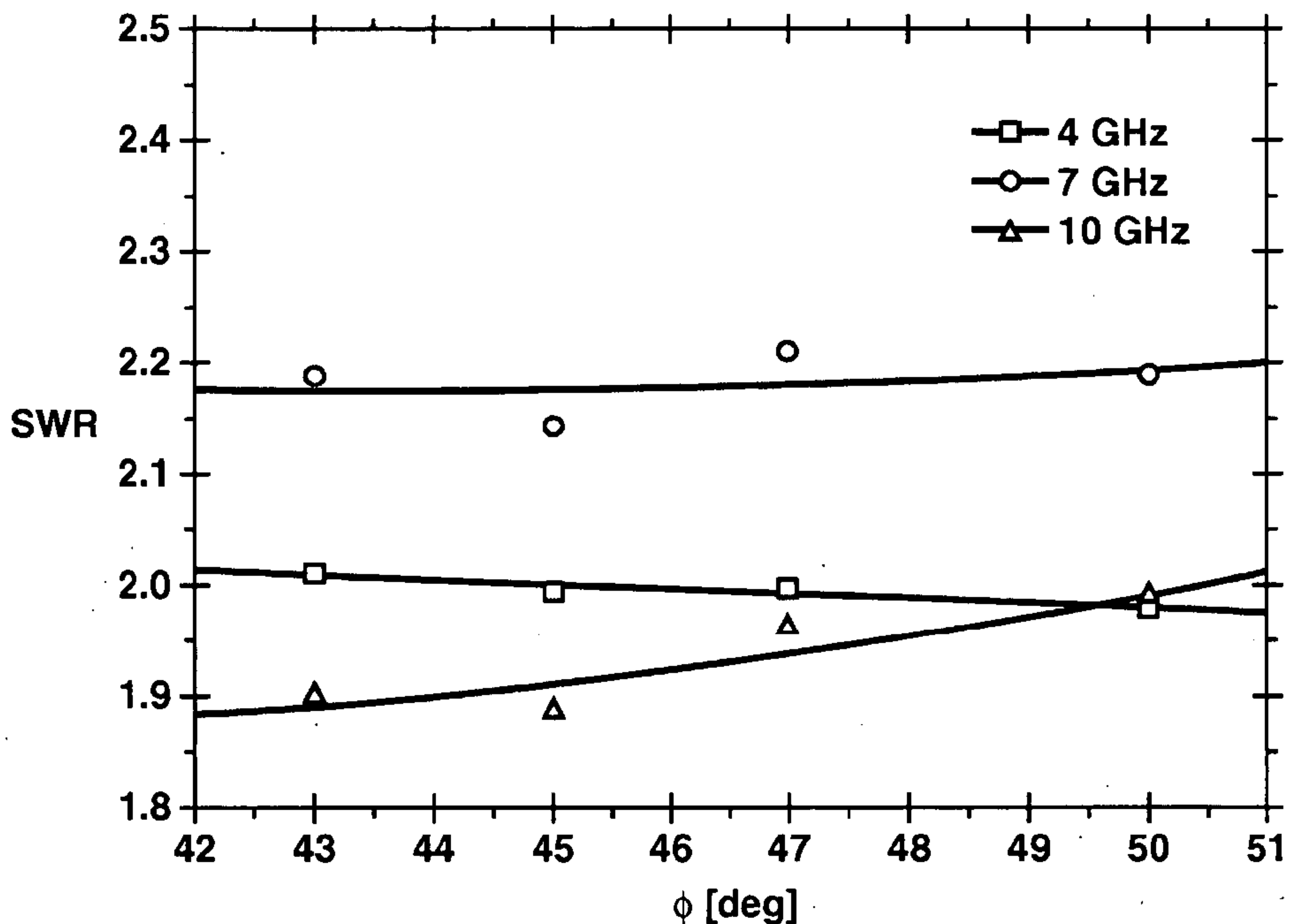
RELATIONSHIP BETWEEN SWR AND ANGLE \phi OF TAPER REGION (H: 25.0 mm \theta : 90° a: 14.4 mm W: 2.0 mm G: 0.6 mm d: 0.5 mm L: 1.0 mm)
