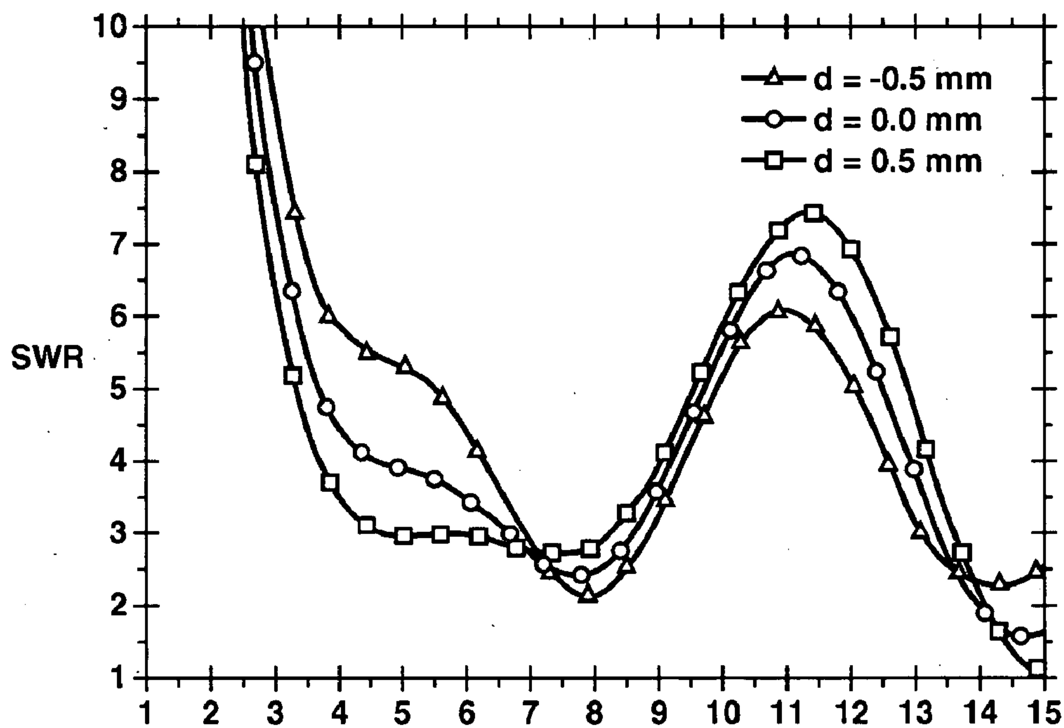
FREQUENCY [GHz] DEPENDENCY ON DISTANCE d BETWEEN ANTENNA AND GROUND (H: 6.0 mm \theta : 90° a: 8.4 mm W: 2.0 mm G: 0.6 mm \phi : — L: —)
