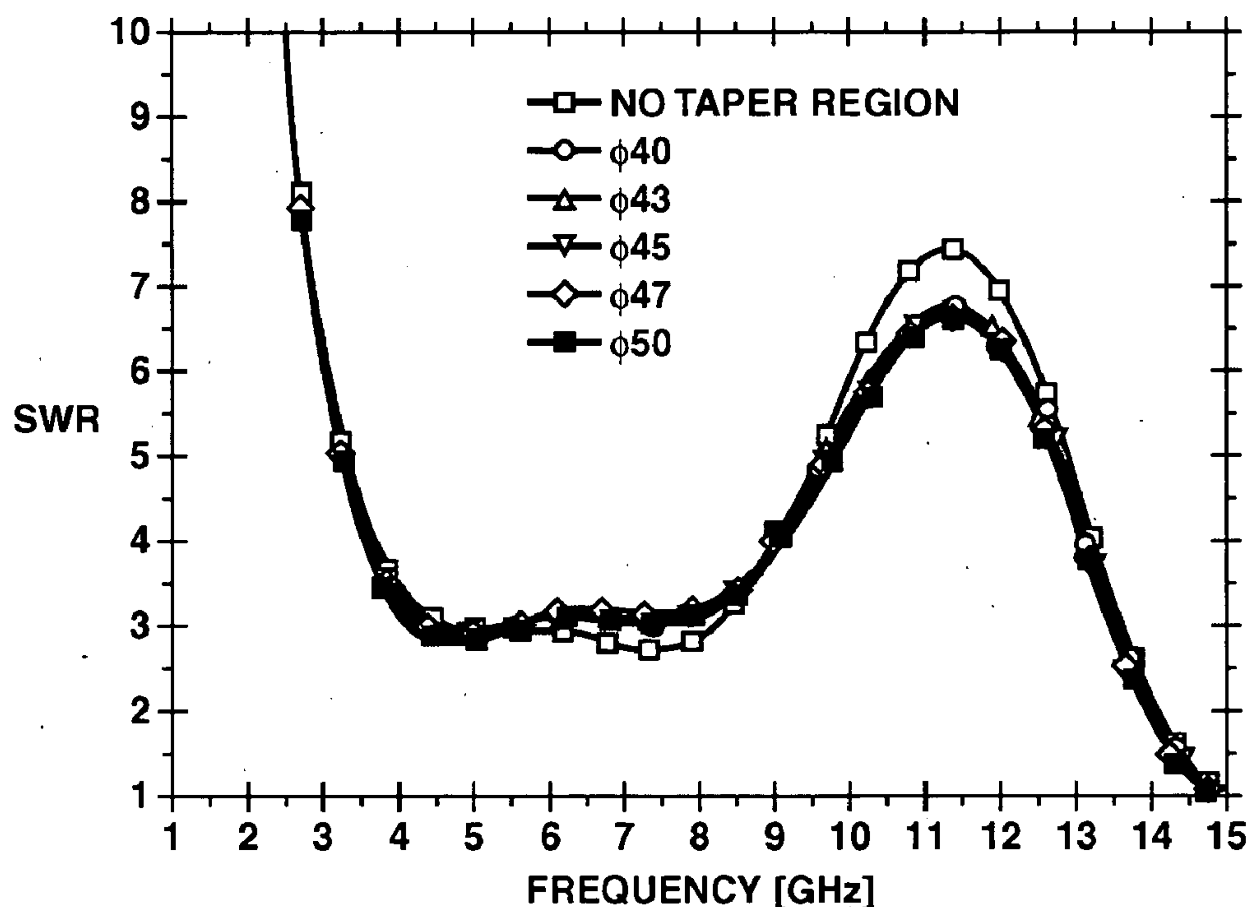
DEPENDENCY ON ANGLE \phi OF TAPER REGION (H: 6.0 mm \theta : 90° a: 8.4 mm W: 2.0 mm G: 0.6 mm d: 0.5 mm L: 0.7 mm)
