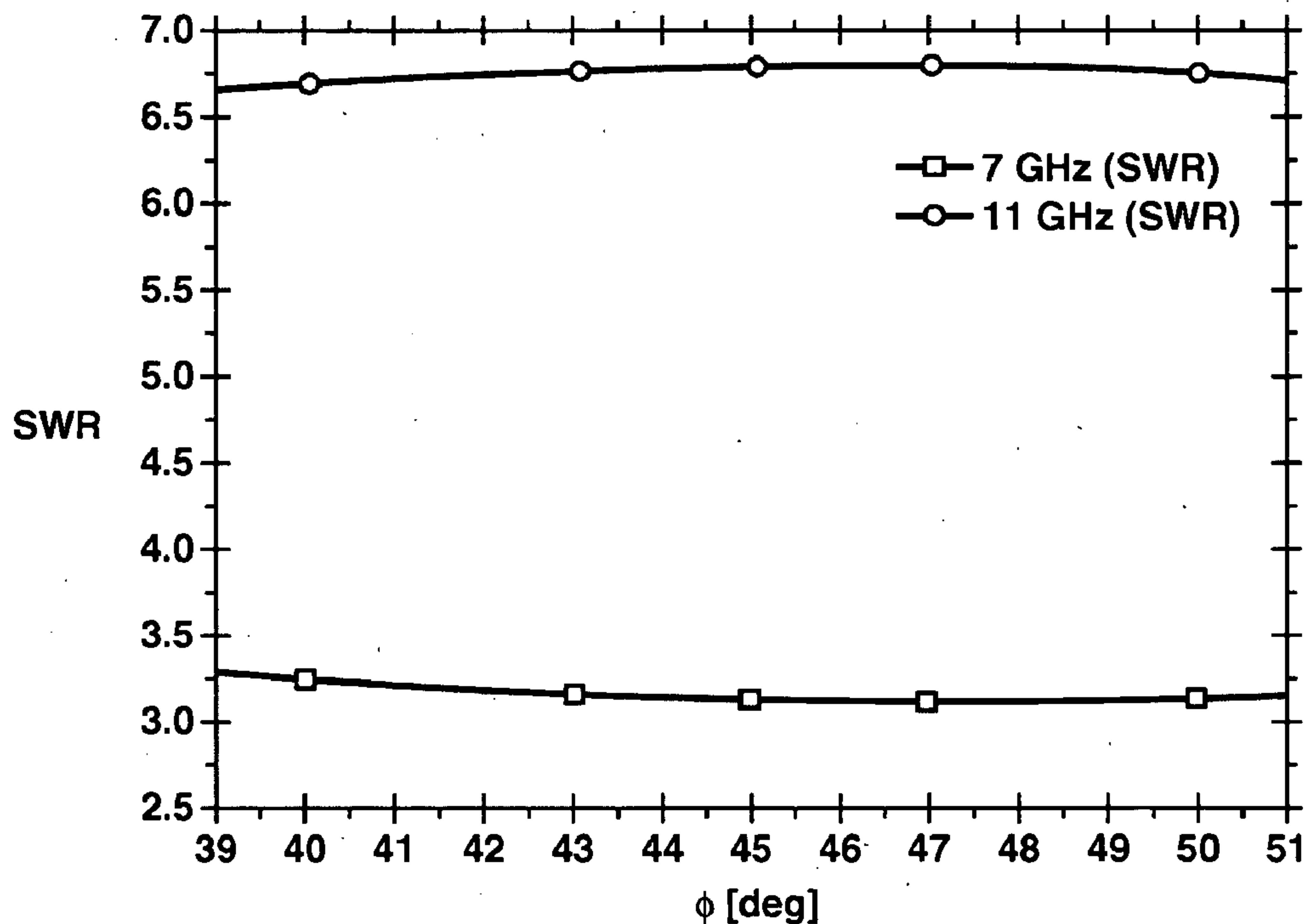
RELATIONSHIP BETWEEN SWR AND ANGLE \phi OF TAPER REGION (H: 6.0 mm \theta : 90° a: 8.4 mm W: 2.0 mm G: 0.6 mm d: 0.5 mm L: 0.7 mm)
