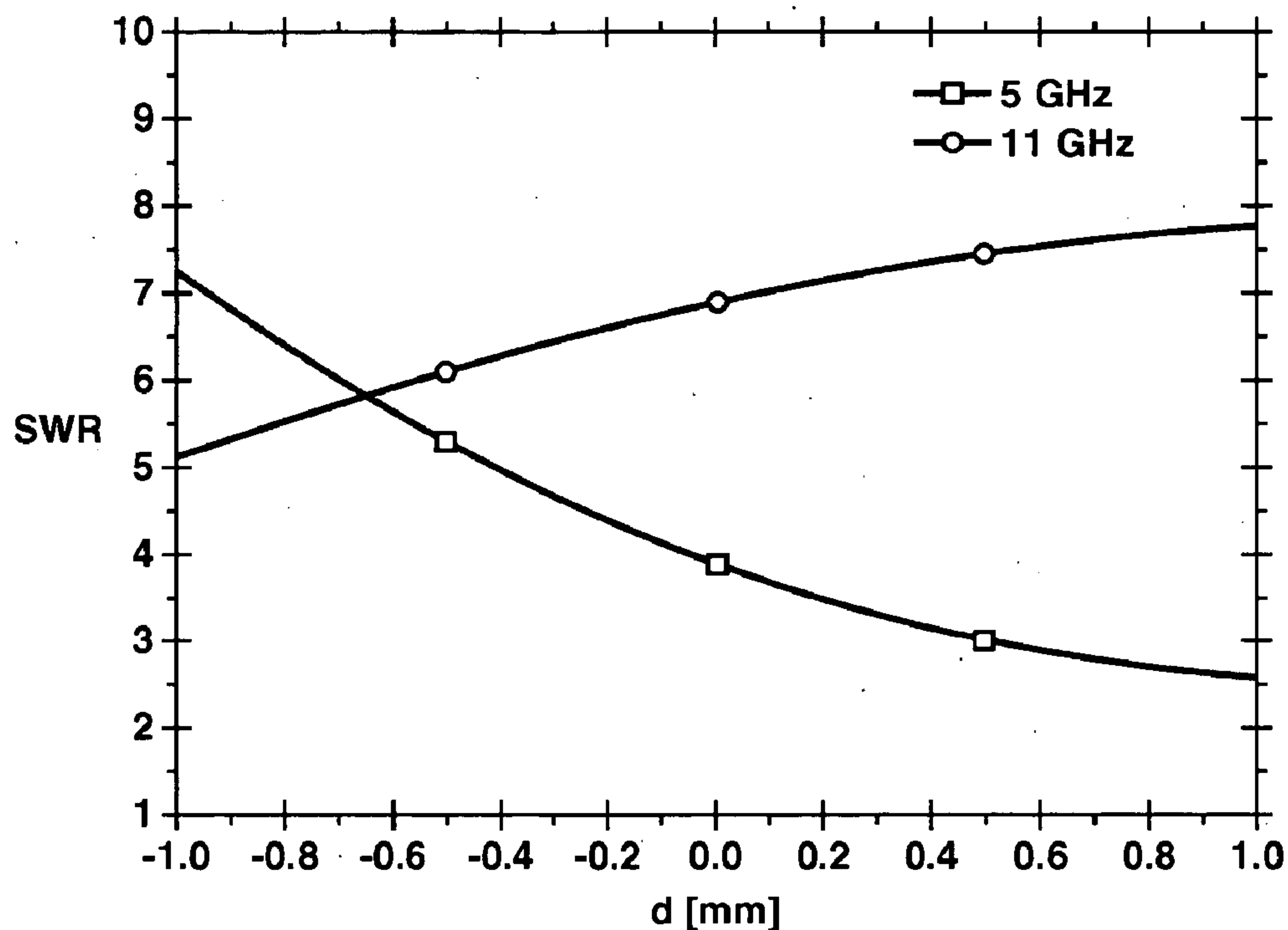
RELATIONSHIP BETWEEN SWR AND DISTANCE d BETWEEN ANTENNA AND GROUND (H: 6.0 mm \theta : 90° a: 8.4 mm W: 2.0 mm G: 0.6 mm \phi : — L: —)
