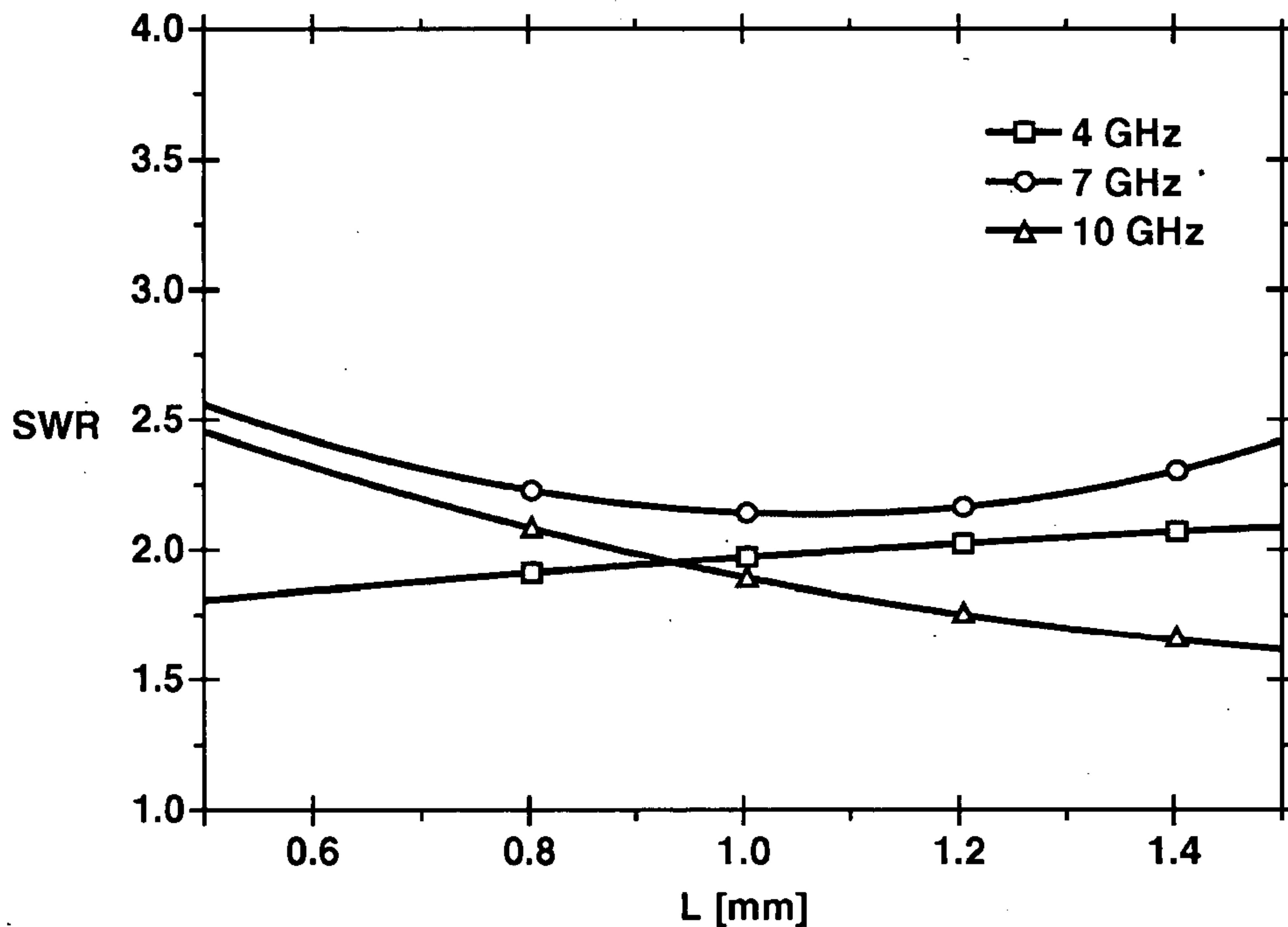
RELATIONSHIP BETWEEN SWR AND HEIGHT L OF TAPER REGION (H: 25.0 mm \theta : 90° a: 14.4 mm W: 2.0 mm G: 0.6 mm \phi : 45° d: 0.5 mm)
