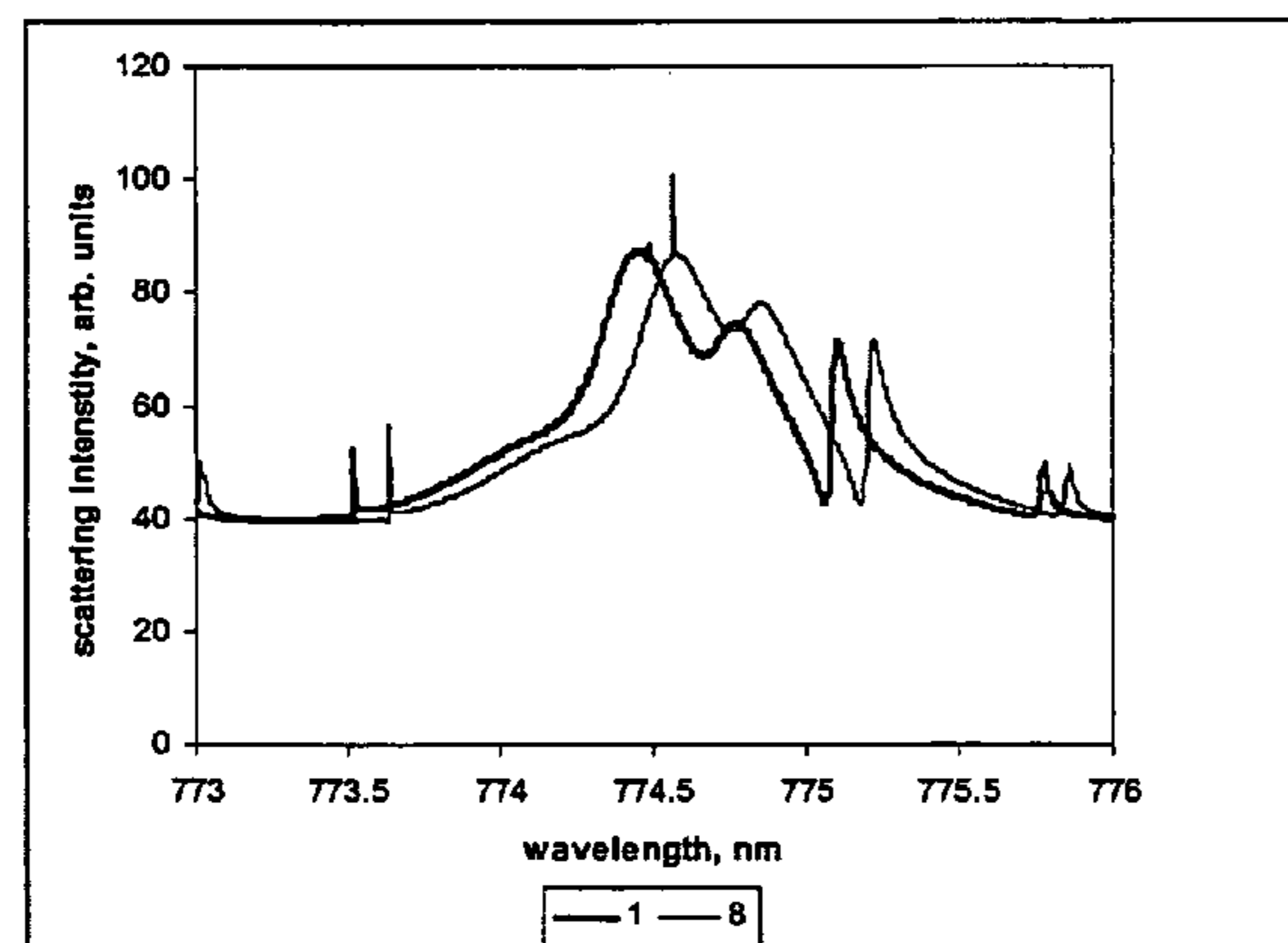
Particles 1 and 2 compared (expanded scale)
