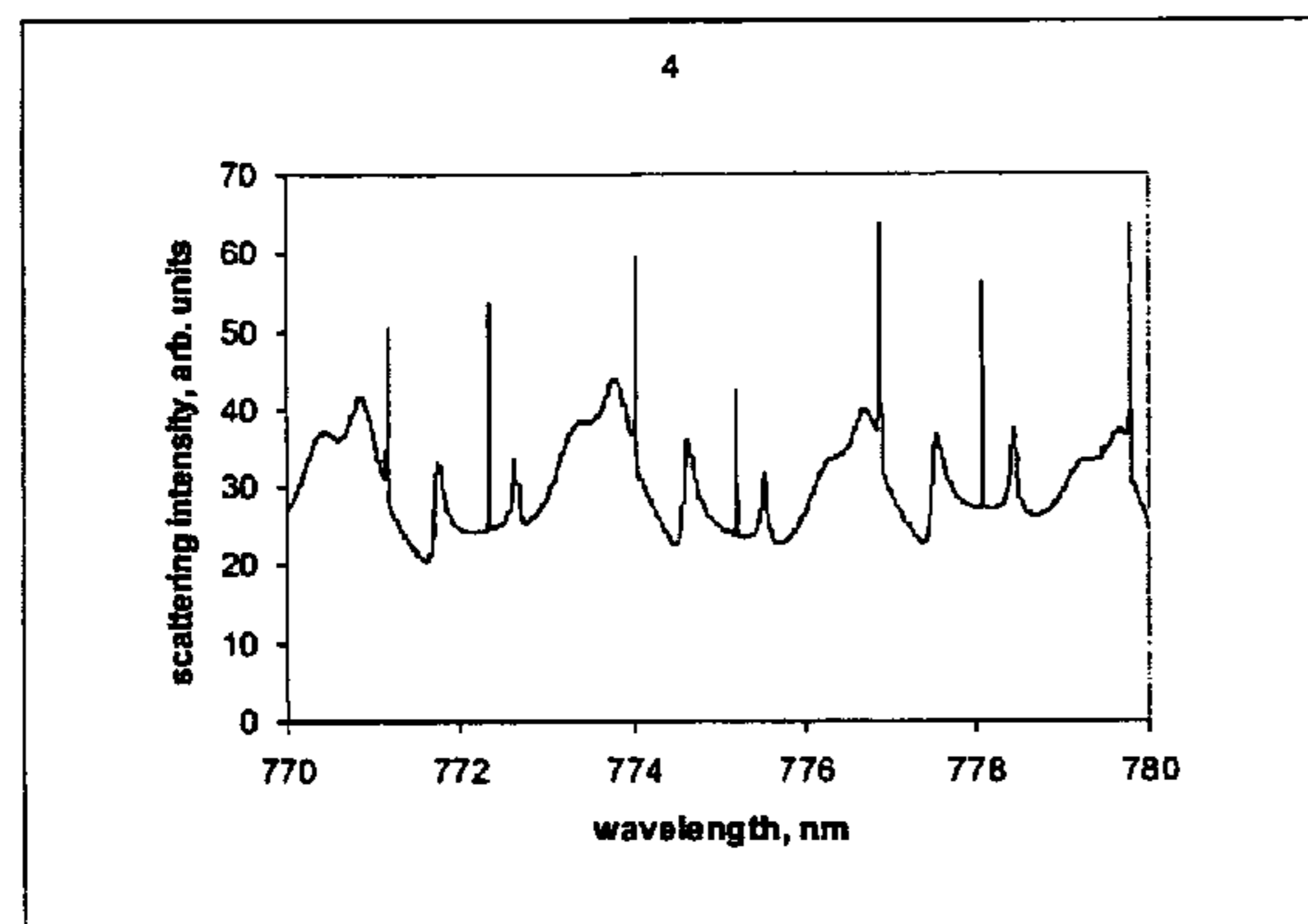
Scattering spectrum for particle 4
