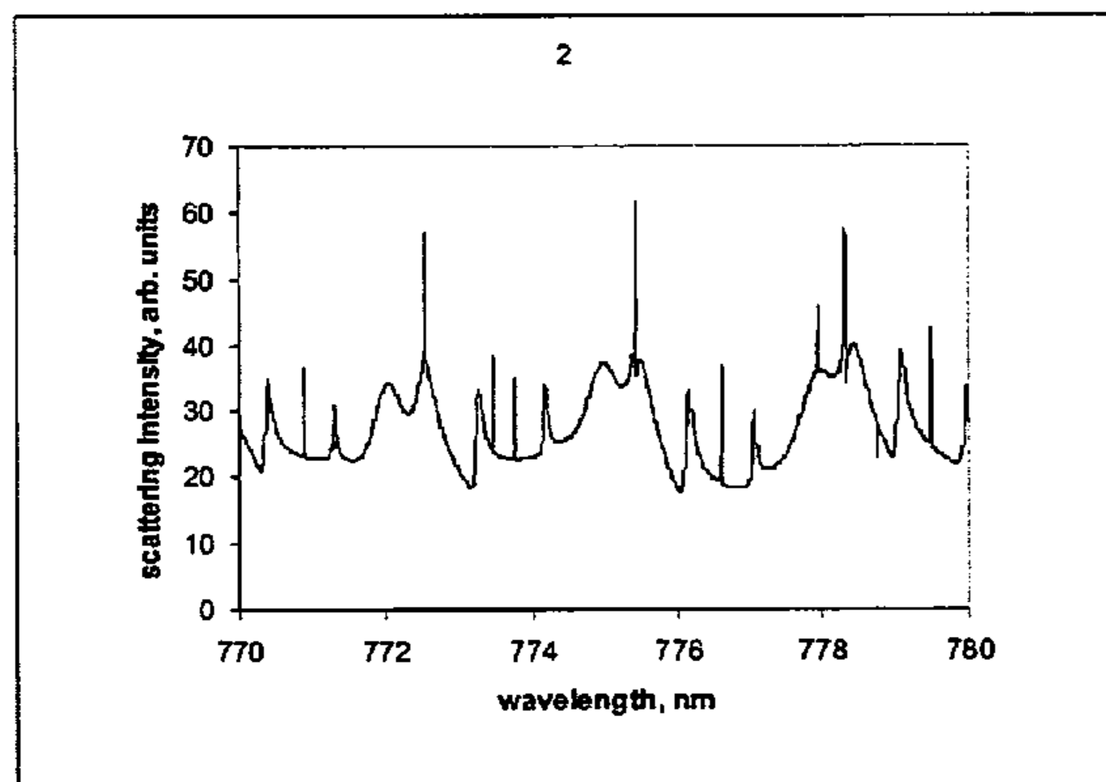
Scattering spectrum for particle 2
