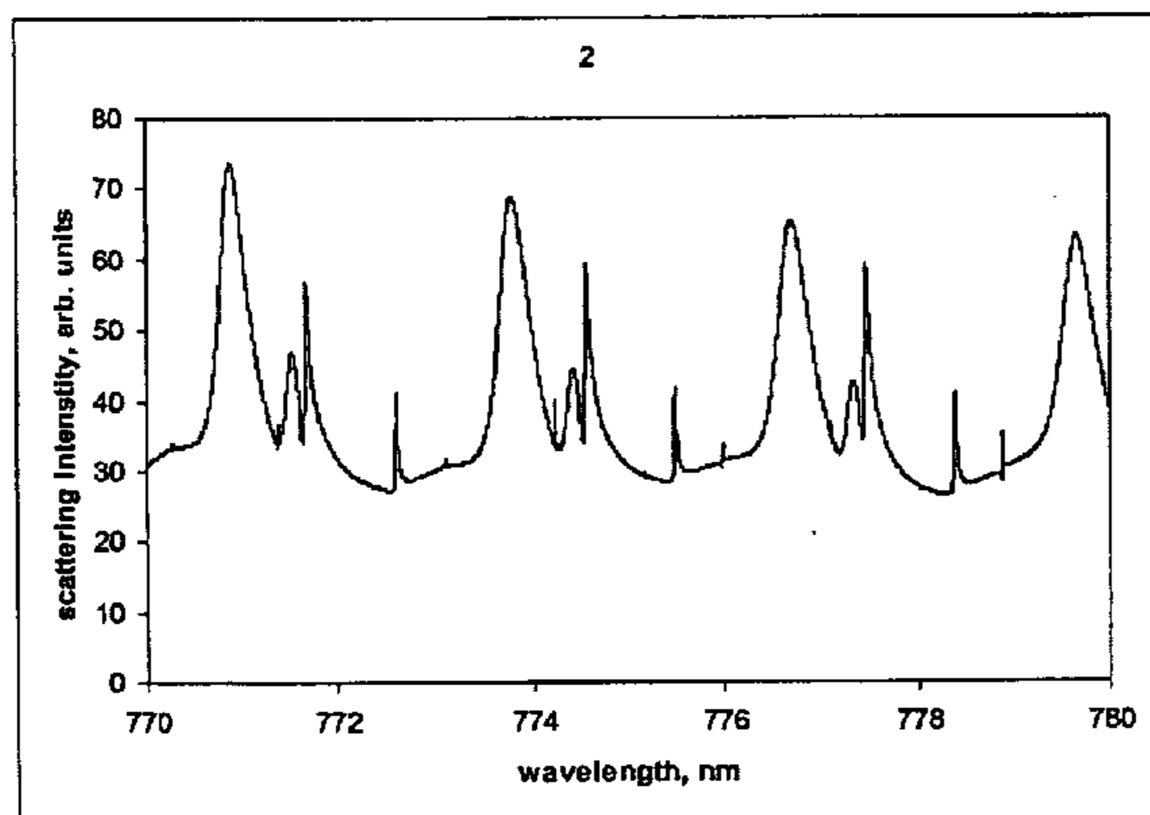
Scattering spectrum for particle 2, 5 μ core
