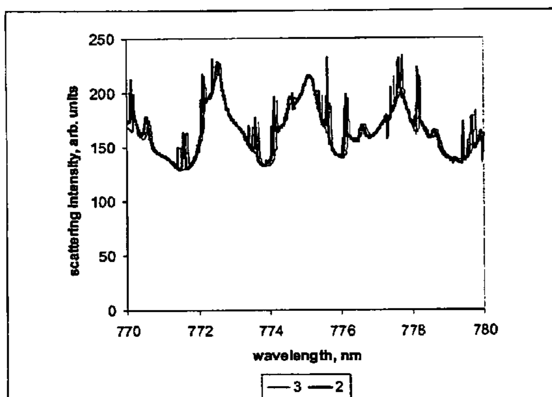
Scattering spectra for particles 2 and 3 compared
