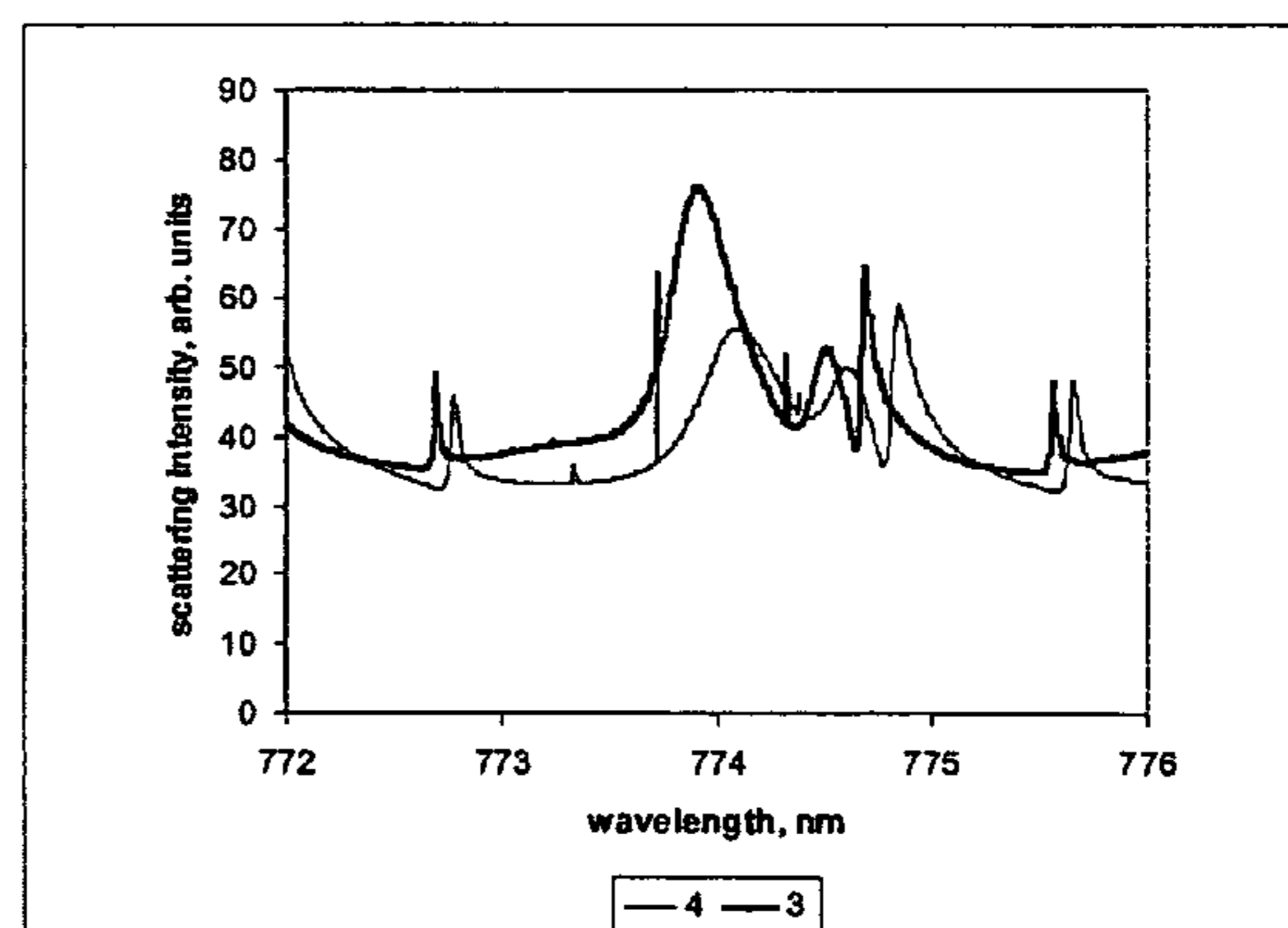
Scattering spectra for particles 3 and 4 compared (expanded scale)
