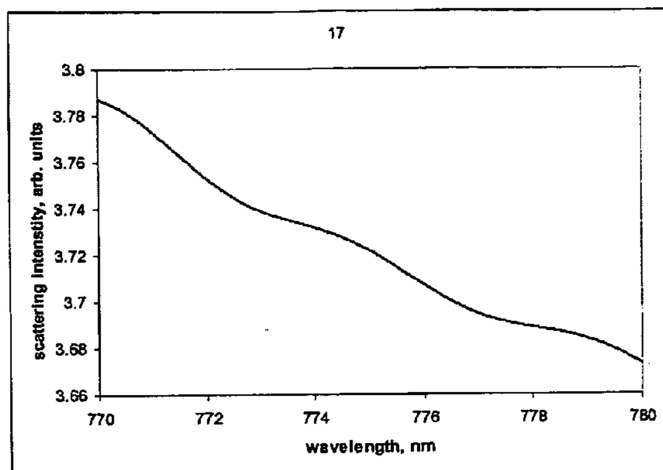
Scattering spectrum for particle 17 , 36 \mu core
