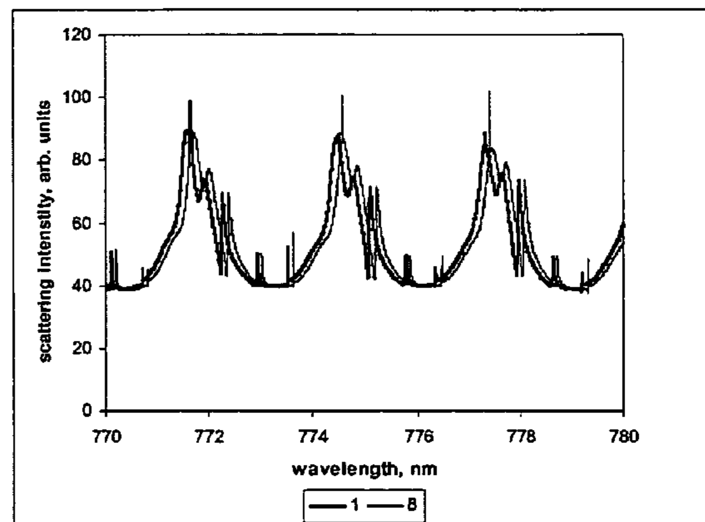
Scattering spectra for particles 1 and 8 compared
