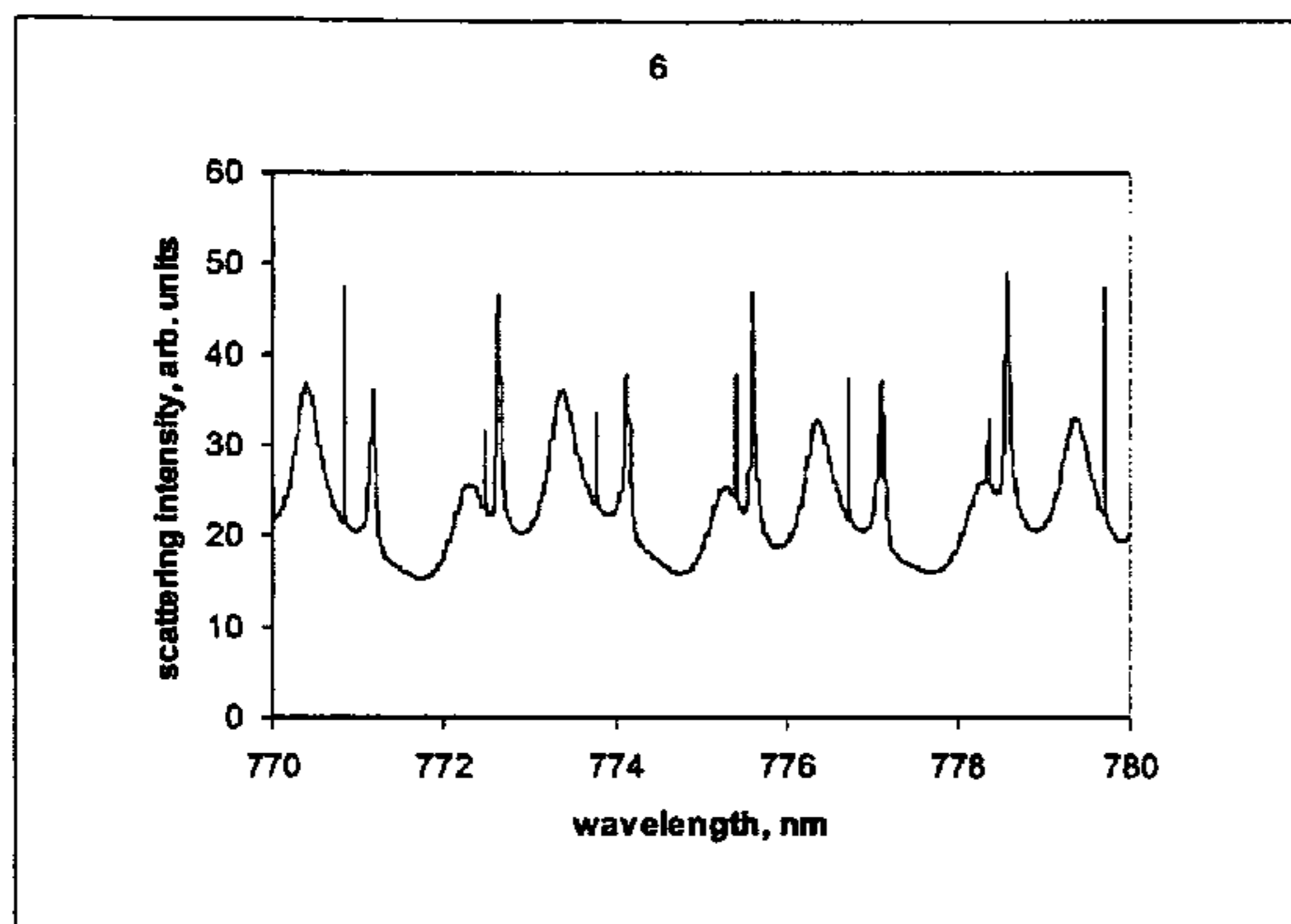
Scattering spectra for particle 6
