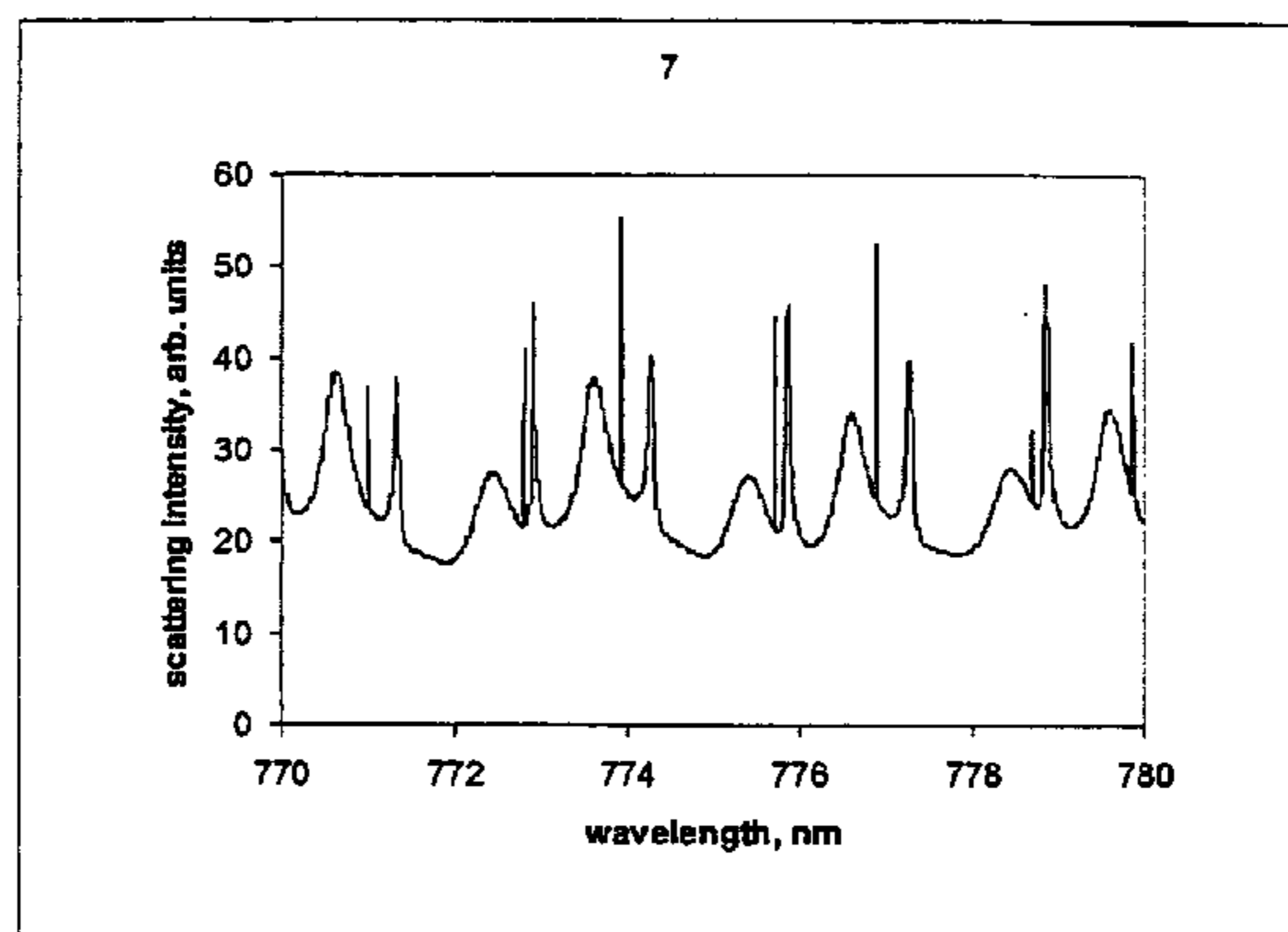
Scattering spectra for particle 7
