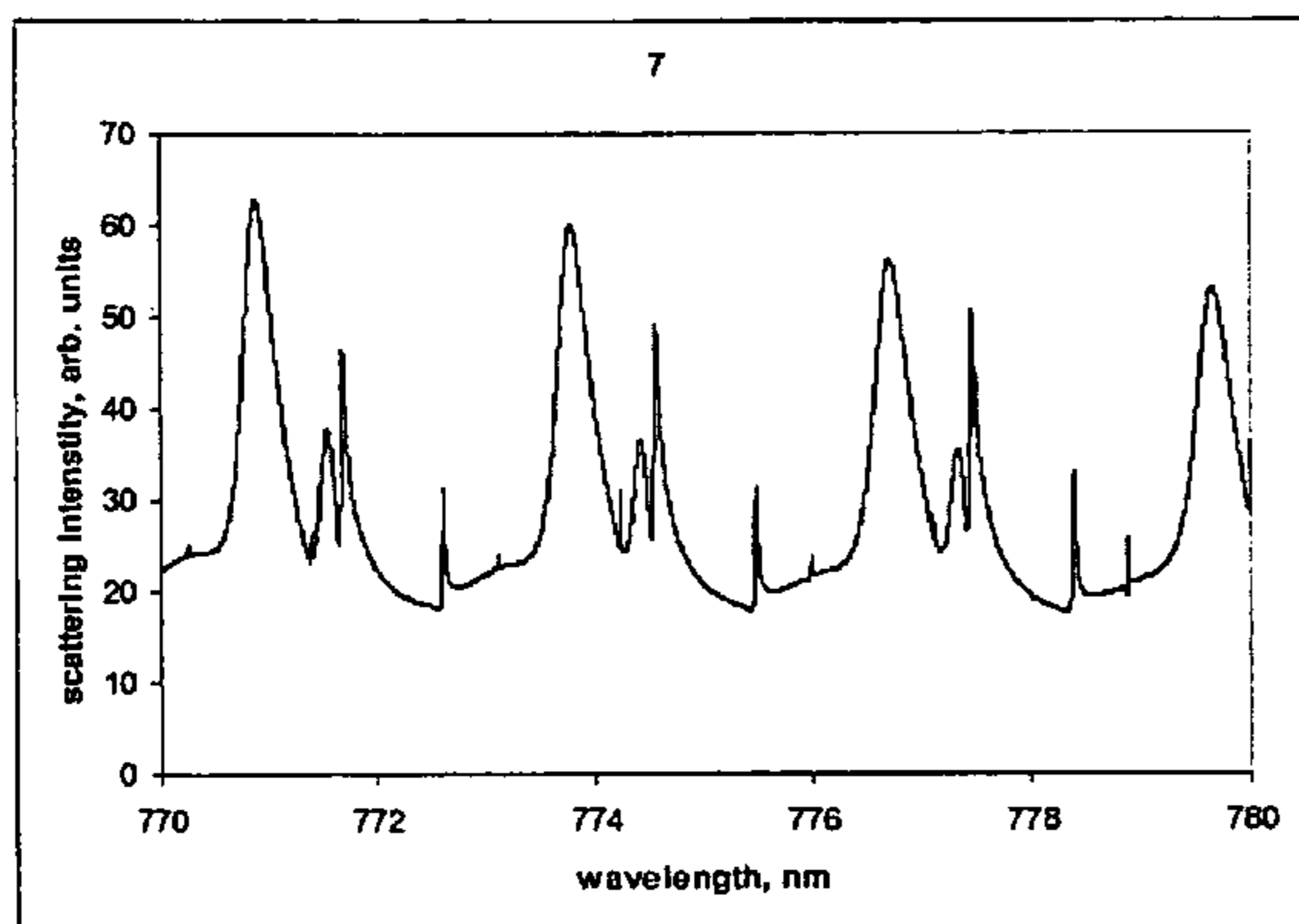
Scattering spectrum for particle 7 , 26 \mu core
