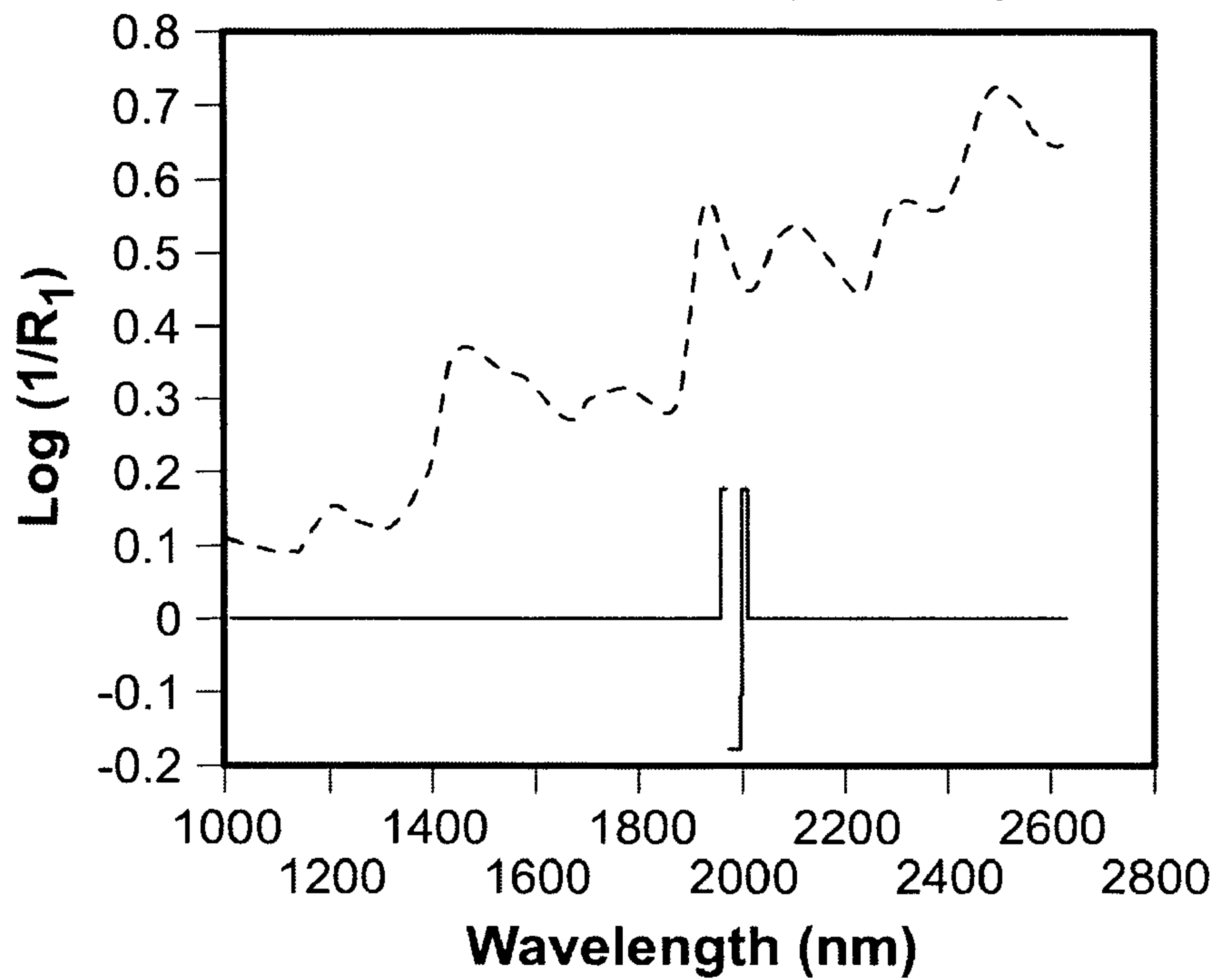
Typical Wheat Spectrum (Top) and Example Feature Vector (Bottom)
