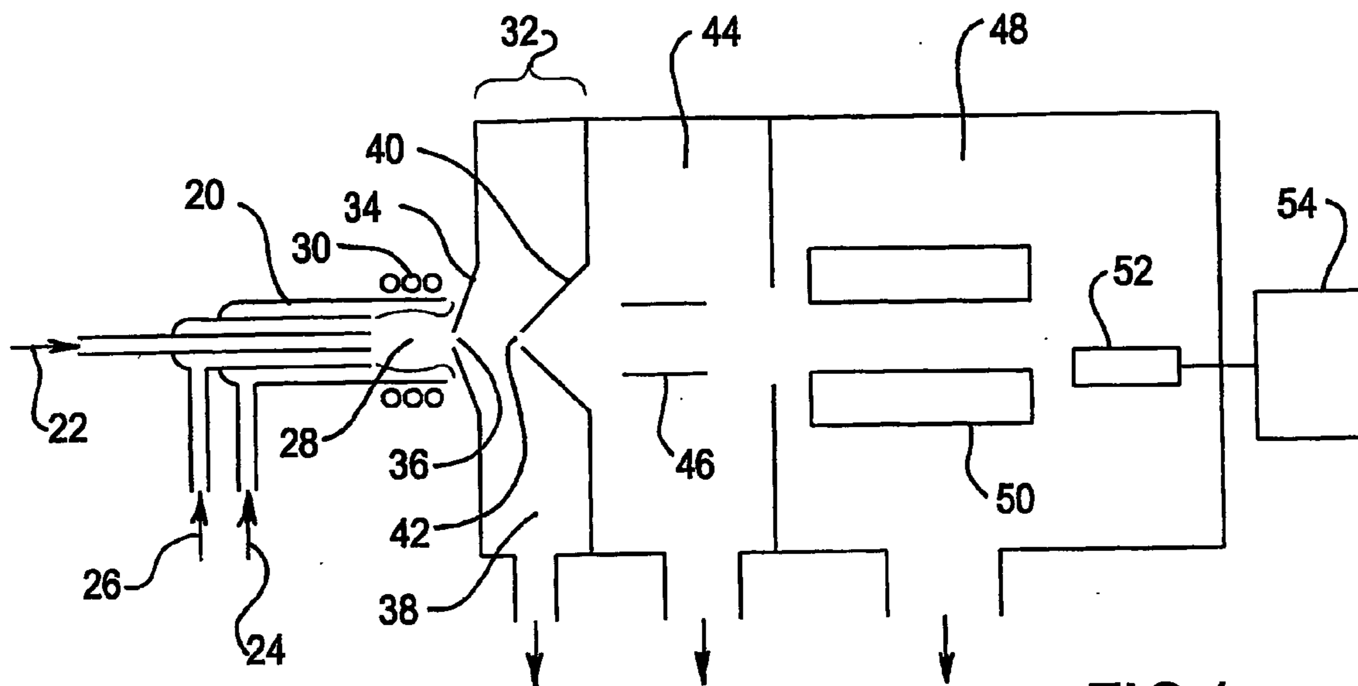
FIG 1 (PRIOR ART)
