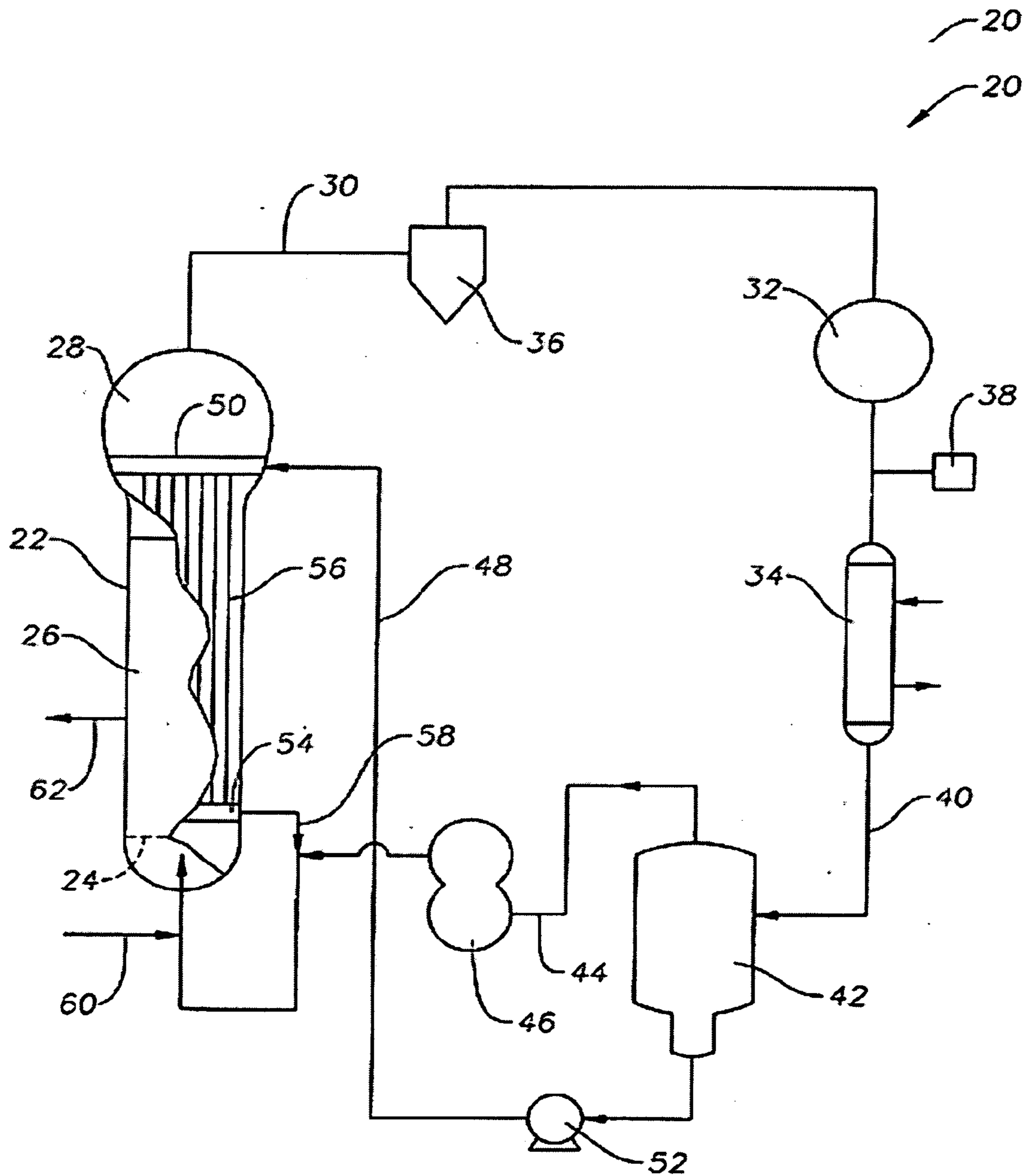
Figure 1. Gas Phase Fluidized Bed Reactor
