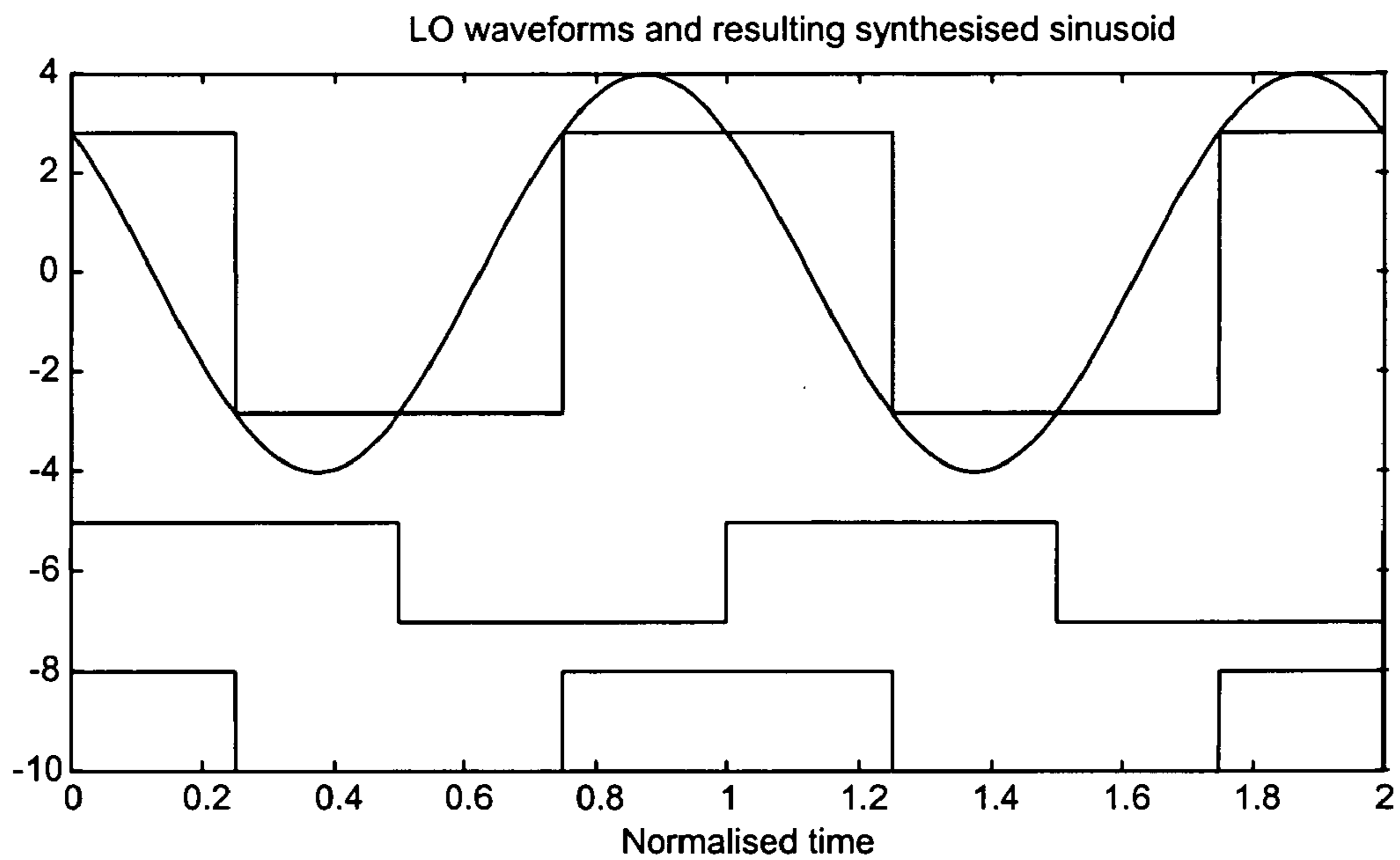
FIG. 11 2 phase, 1 cycle, 1 LO
