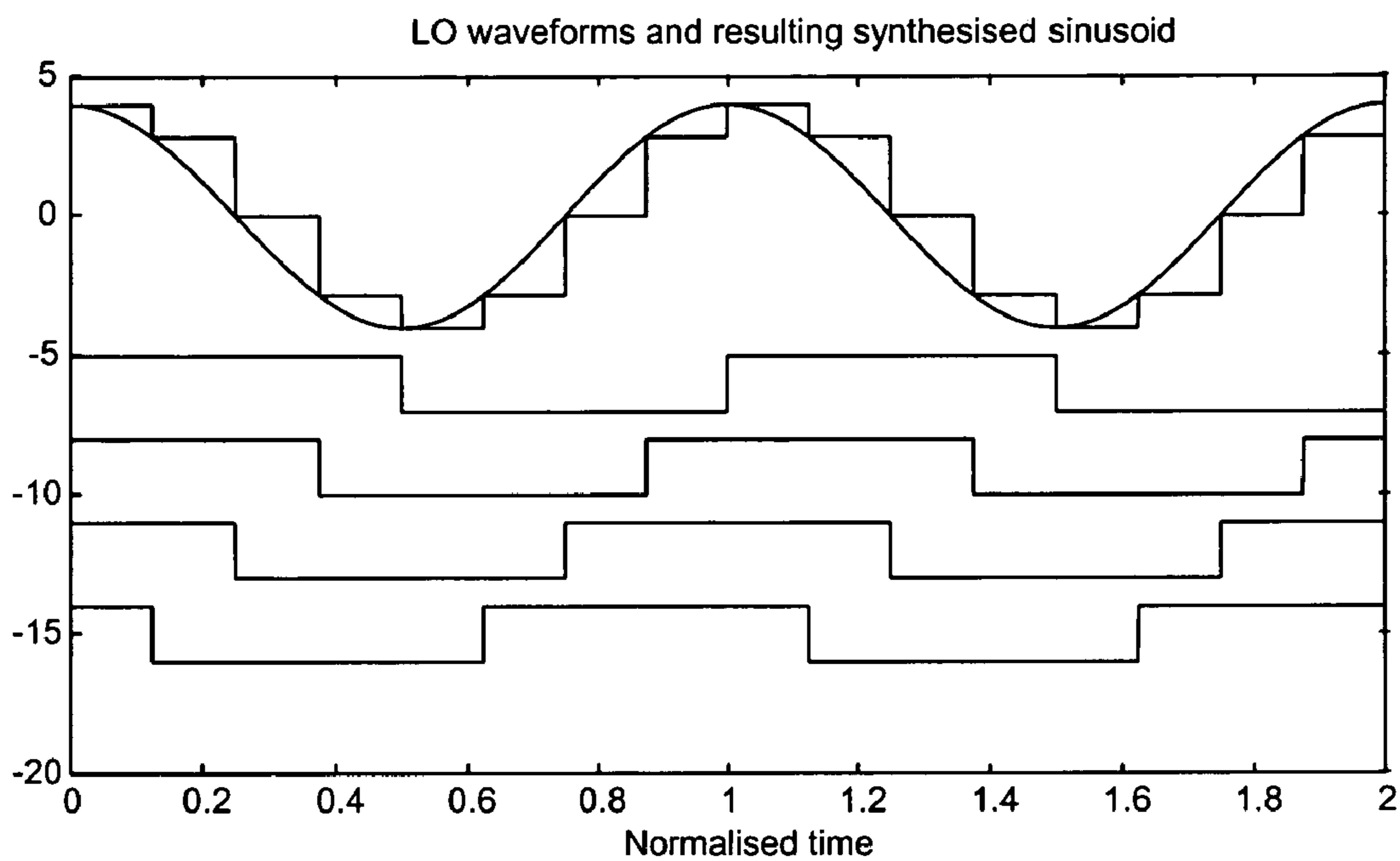
FIG. 10 4 phase, 1 cycle, Q LO
