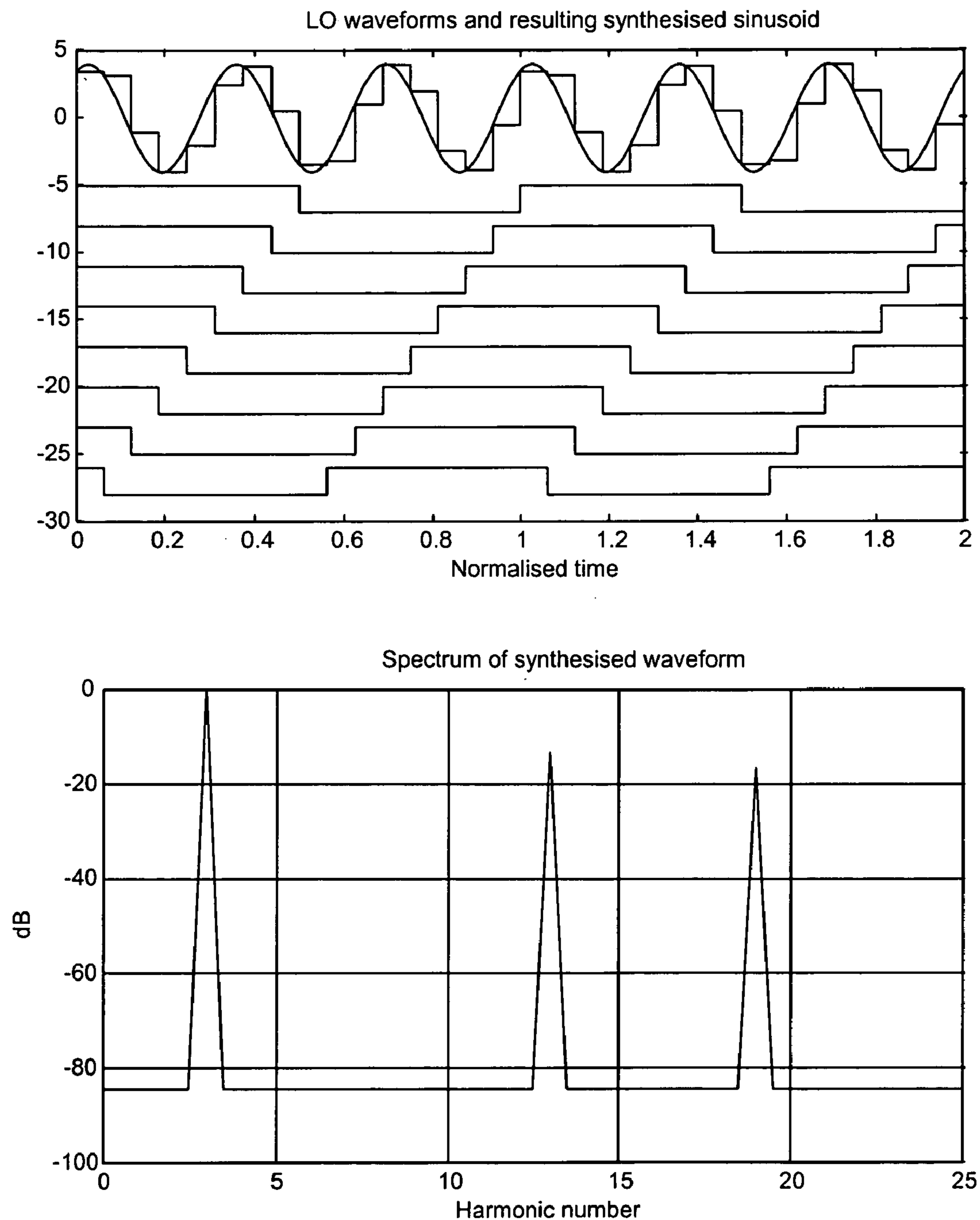
FIG. 8 8 phase, 3 cycle, Q LO
