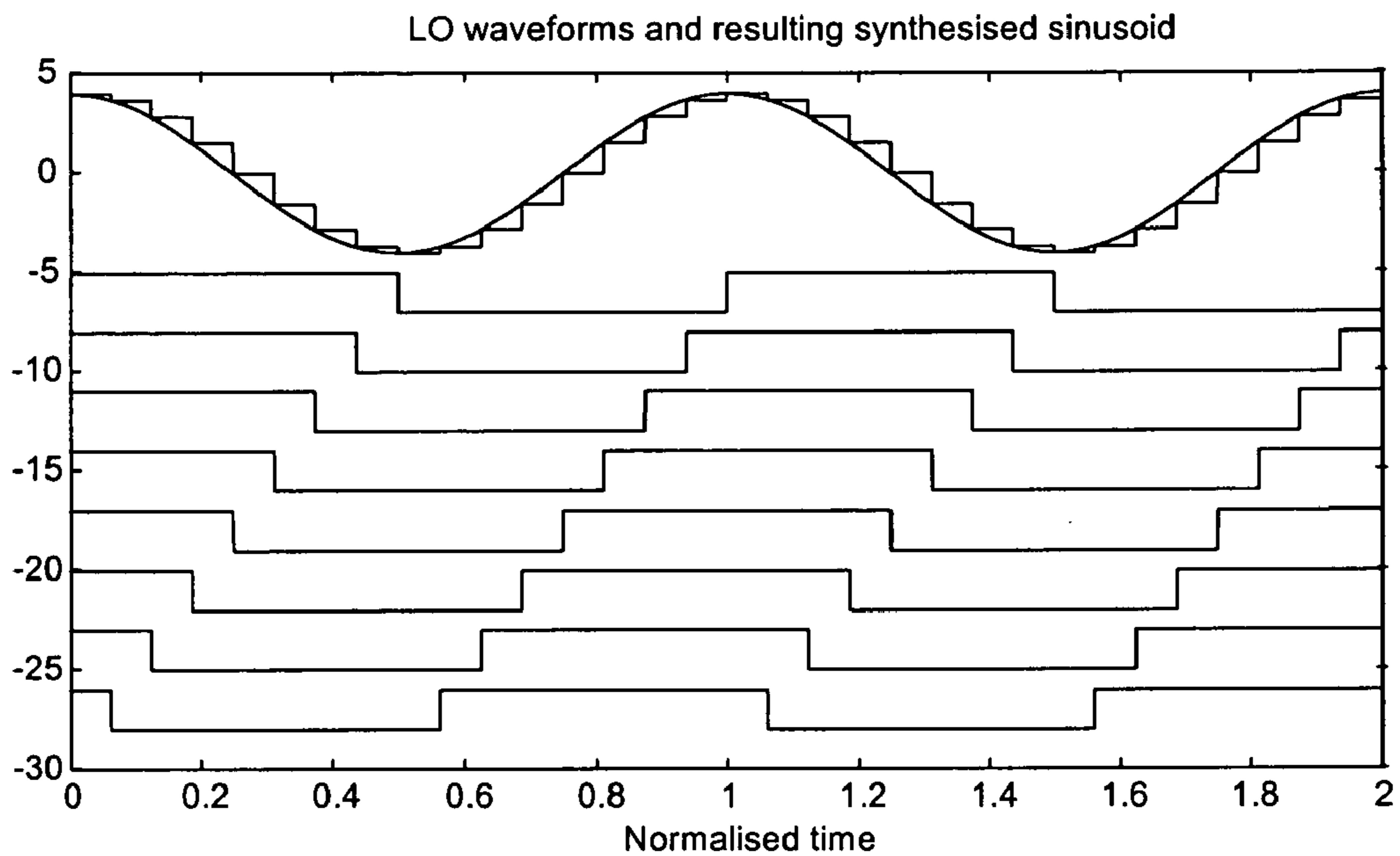
FIG. 6 8 phase, 1 cycle, Q LO
