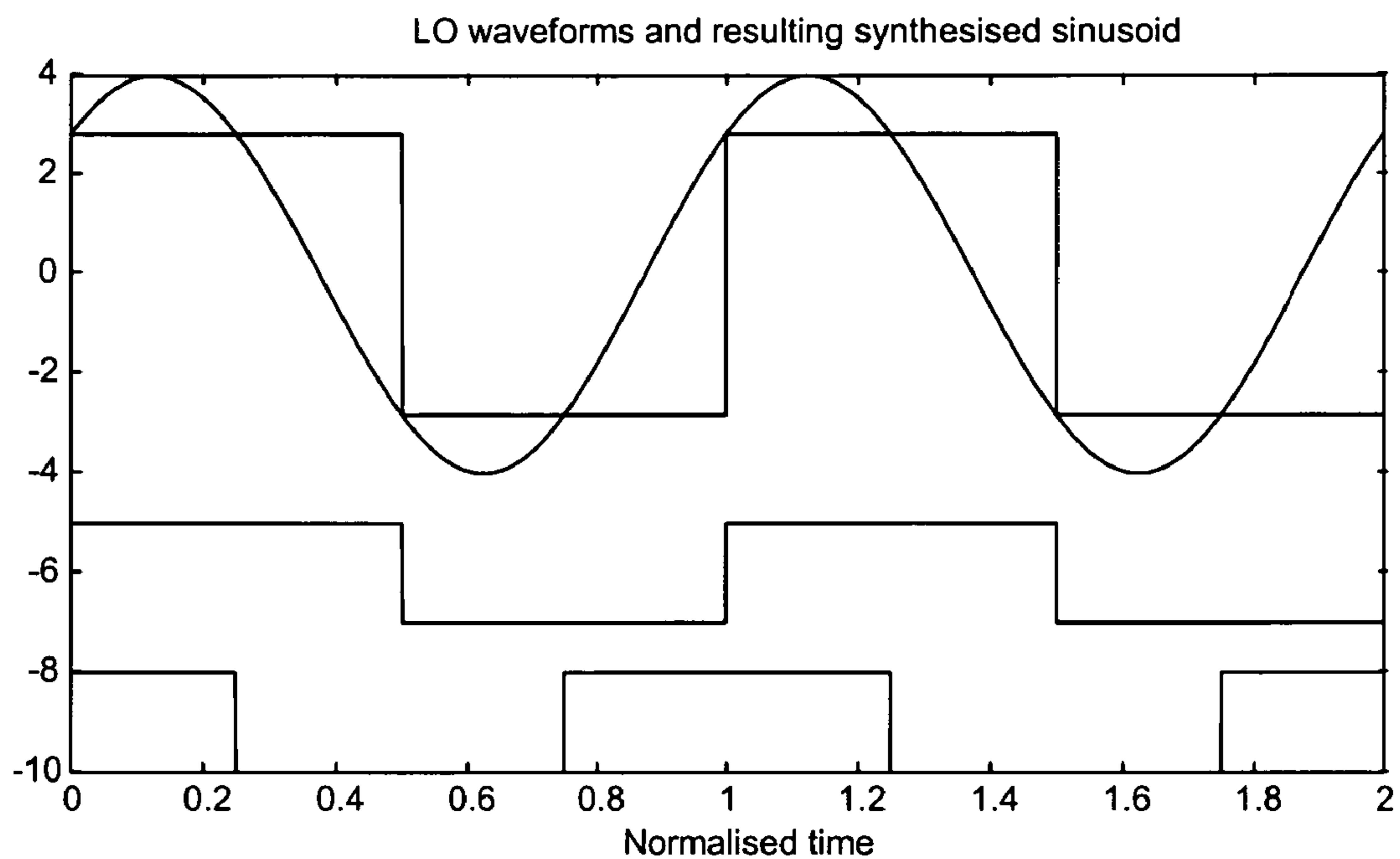
FIG. 12 2 phase, 1 cycle, Q LO
