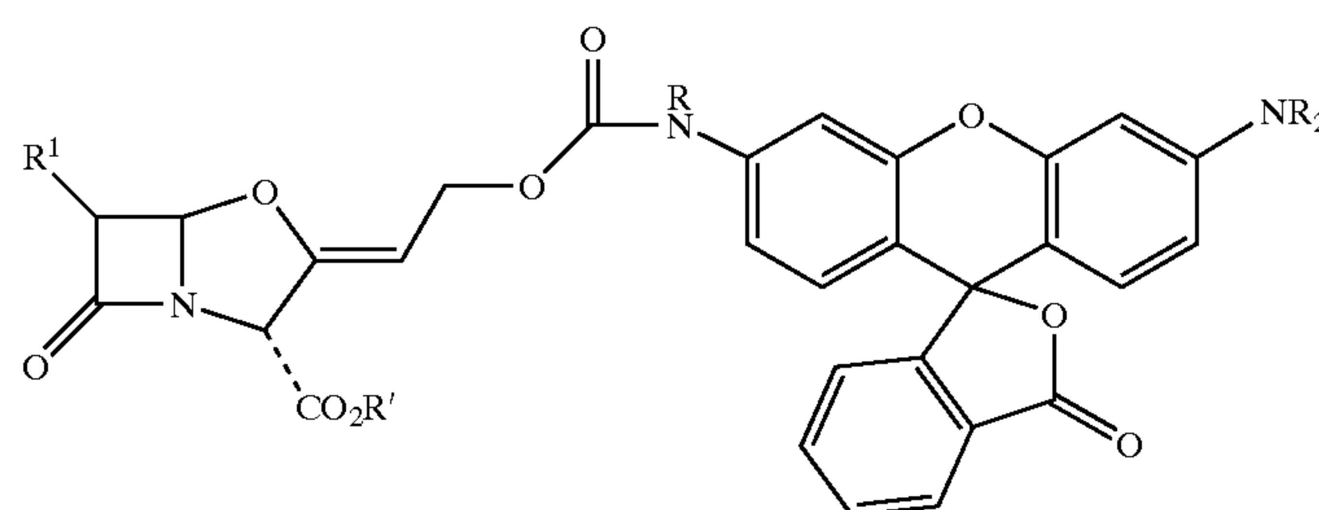
Compound 53
