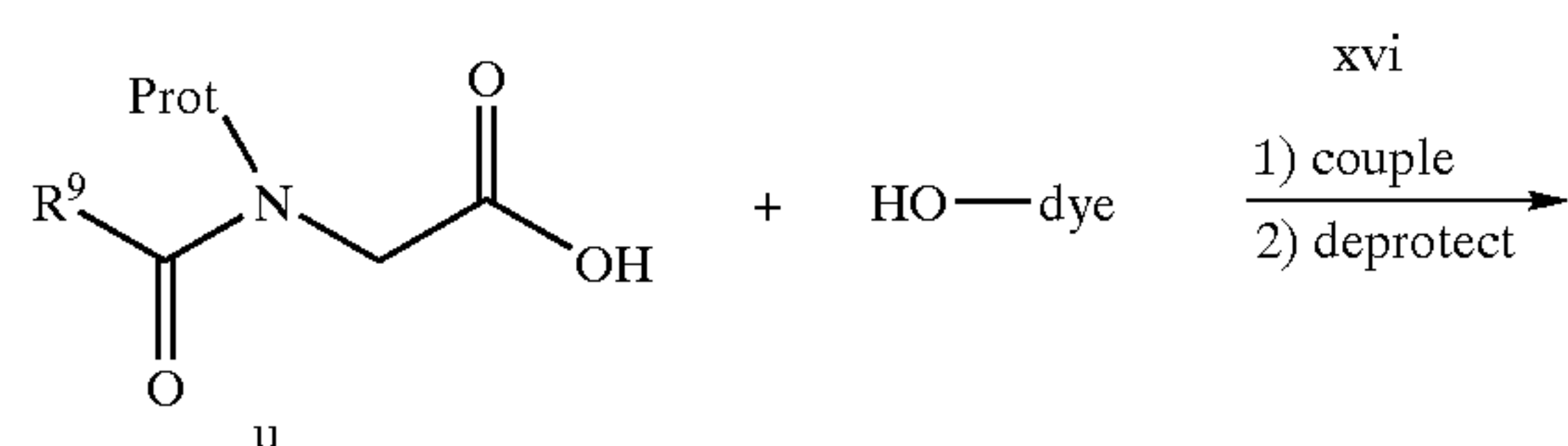
Scheme 14
