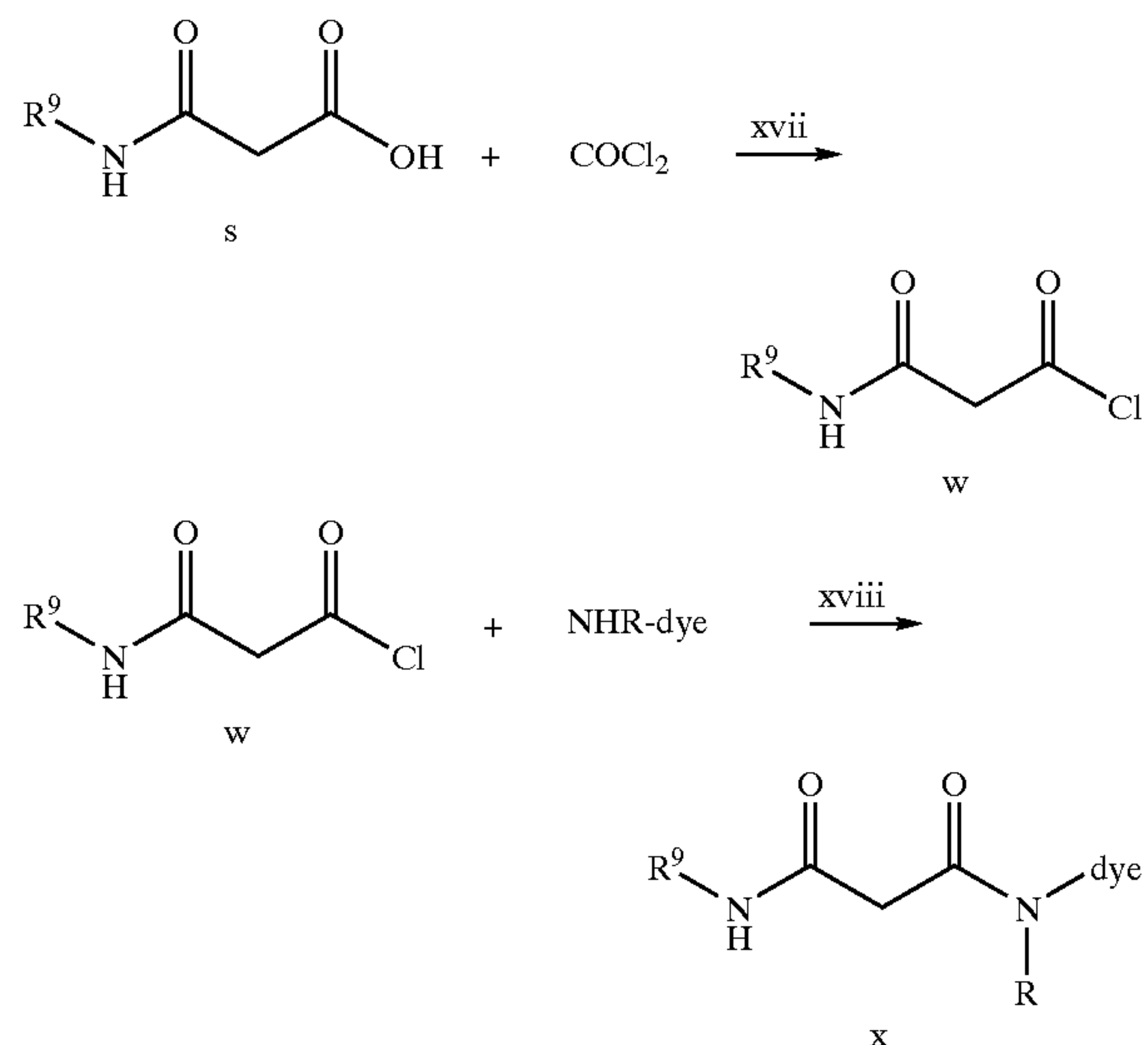
Scheme 15
