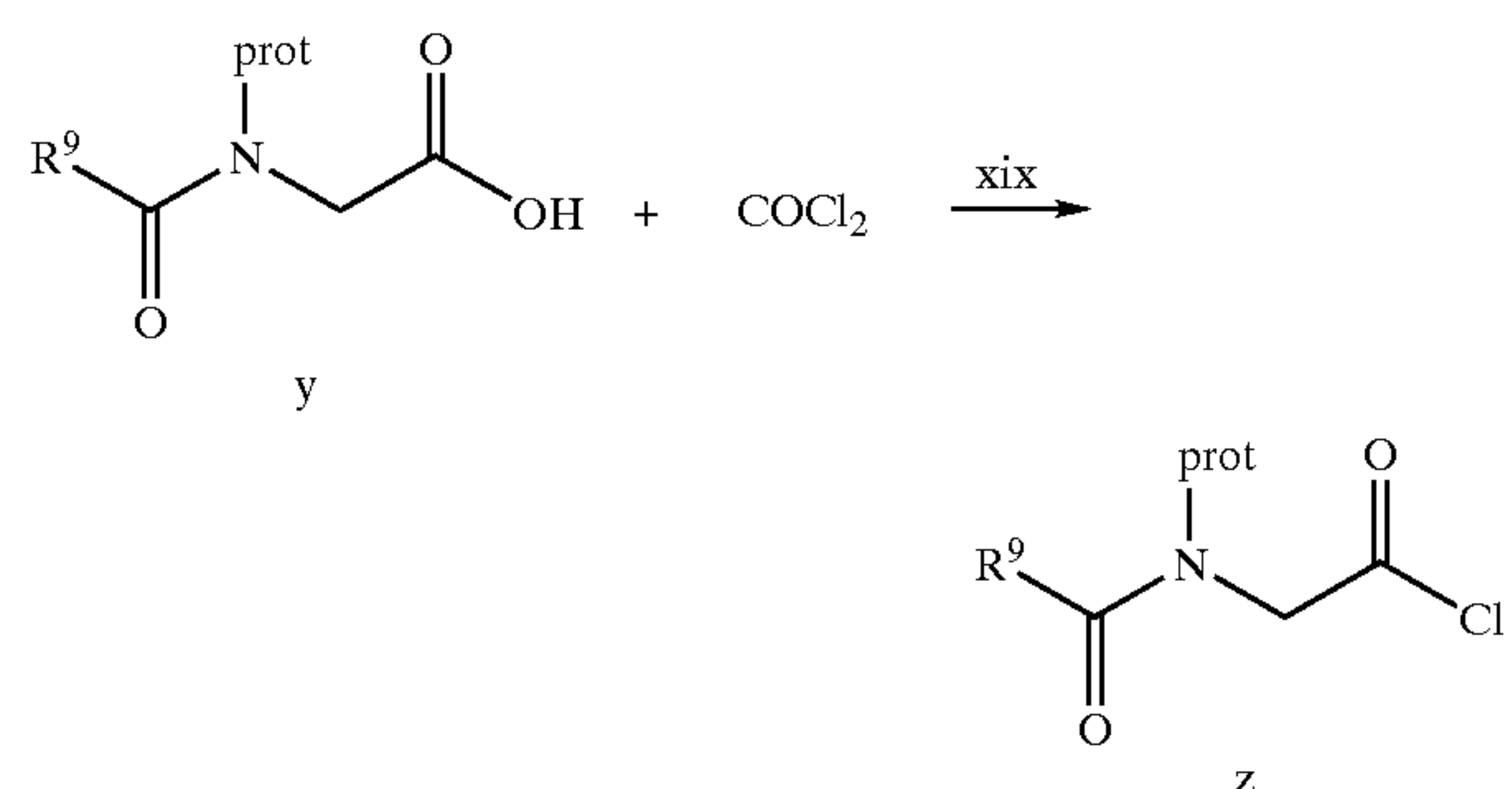
Scheme 16
