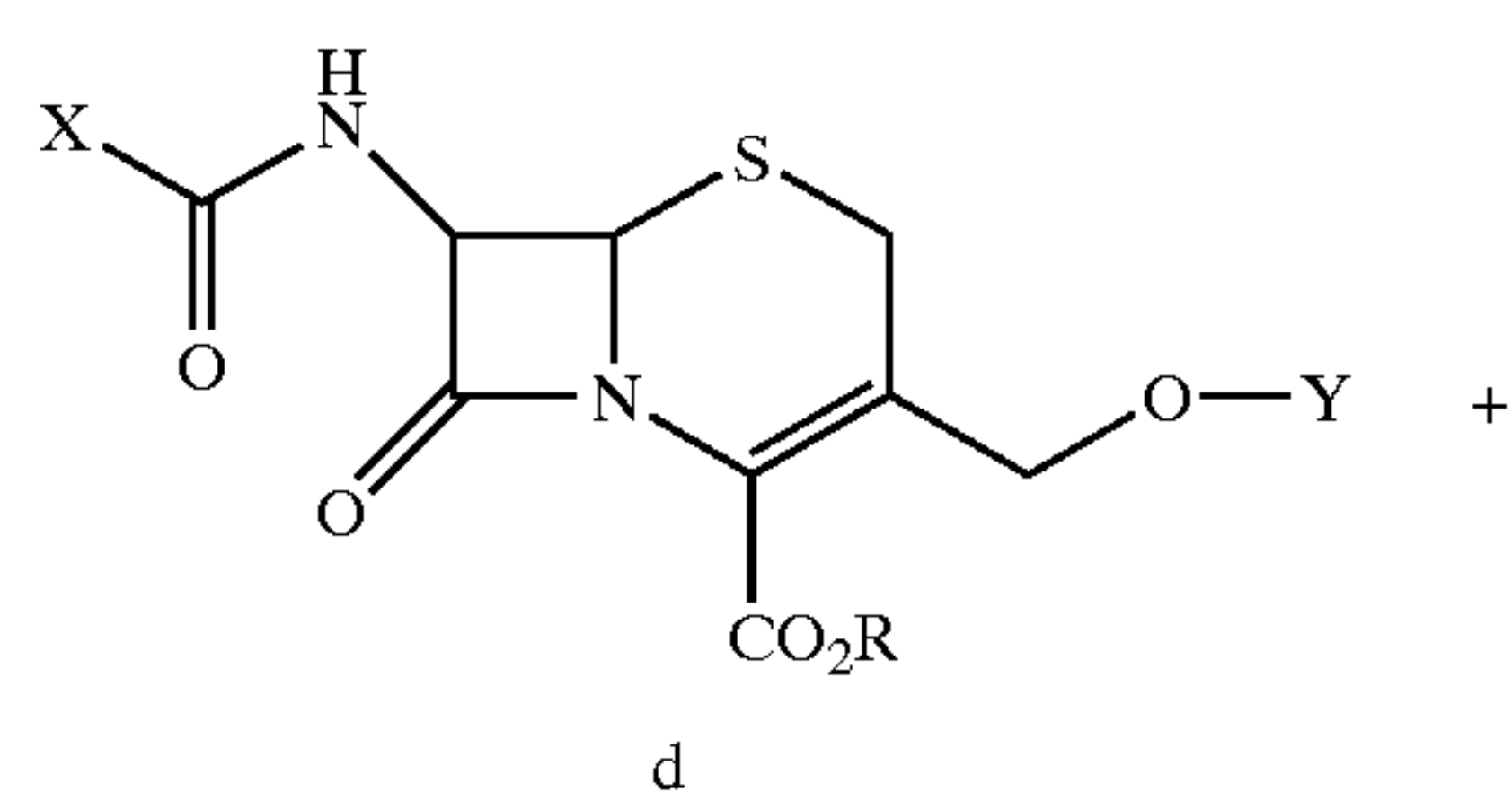
Scheme 6
