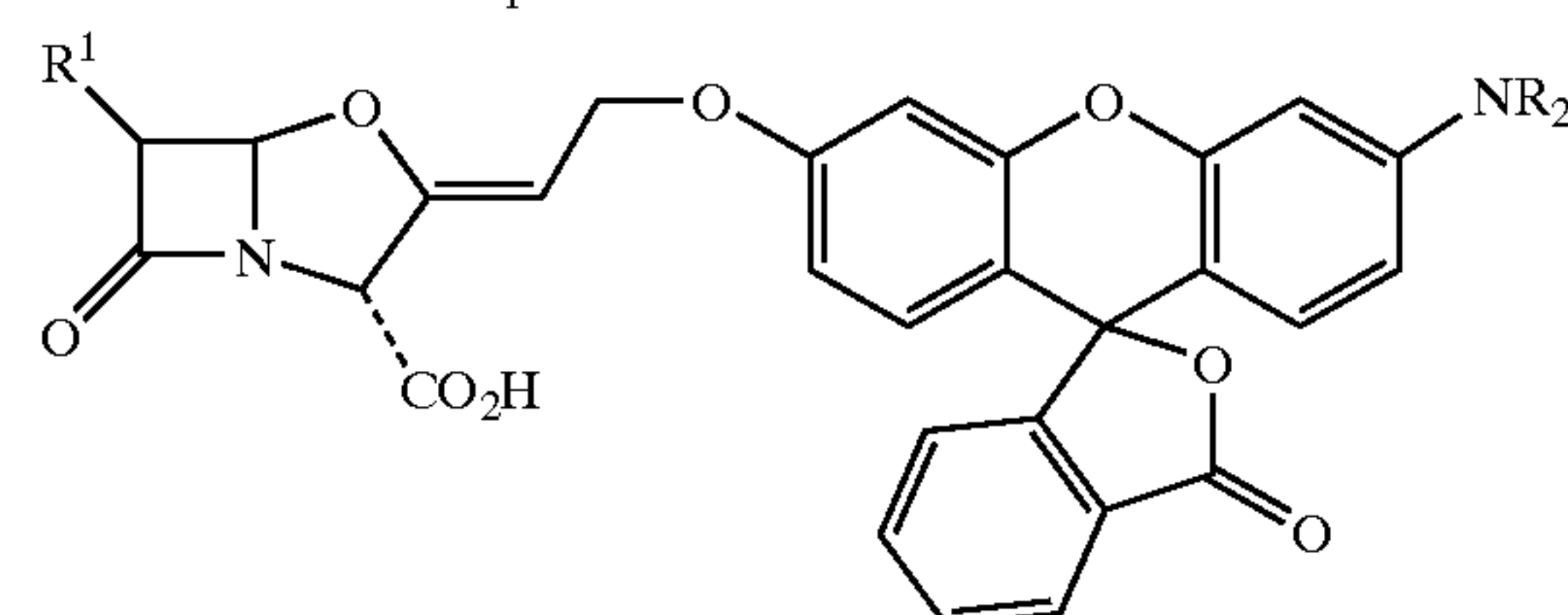
Compound 51
