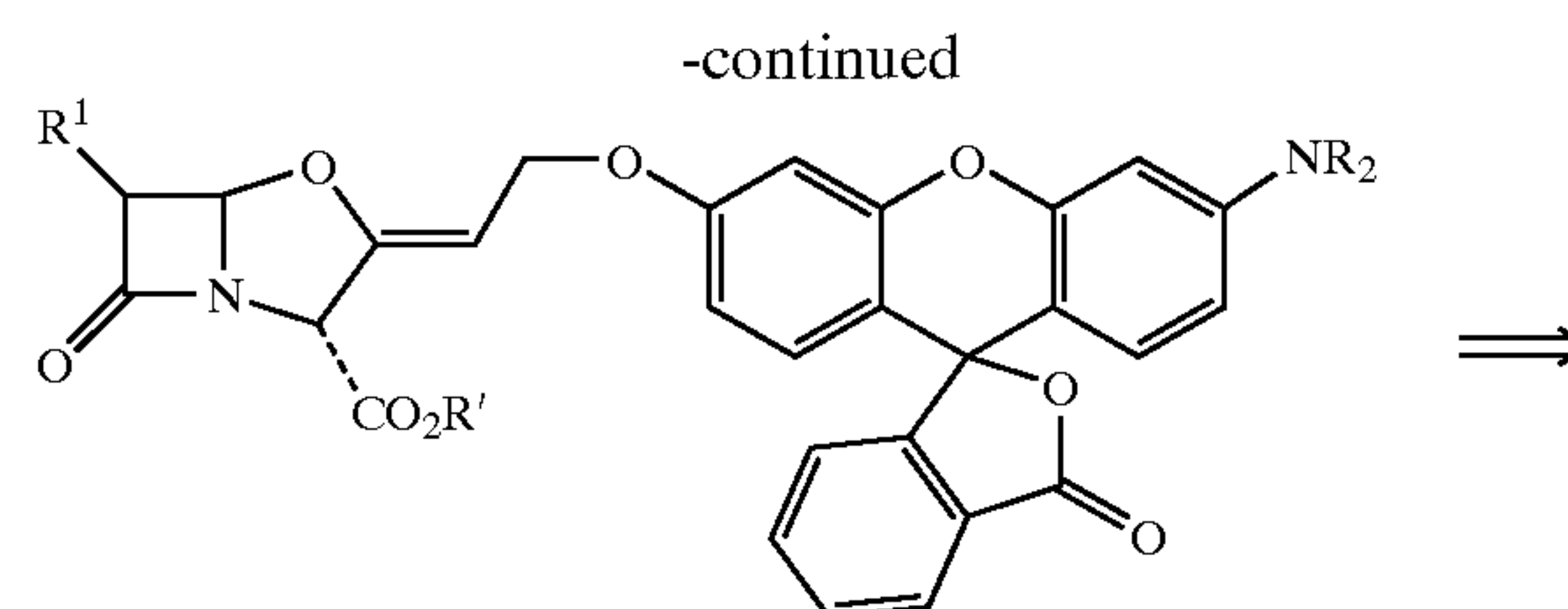
Compound 51
