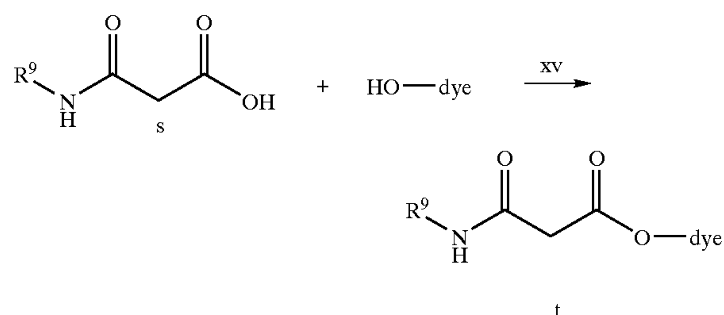
Scheme 13
