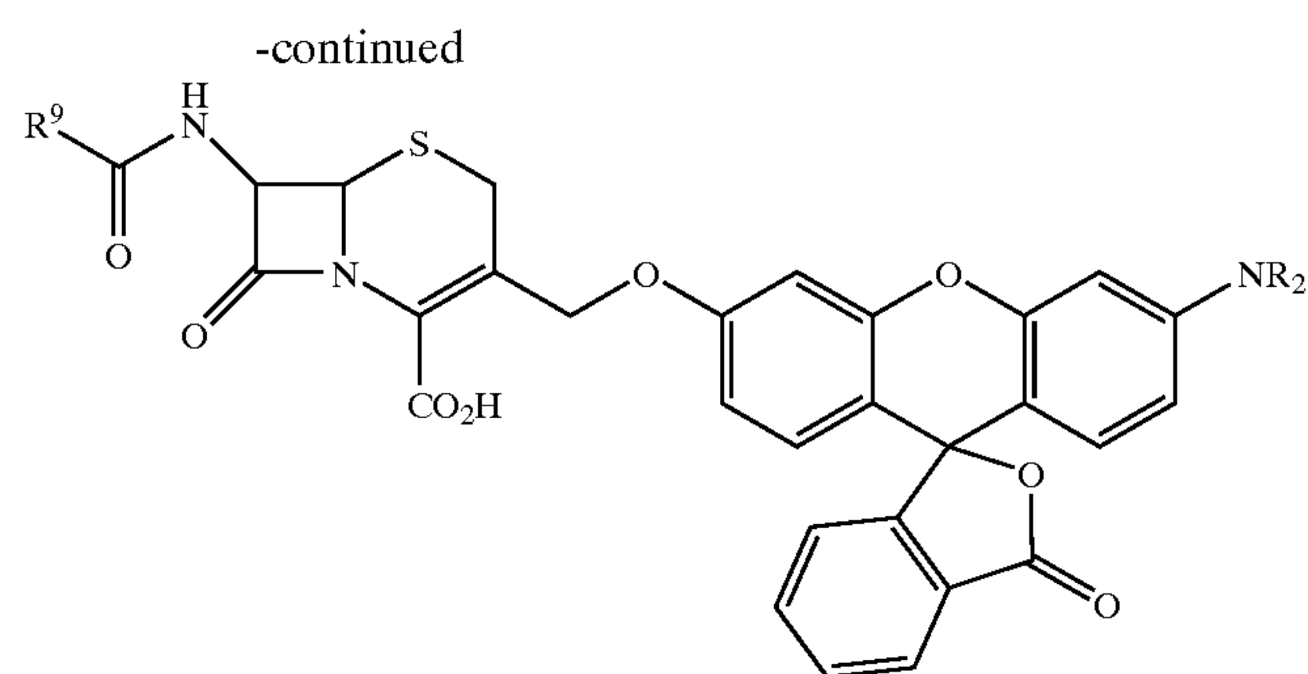
Compound 48
