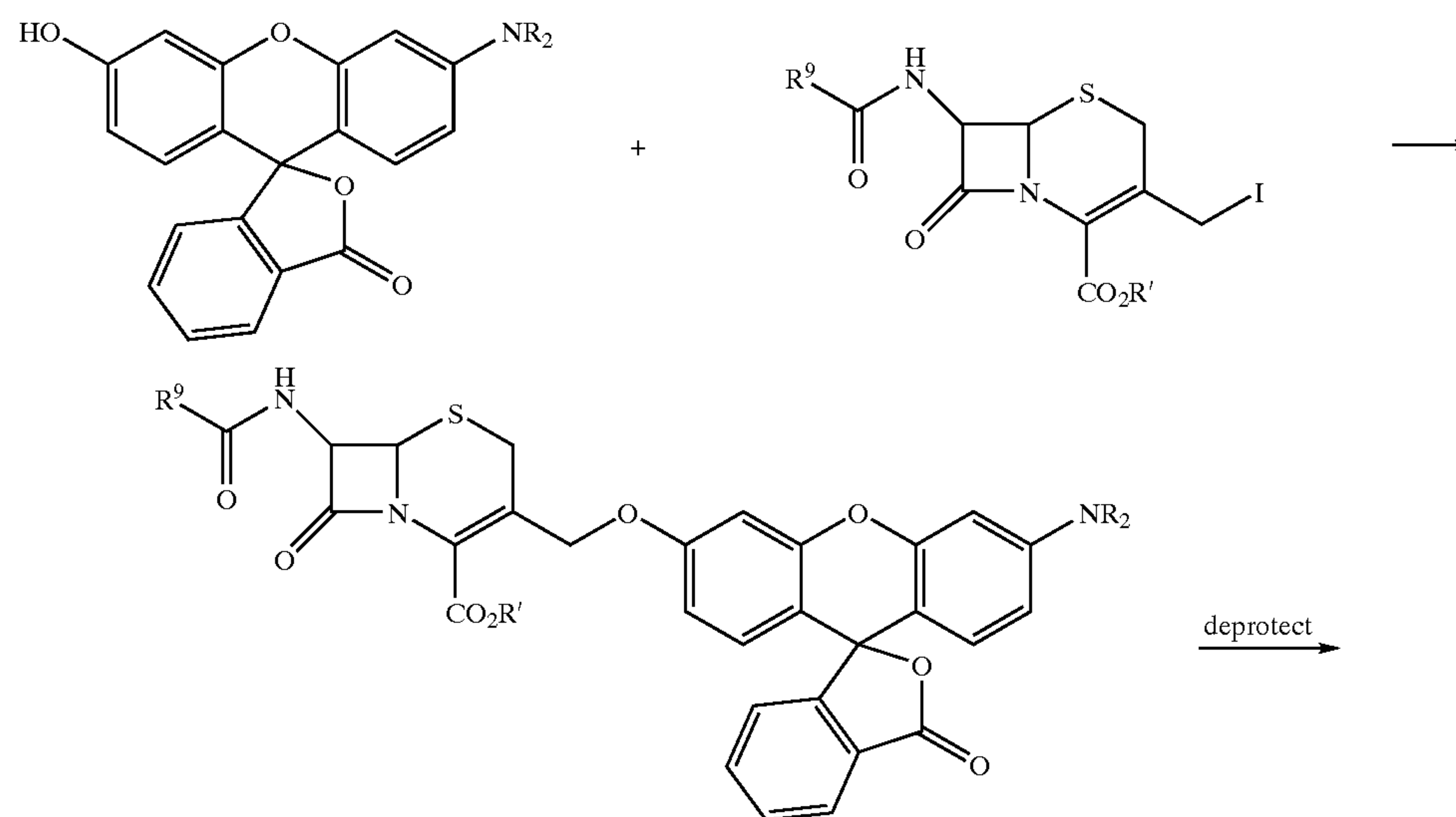
Compound 47
