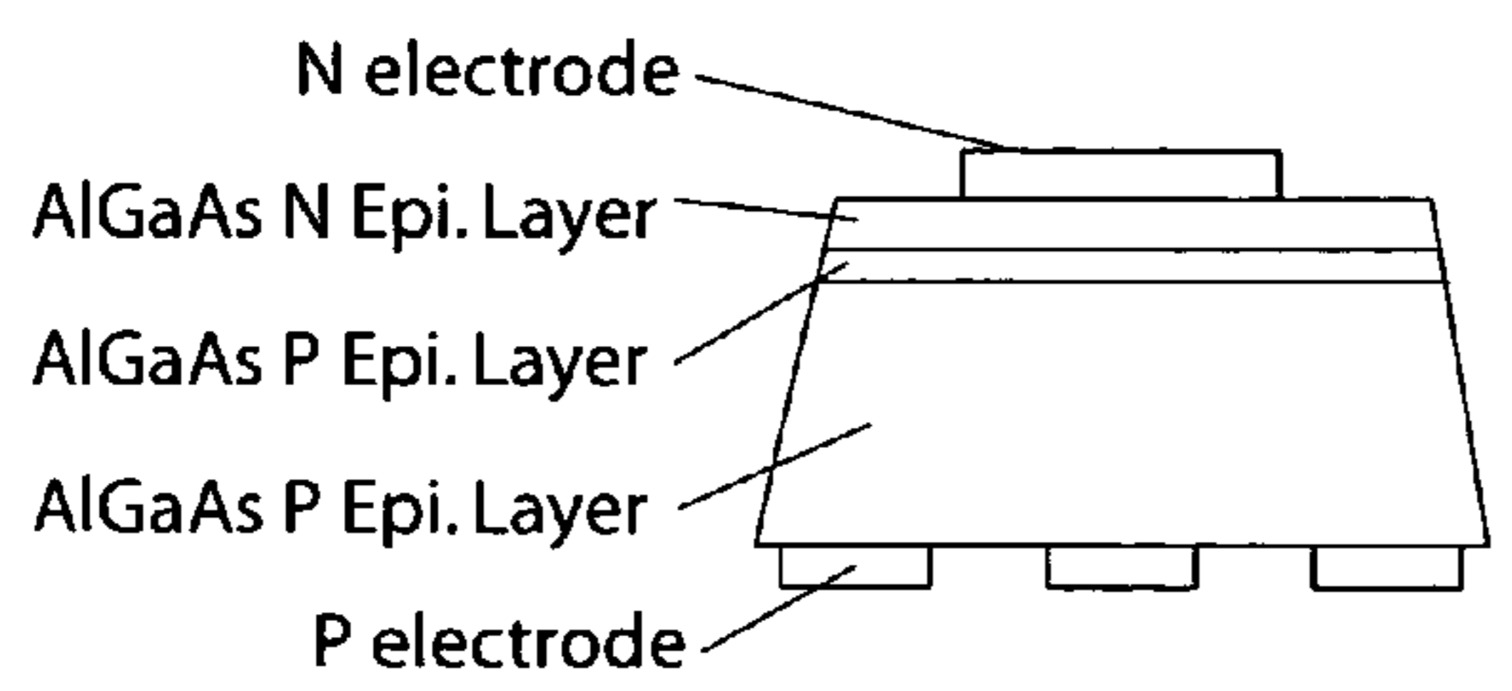
Figure 66 Prior Art
