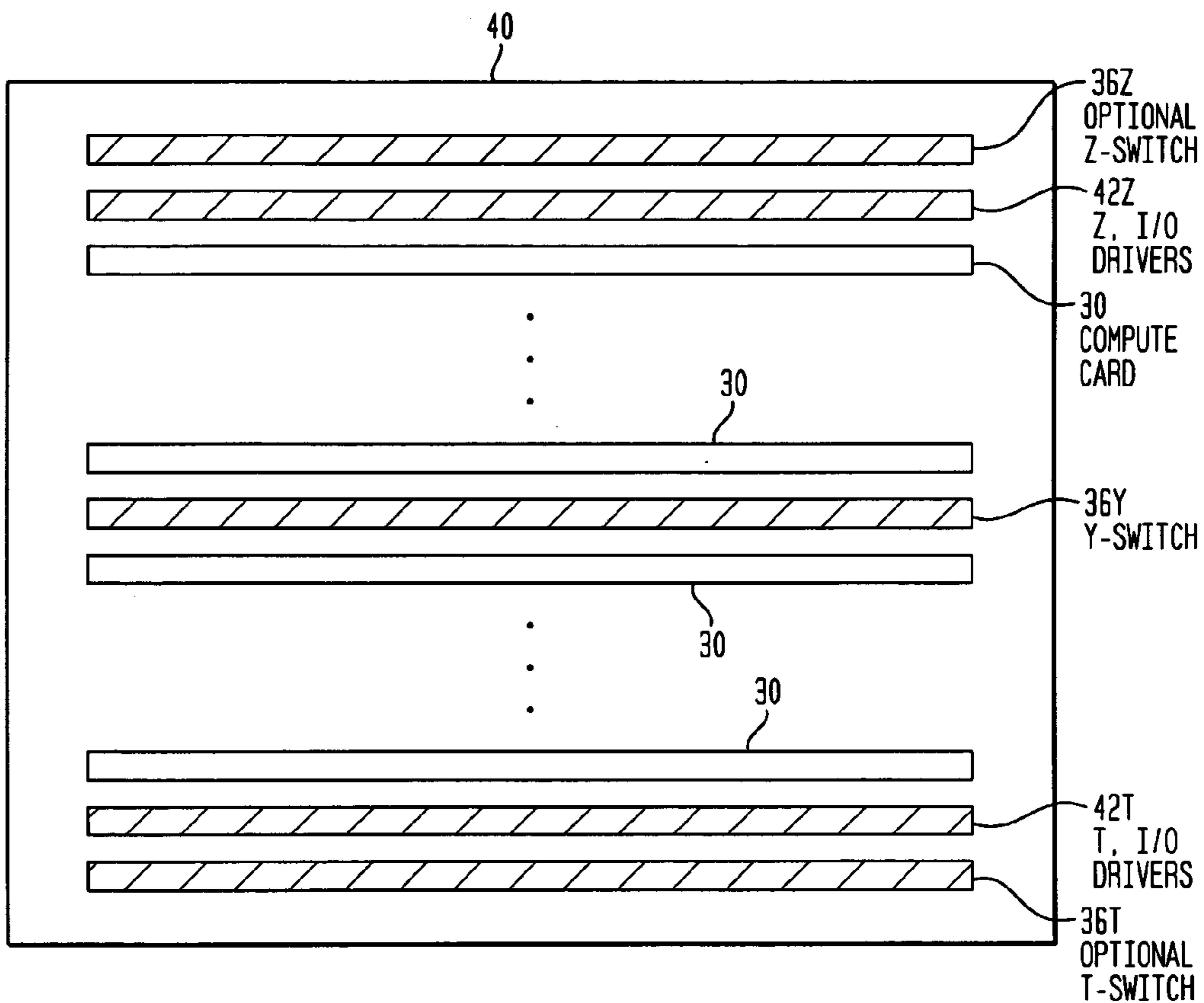
FIG. 4 COMPUTE MIDPLANE
