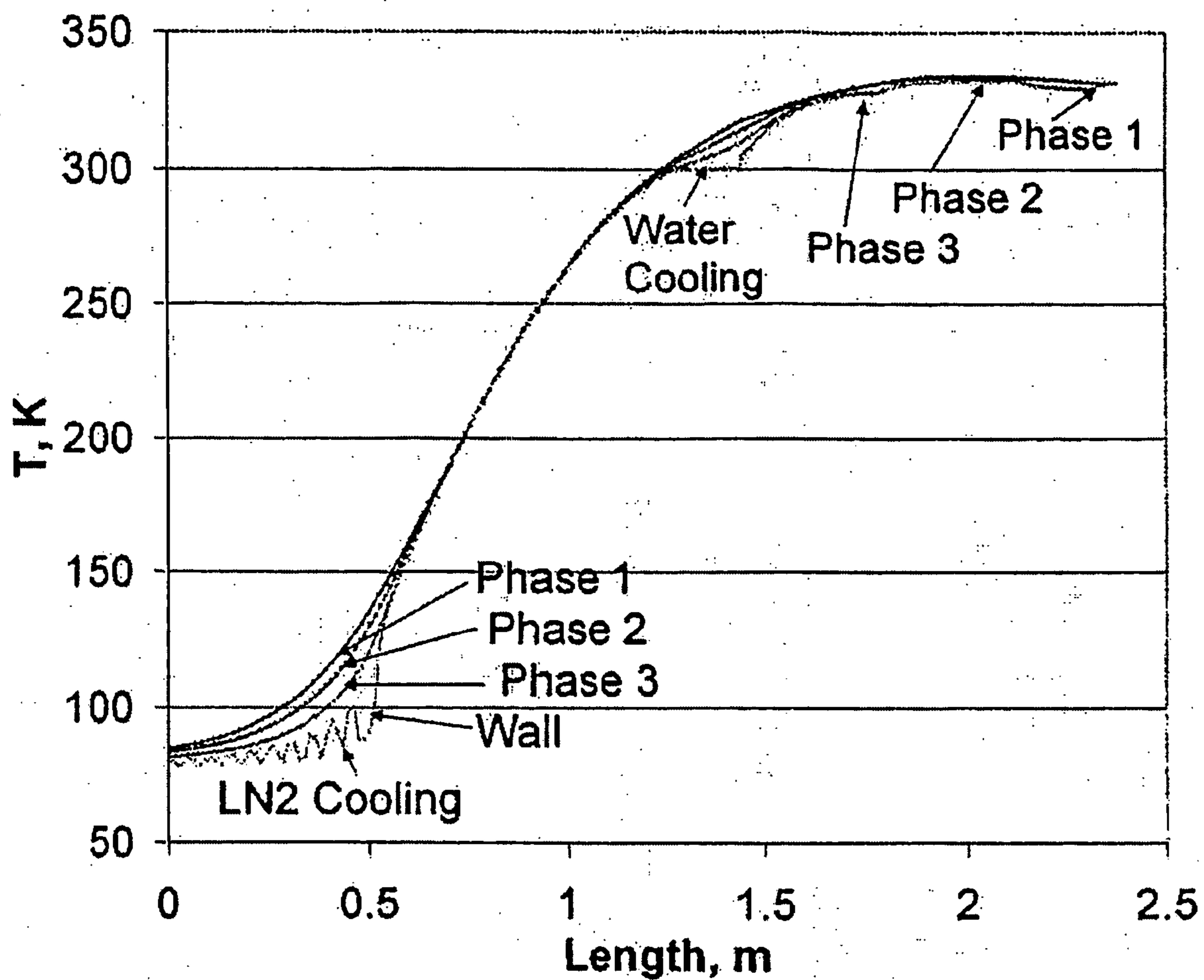
Figure 5. ANSYS predicted temperature profiles in the termination.
