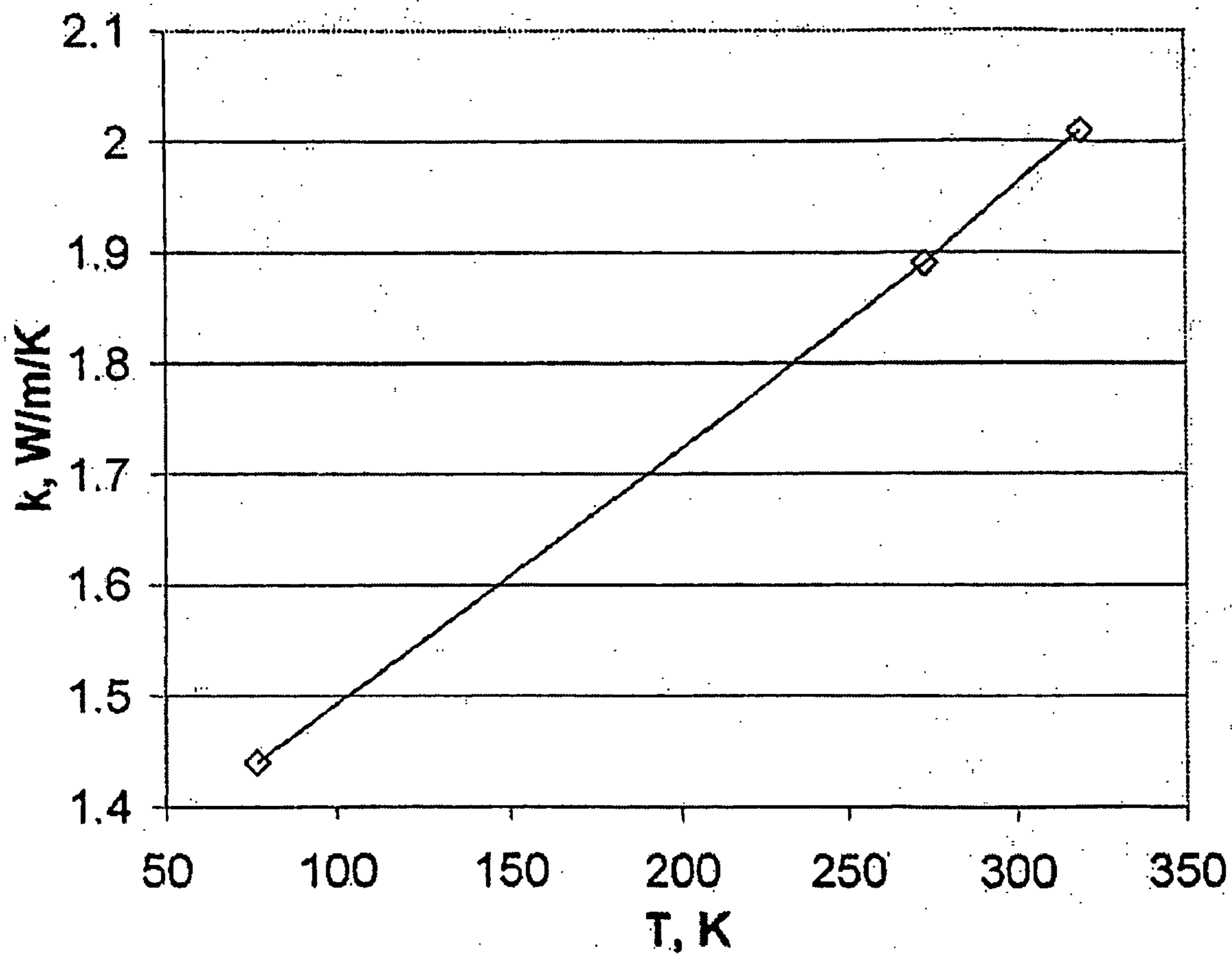
Figure 4. Thermal conductivity of termination dielectric material.
