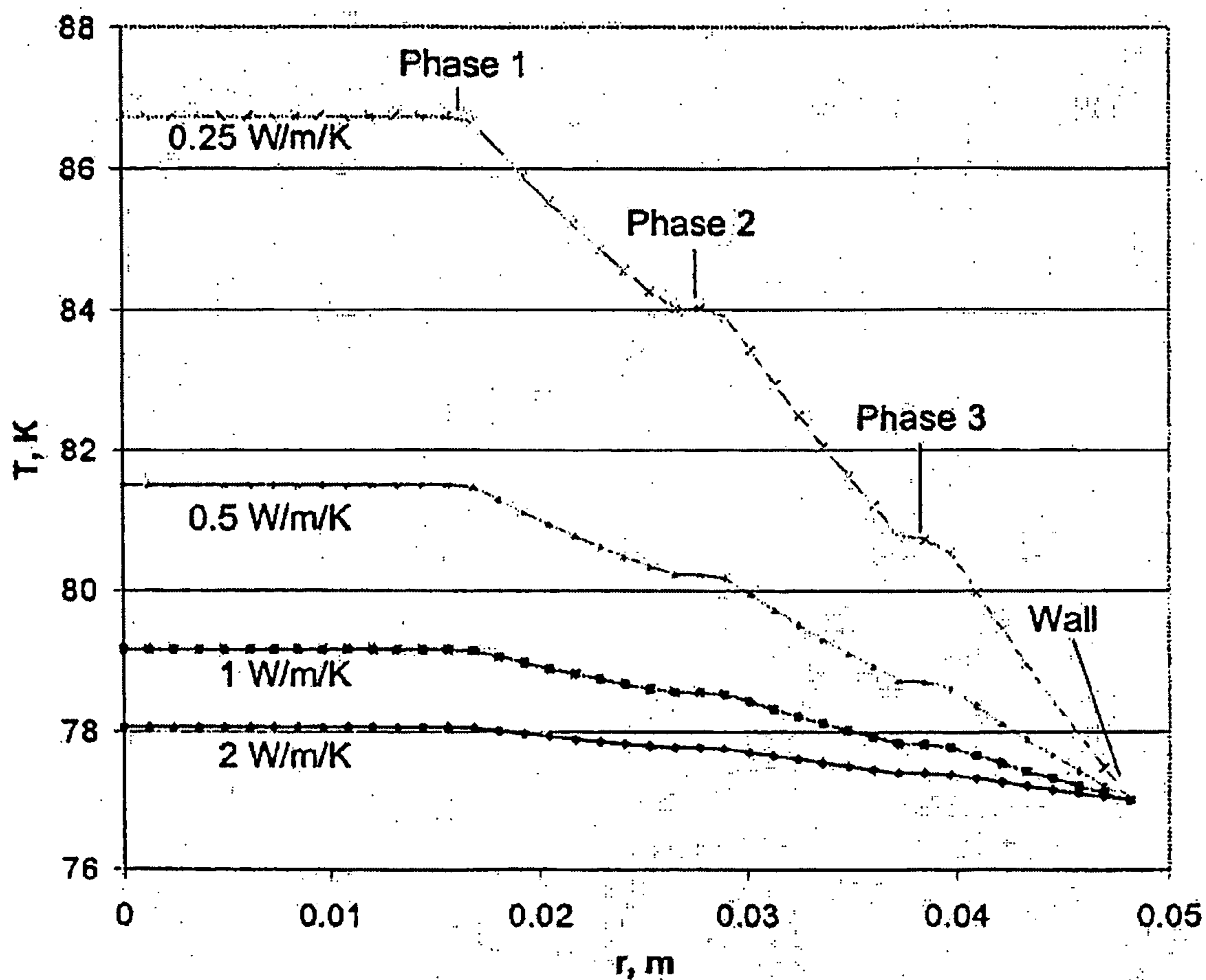
Fig. 3. Radial temperature profile of the tri-axial termination.
