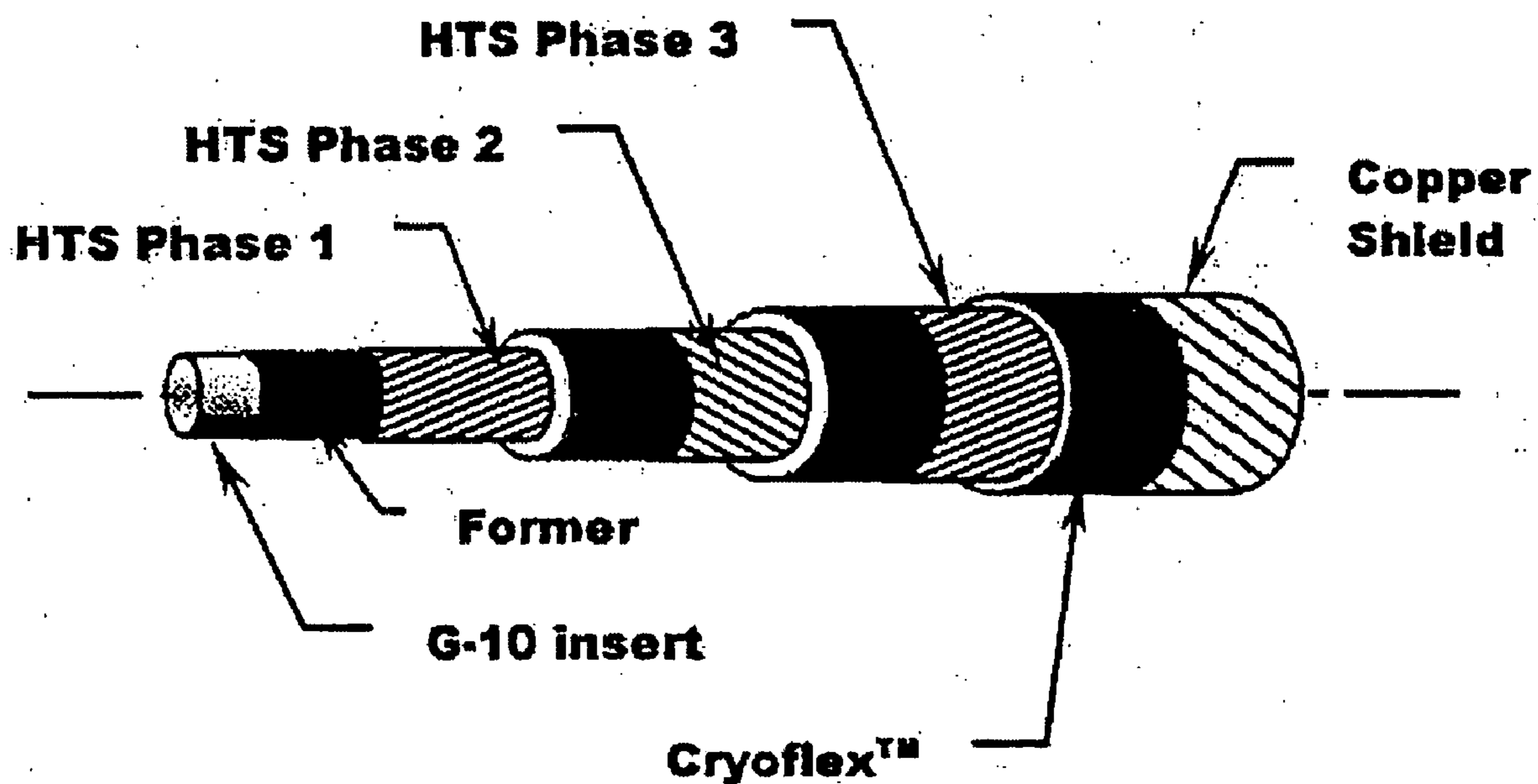
Fig. 2. Schematic of the tri-axial cable.
