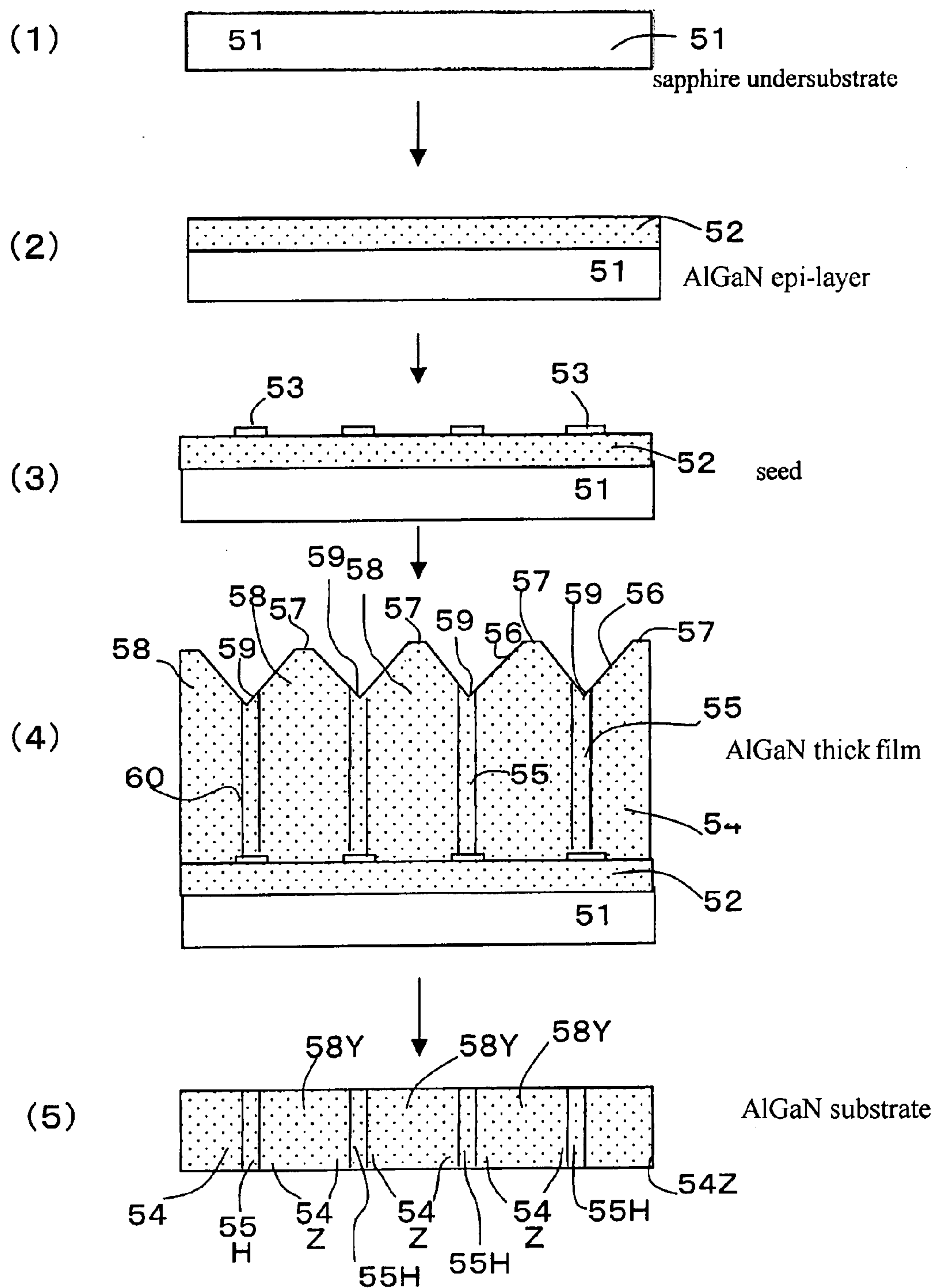
Embodiment 1 Processes of producing an AlGa N substrate
