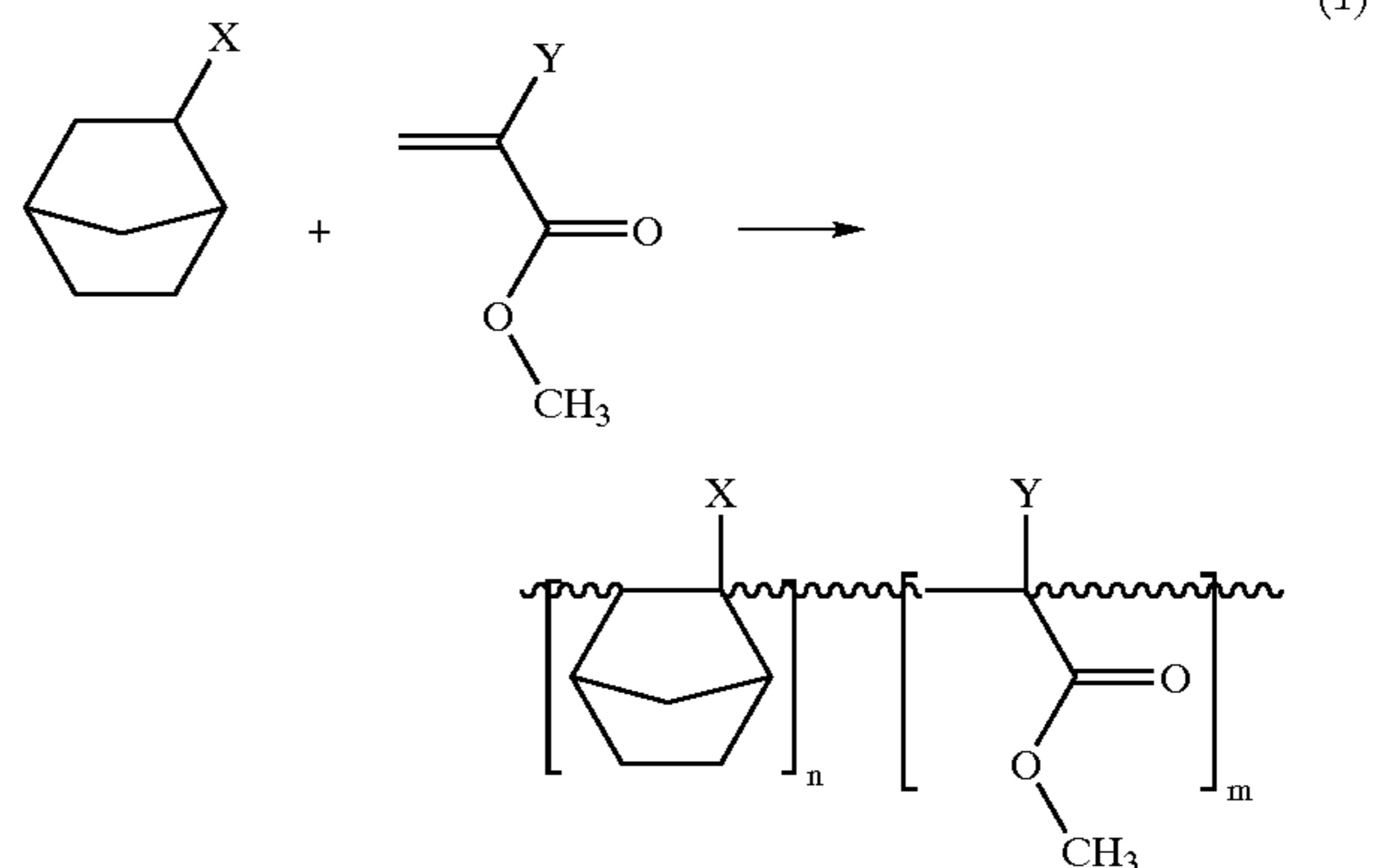
Scheme 1
