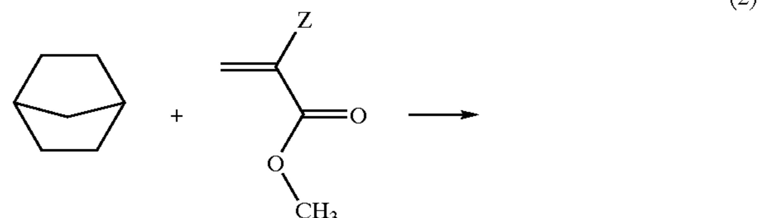
Scheme 2
