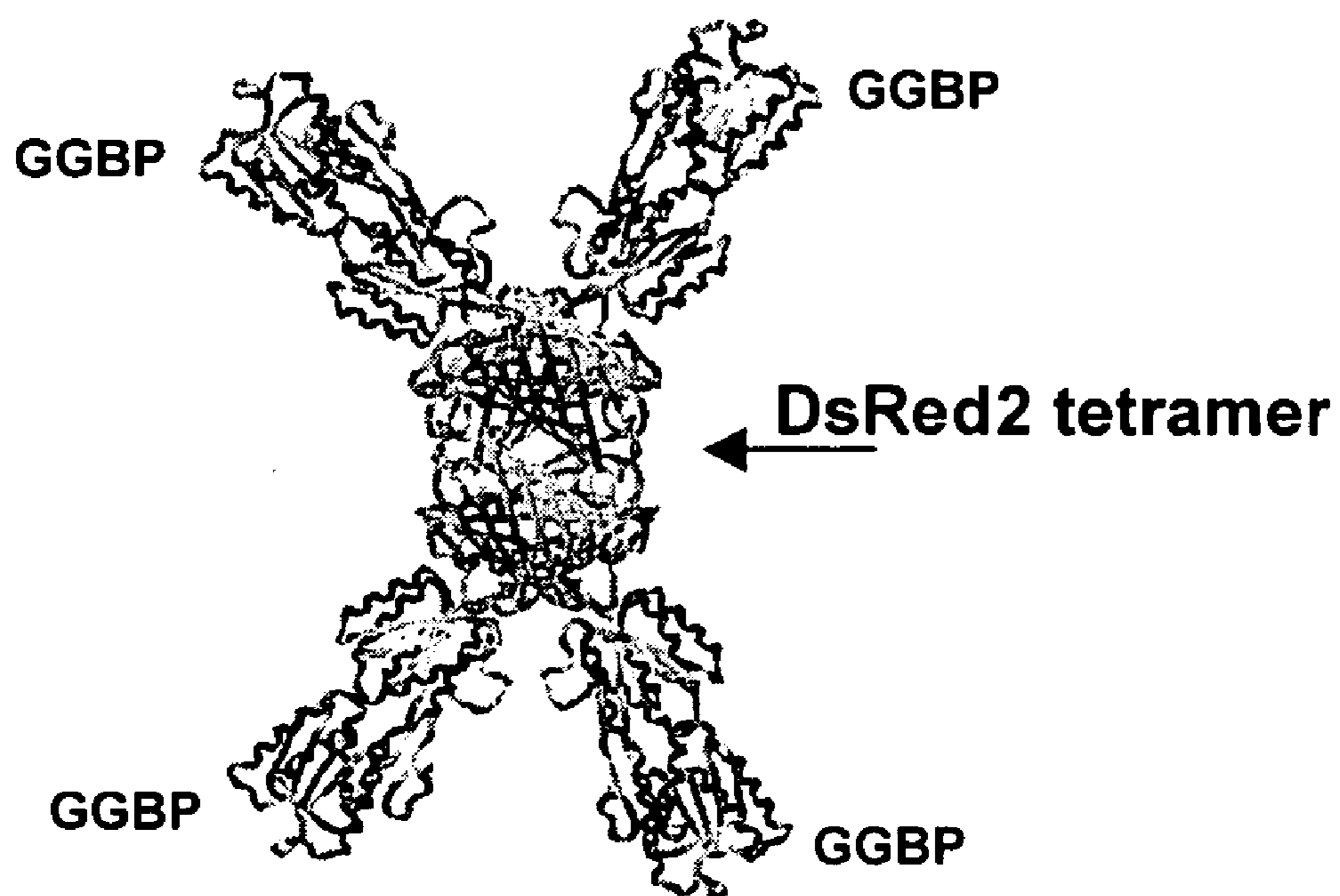
DsRed2(C119A)GGBP tetrameric structure
