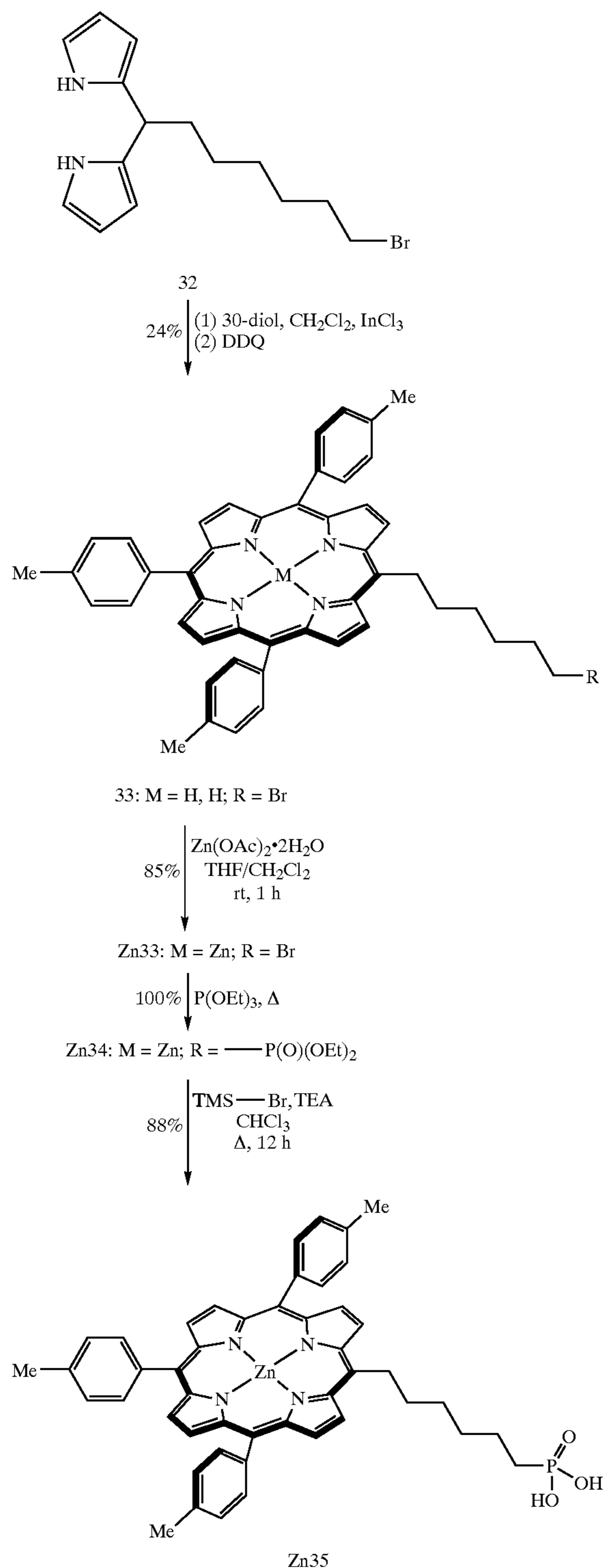
Scheme 13
