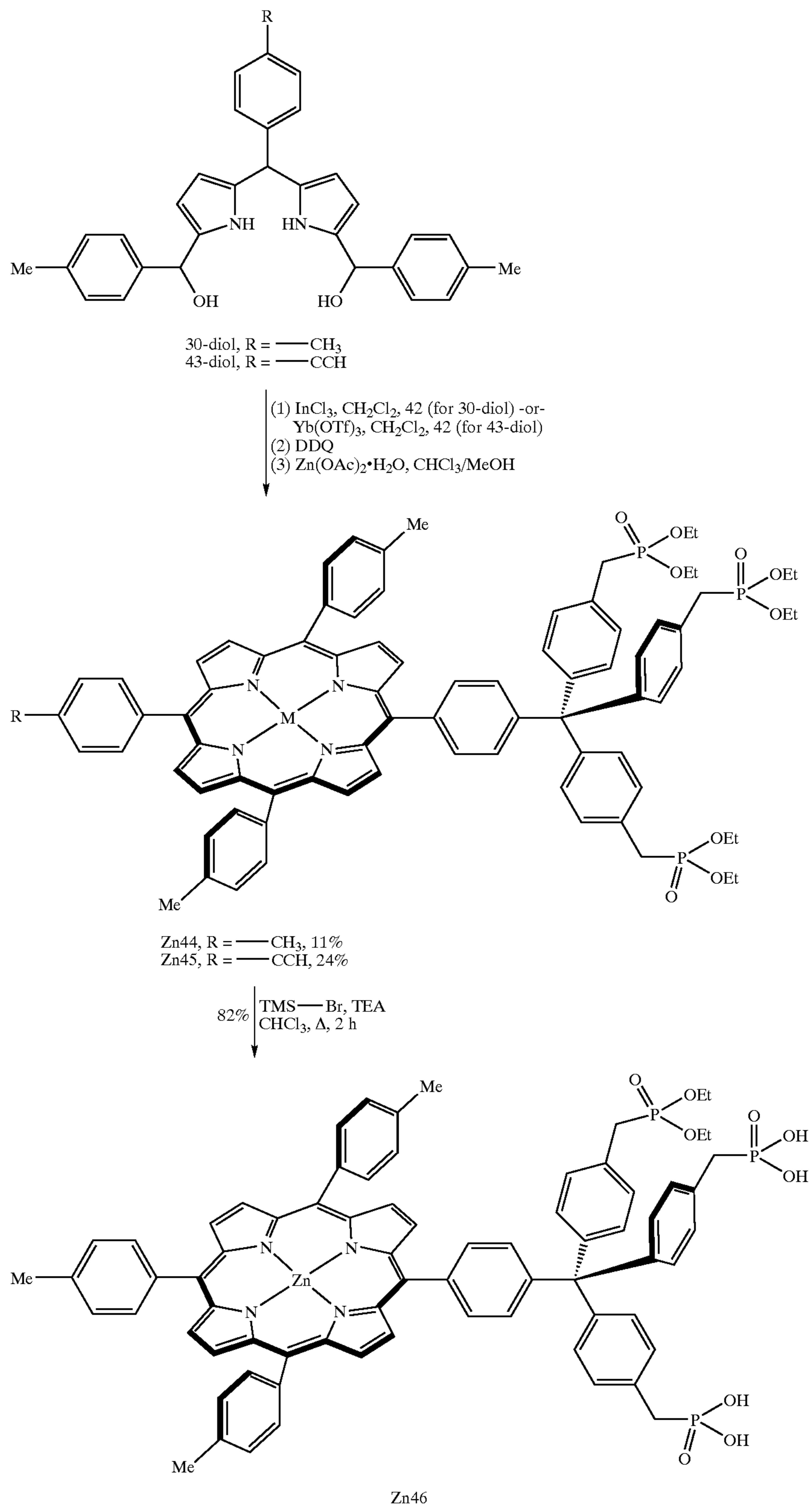
Scheme 16
