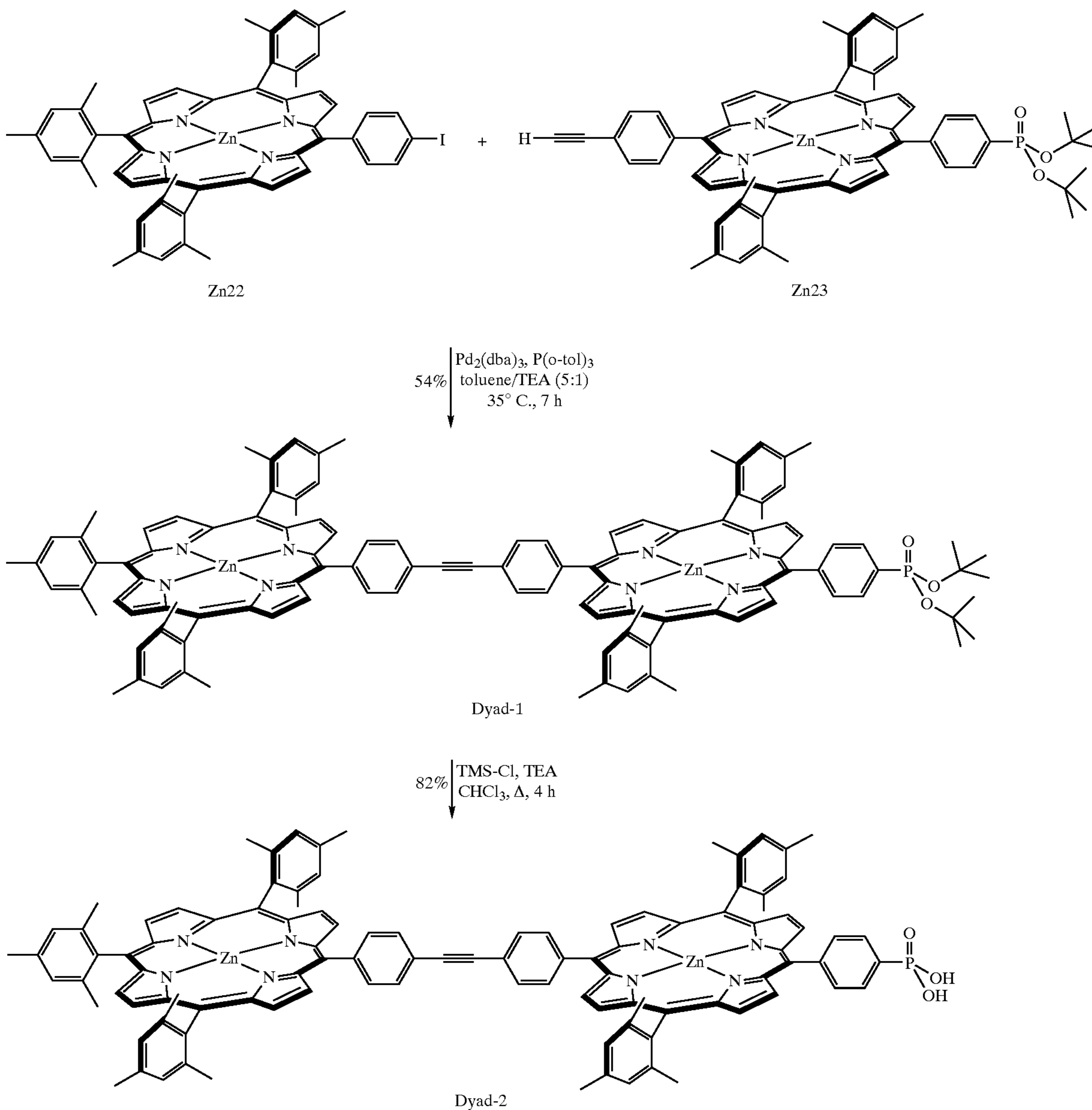
Scheme 9
