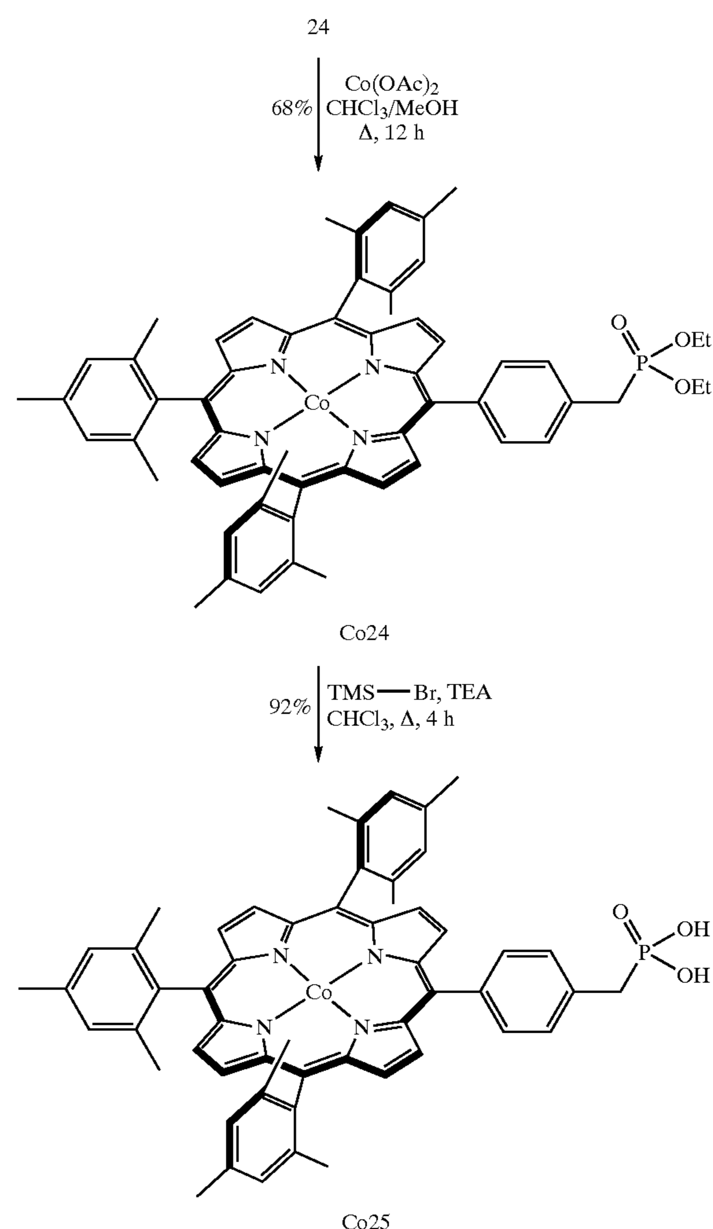
Scheme 14
