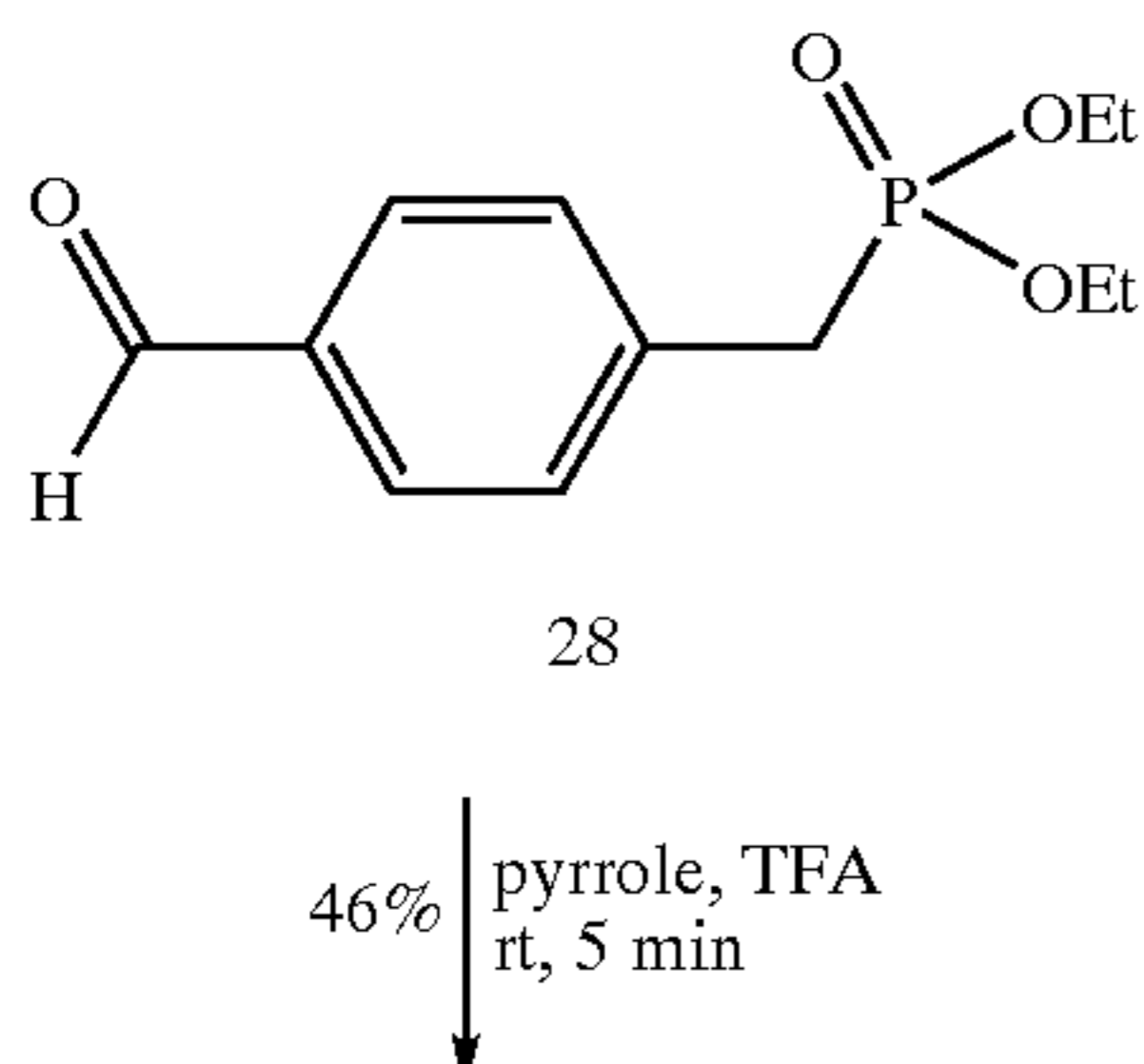
Scheme 12
