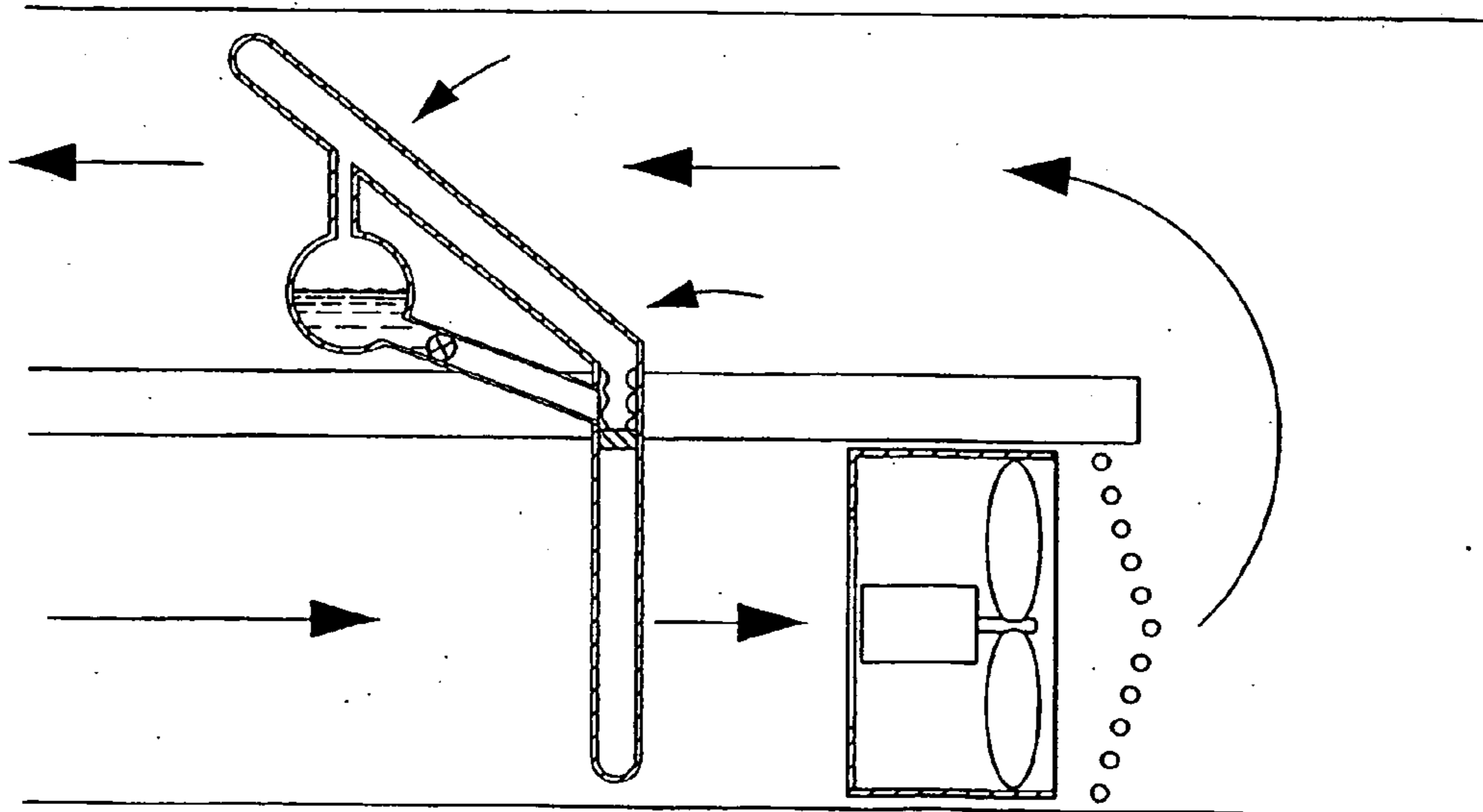
Fig. 4 (PRIOR ART)
