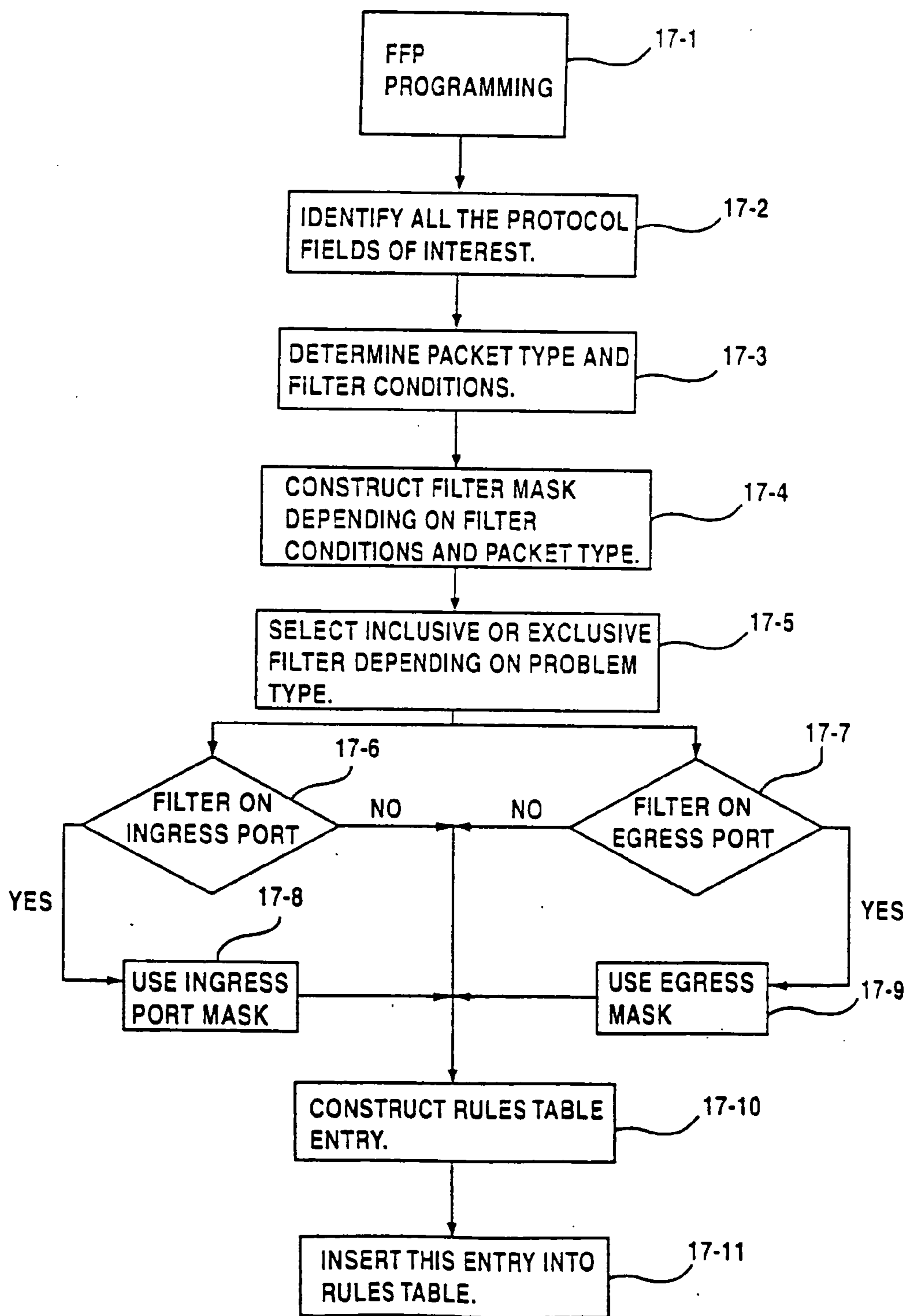
FFP PROGRAMMING FLOW CHART
