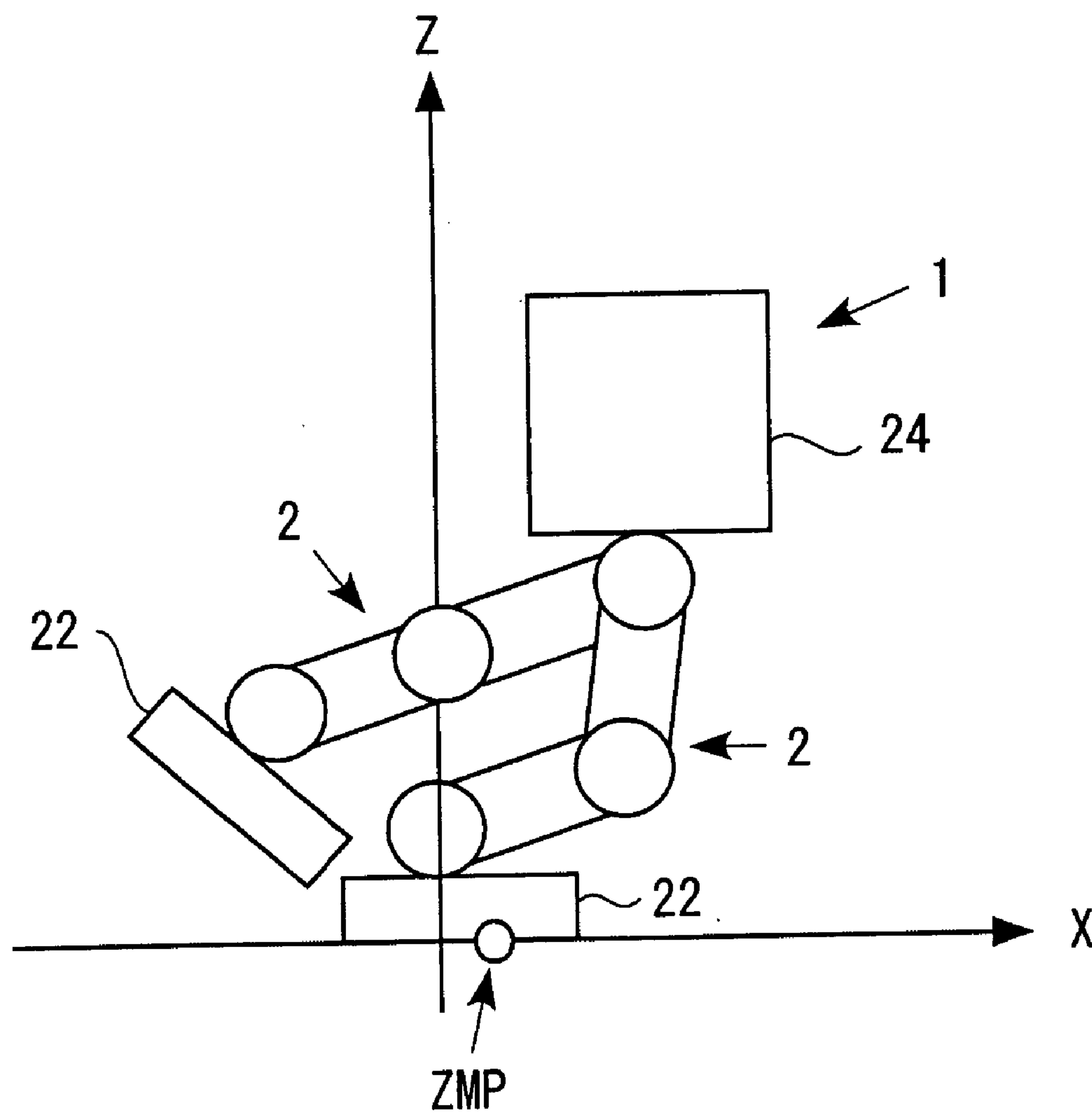
FIG.14 ( DIVERGENCE STATE OF BODY POSITION )
