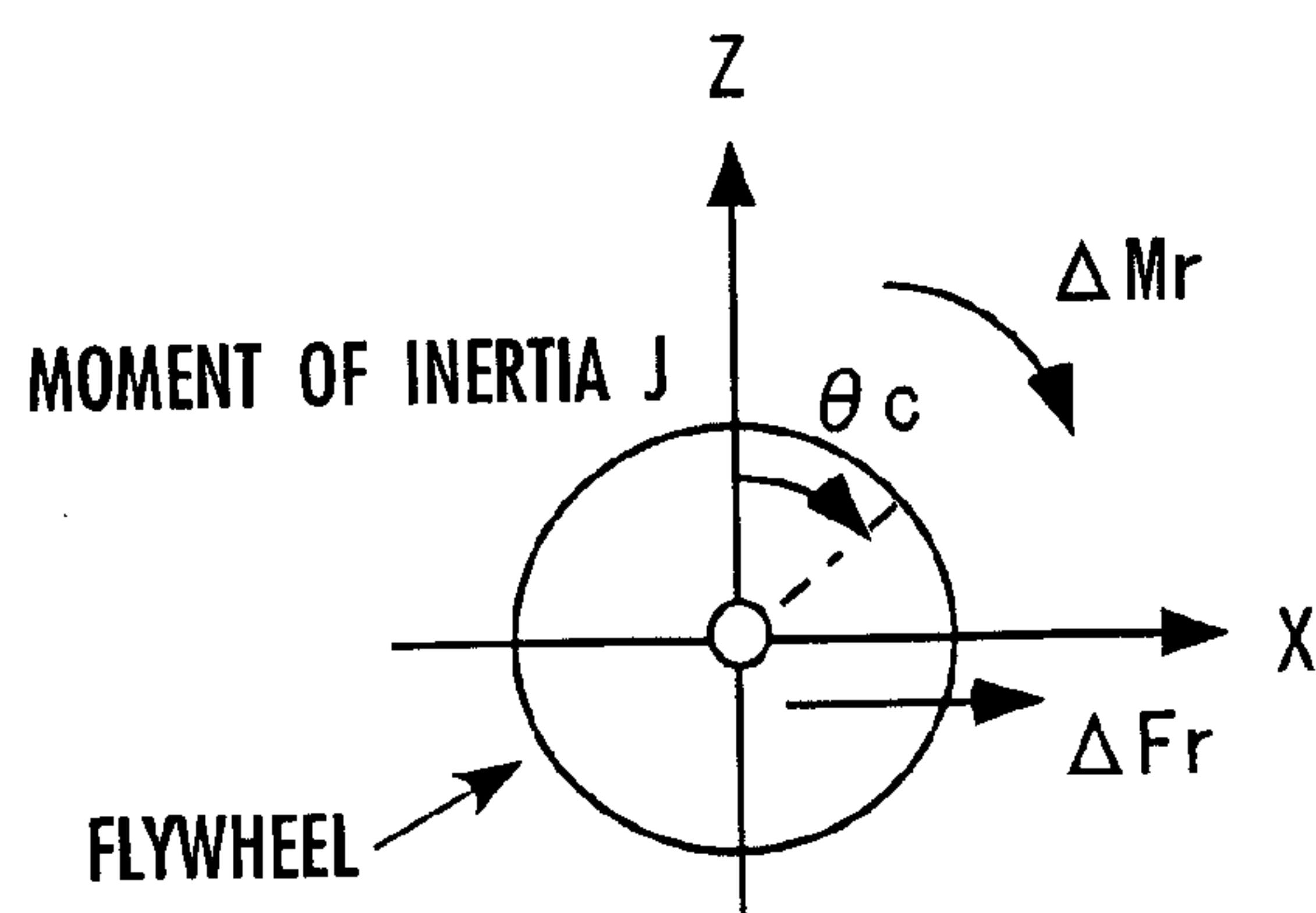
FIG.44 ( PERTURBATION MODEL FOR CORRECTING BODY POSTURE ANGLES )
