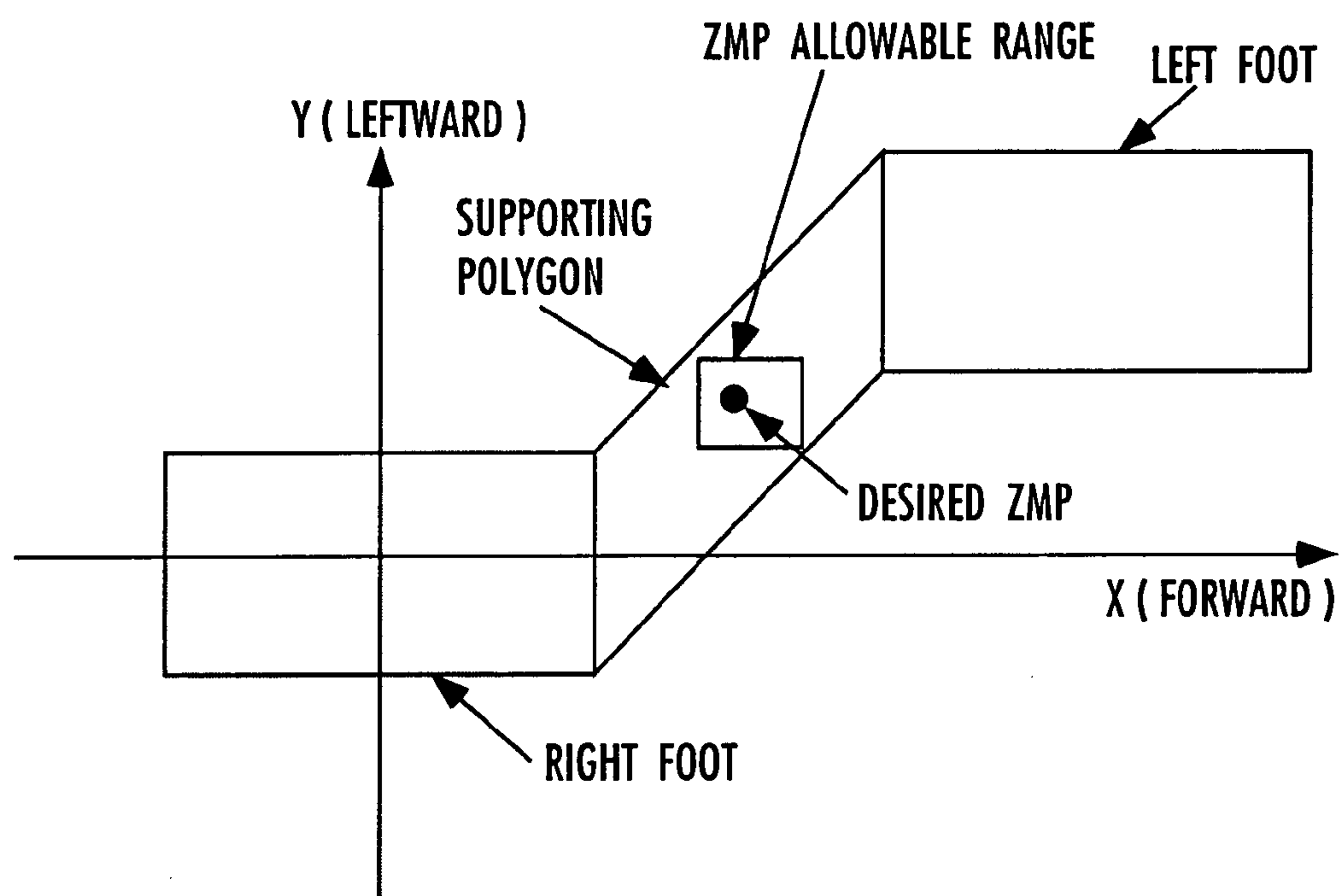
FIG.45 ( SUPPORTING POLYGON AND ZMP ALLOWABLE RANGE )
