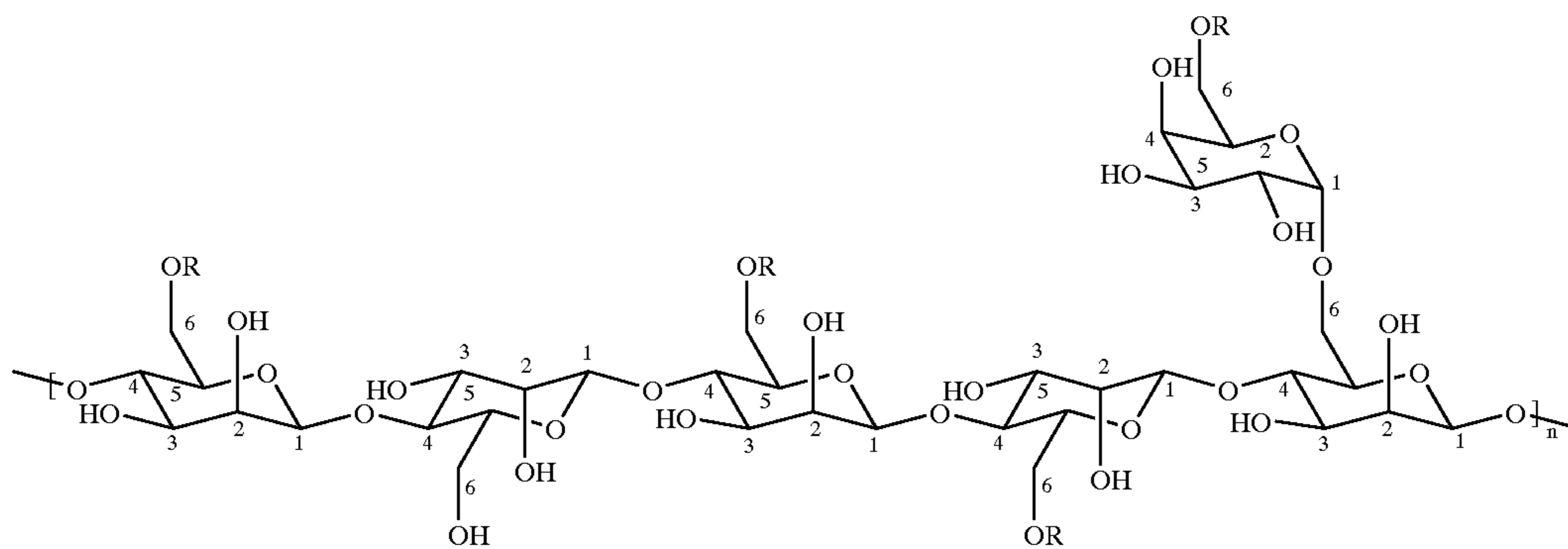
polygalactomannose backbone
