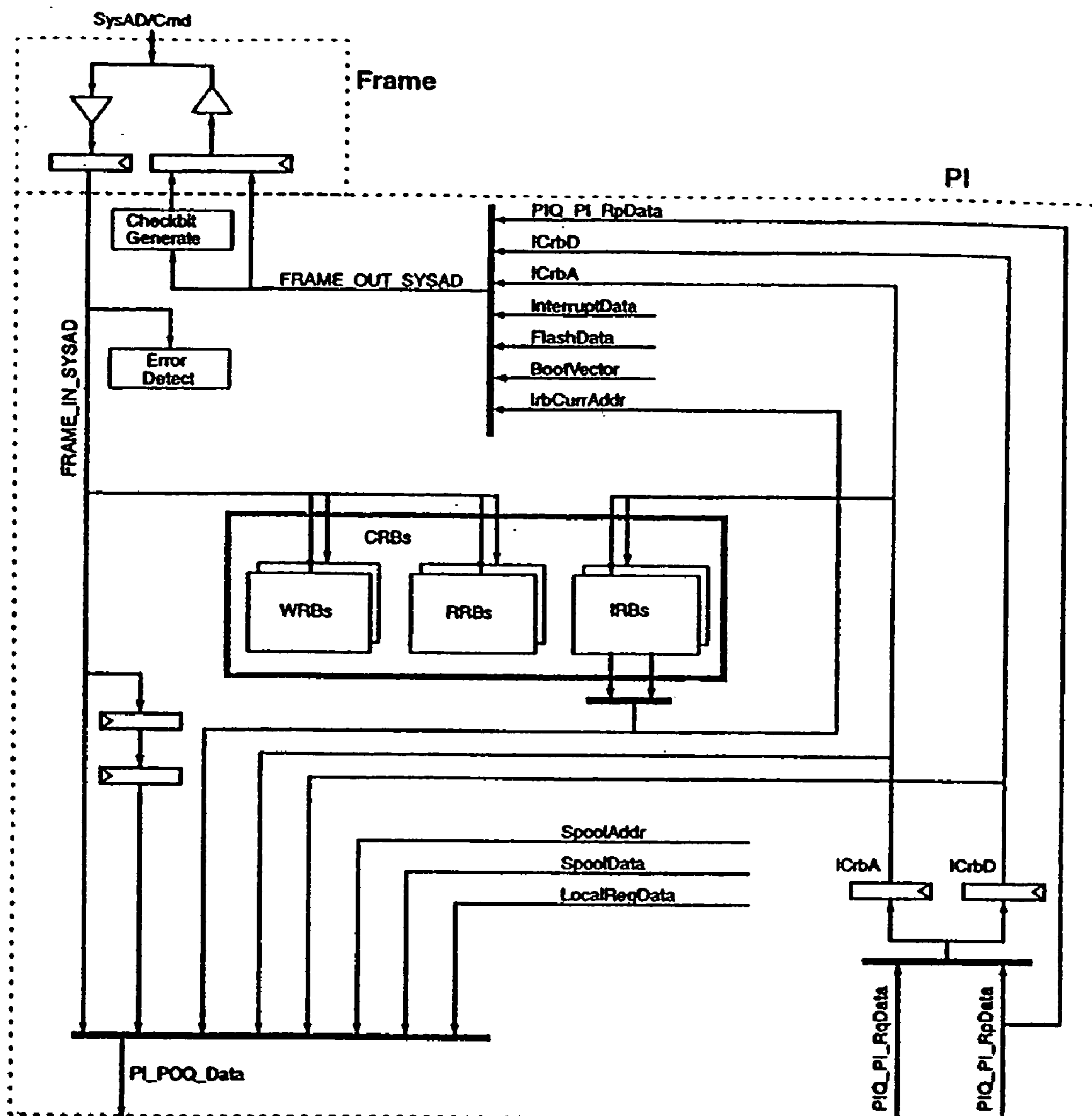
PI Address/Data Path Diagram
