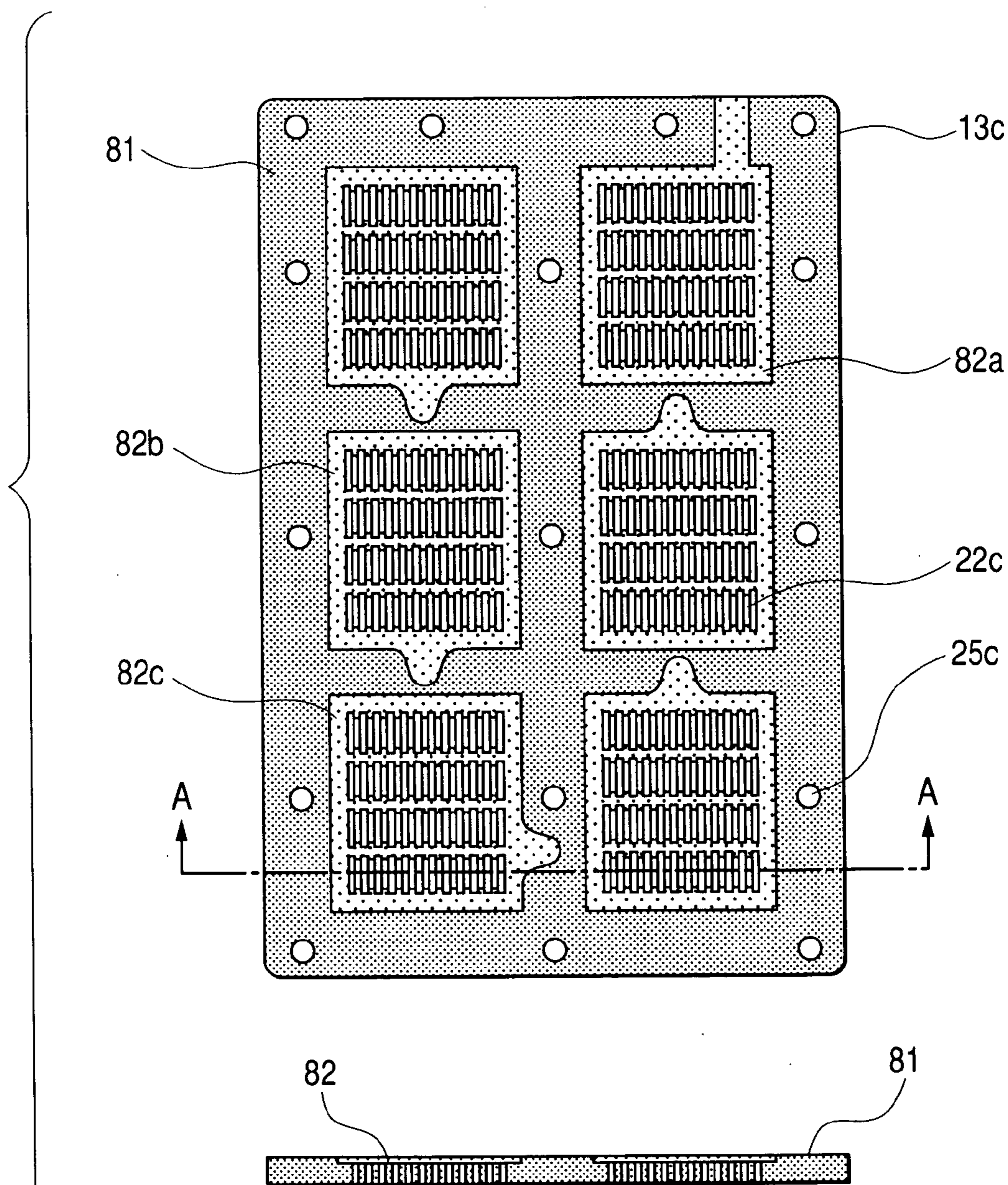
CROSS-SECTIONAL VIEW TAKEN ALONG A-A LINE
