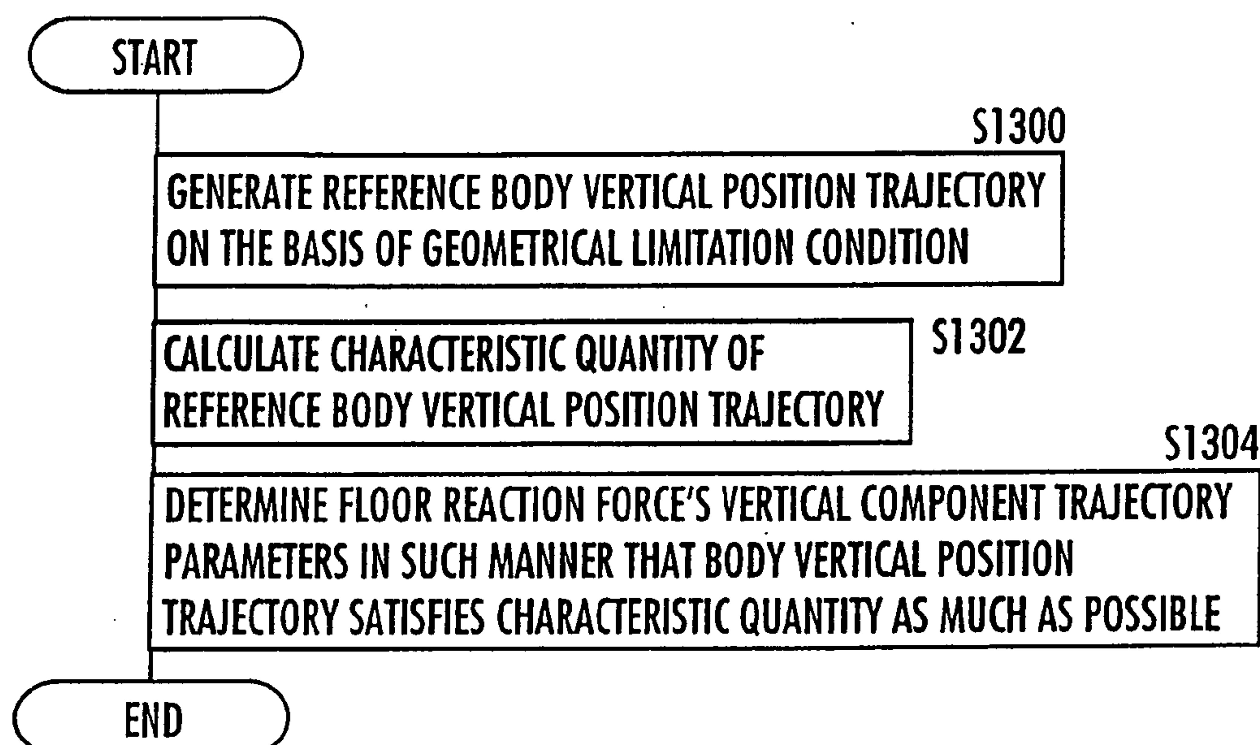
FIG.43 ( DETERMINATION PROCESS a FOR FLOOR REACTION FORCE'S VERTICAL COMPONENT TRAJECTORY PARAMETERS FOR WALKING)
