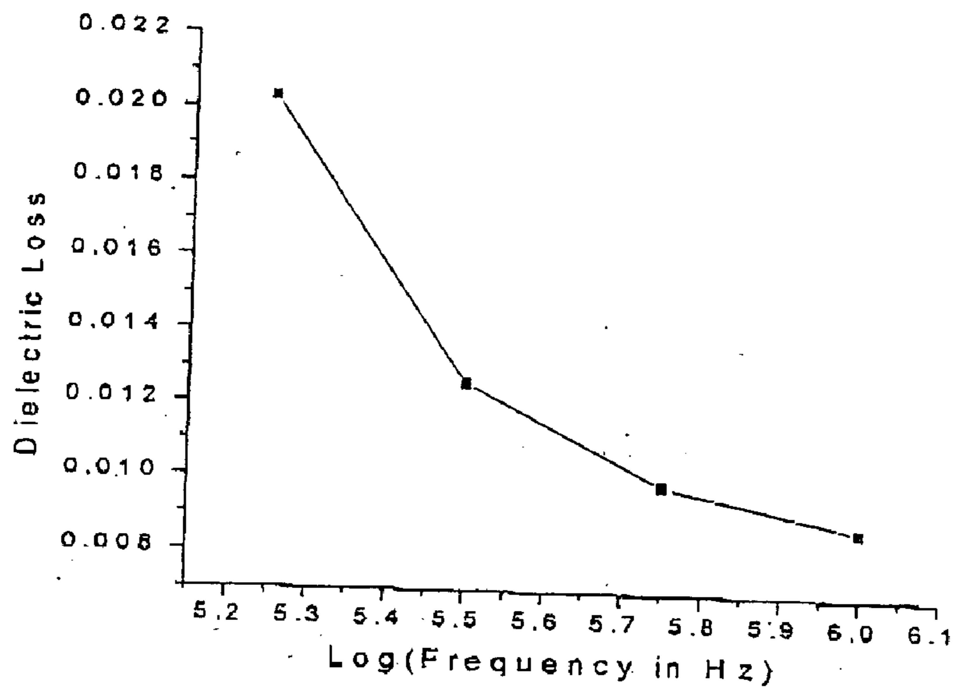
Fig-3: Variation of Dielectric loss with Log (frequency) of sintered Mg_2EuSnO_{5.5}
