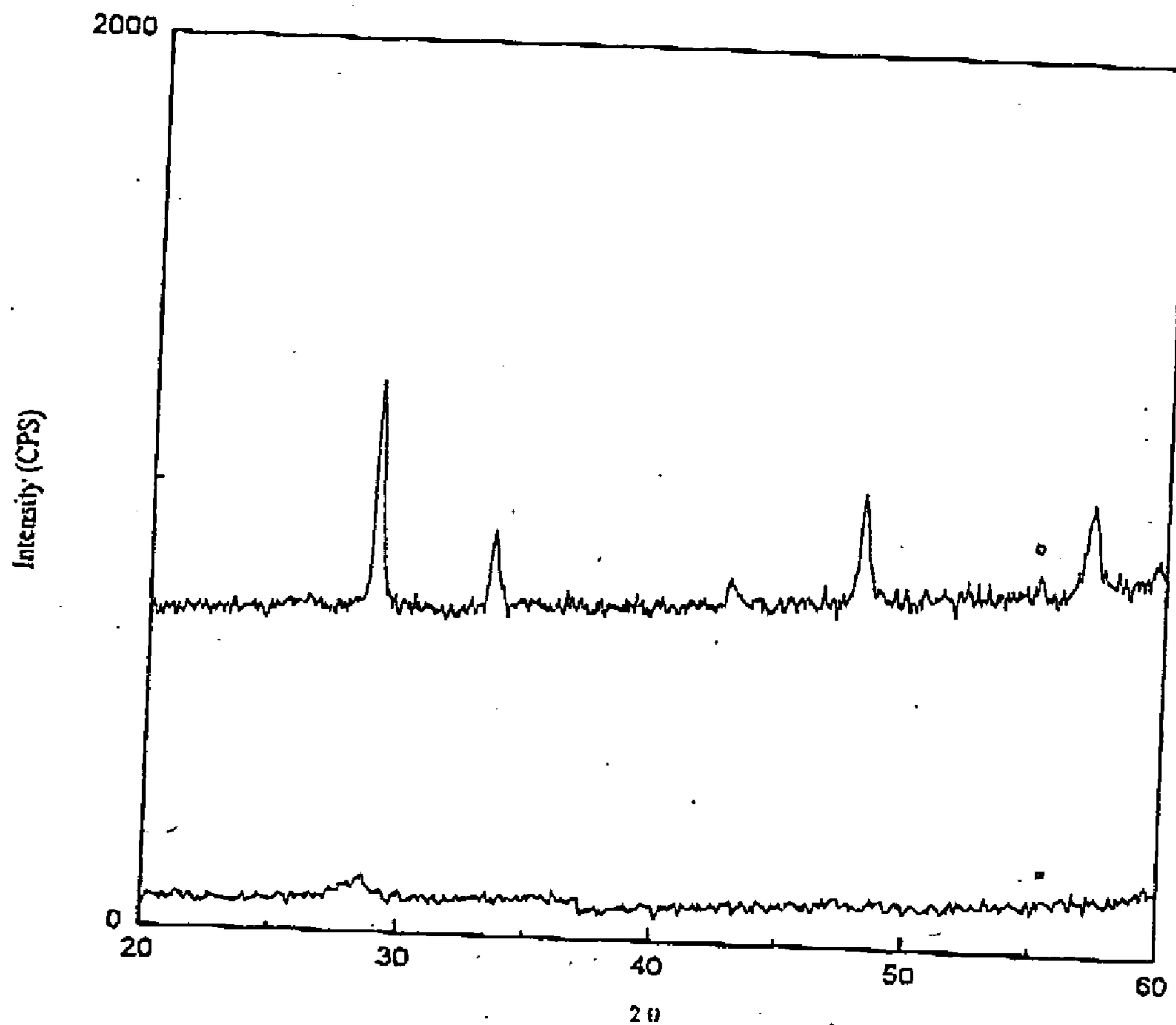
Fig-10: XRD of Mg_2PrZr_{5.5} (a) Obtained by heating the precursor at 500^{\circ}C (b) Obtained by heating the powder at 1000^{\circ}C
