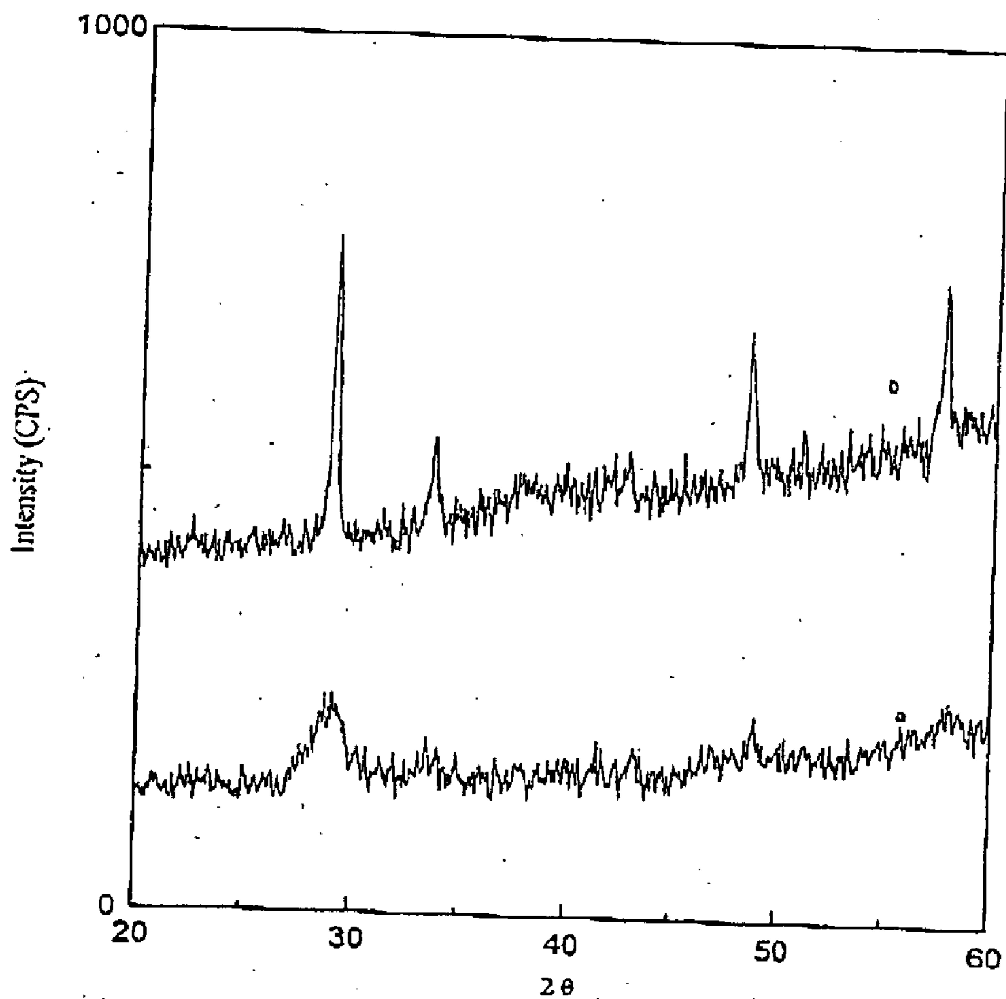
Fig - 7: XRD of Mg_2SmZrO_{5.5} (a) Obtained by heating the precursor at 500^{\circ}C (b) Obtained by heating the powder at 1000^{\circ}C
