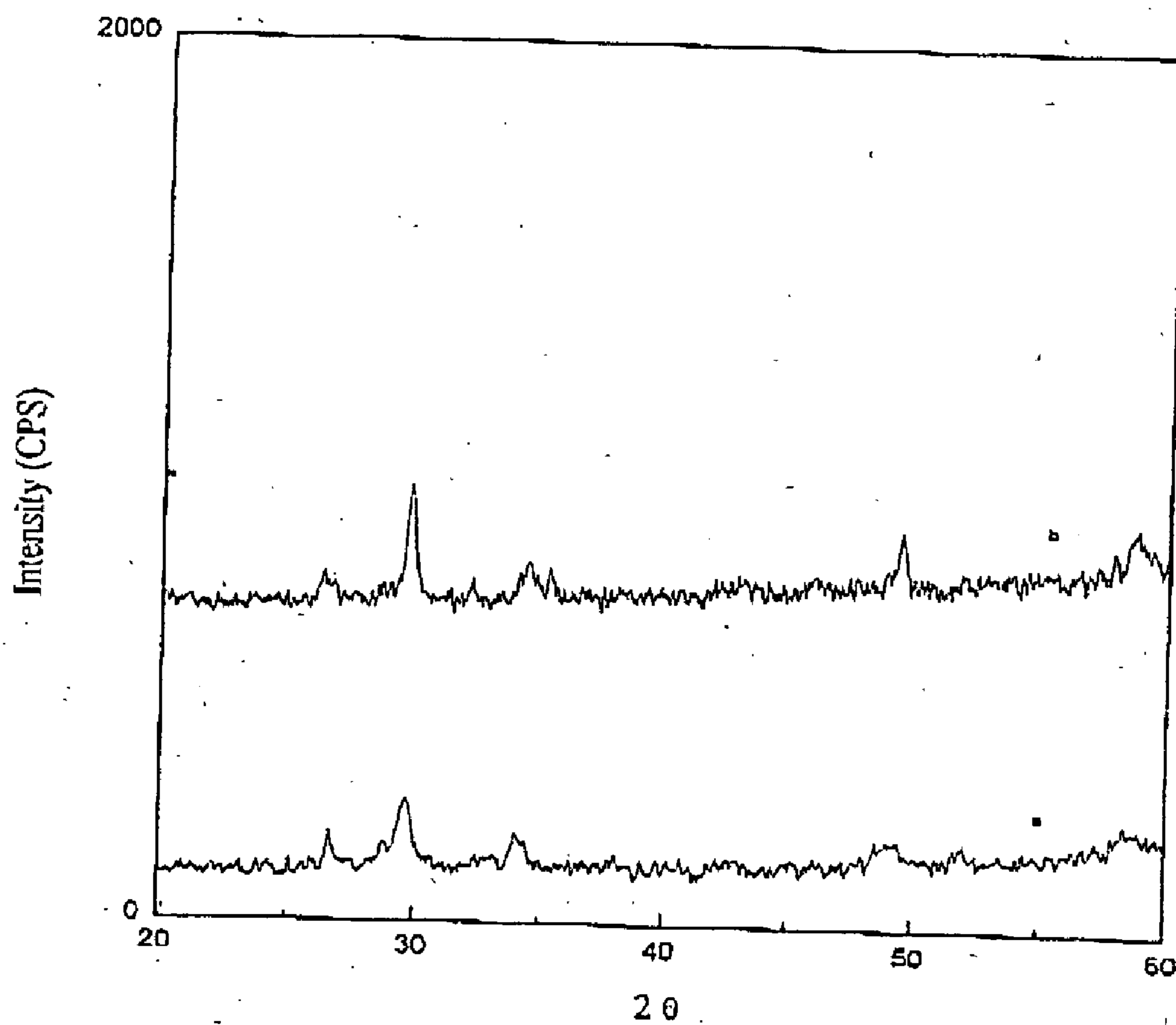
Fig-4: XRD of Mg_2GdSnO_{5.5} (a) Obtained by heating the precursor at 500^{\circ}C (b) Obtained by heating the powder at 1000^{\circ}C
