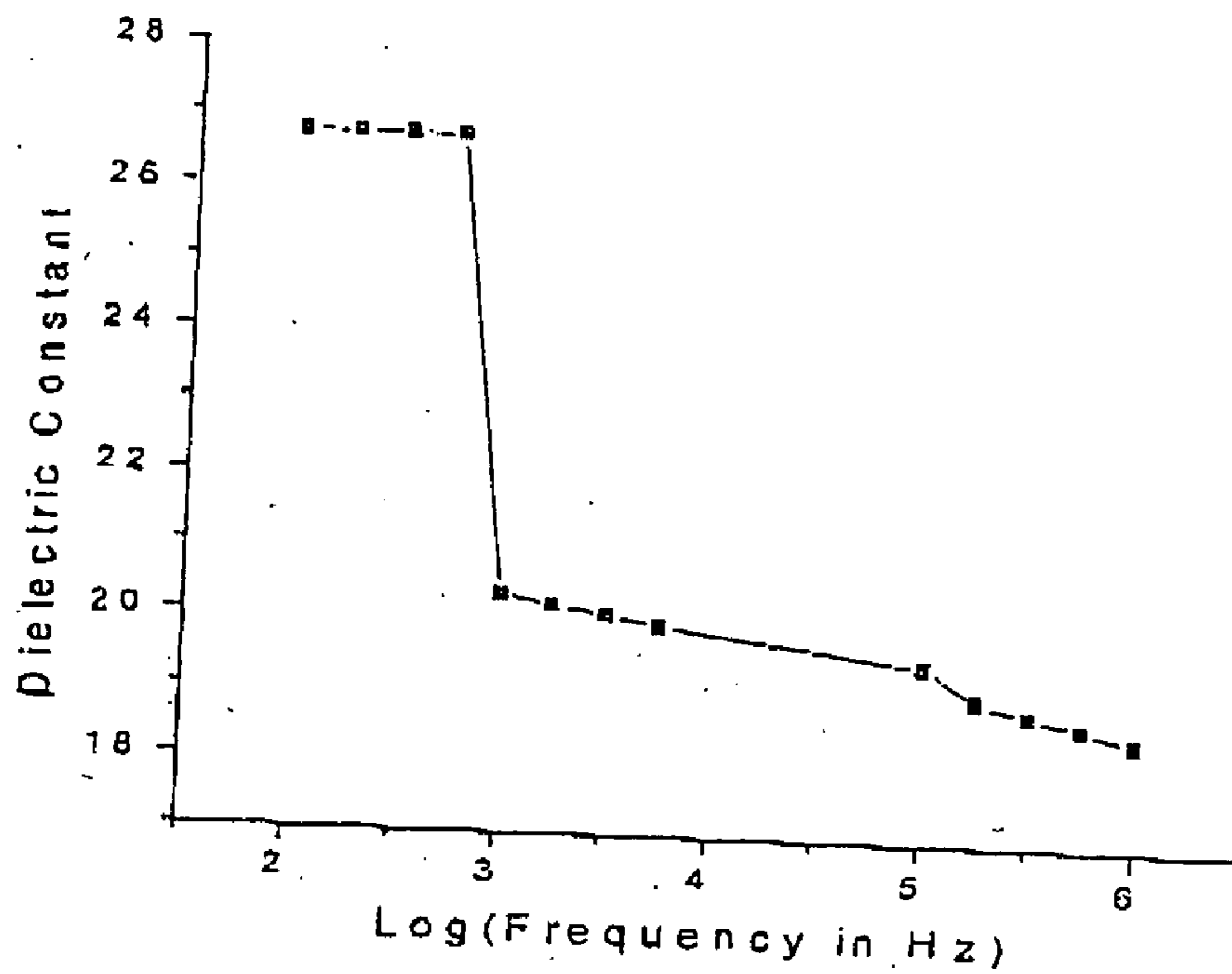
Fig-8: Variation of Dielectric constant with Log(Frequency) of sintered Mg_2SmZrO_{5.5}
