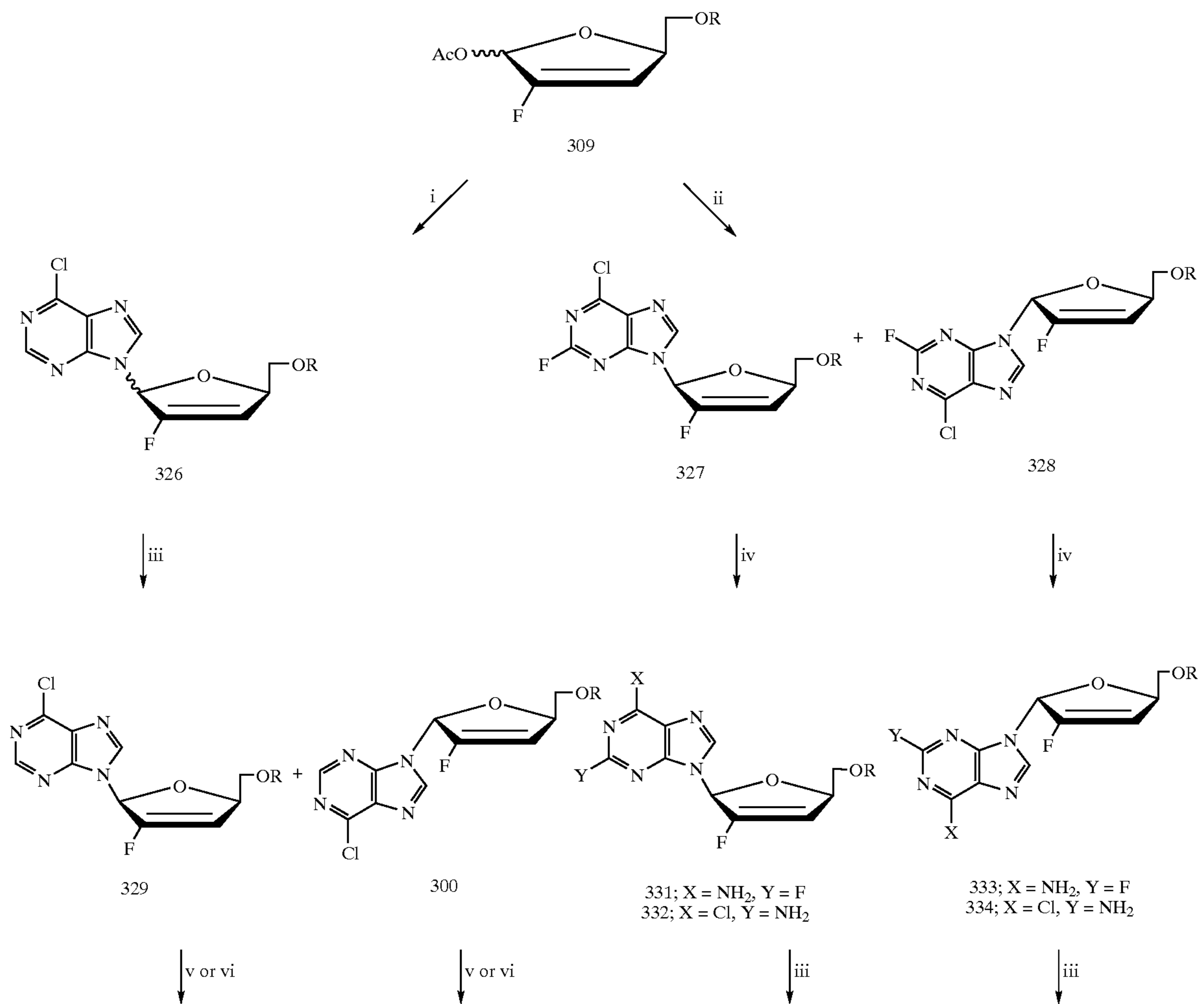
Scheme 9
