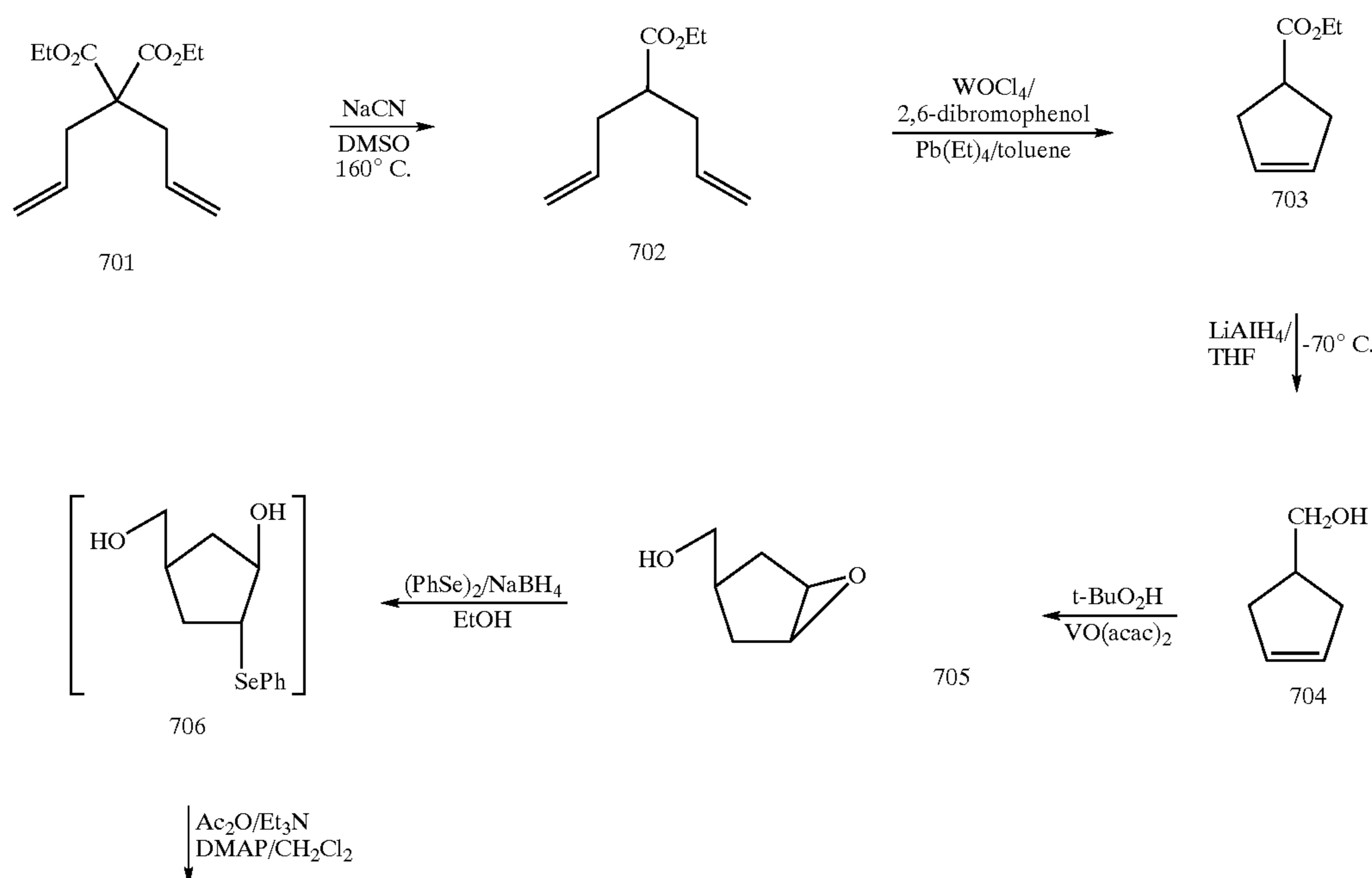
Scheme 11
