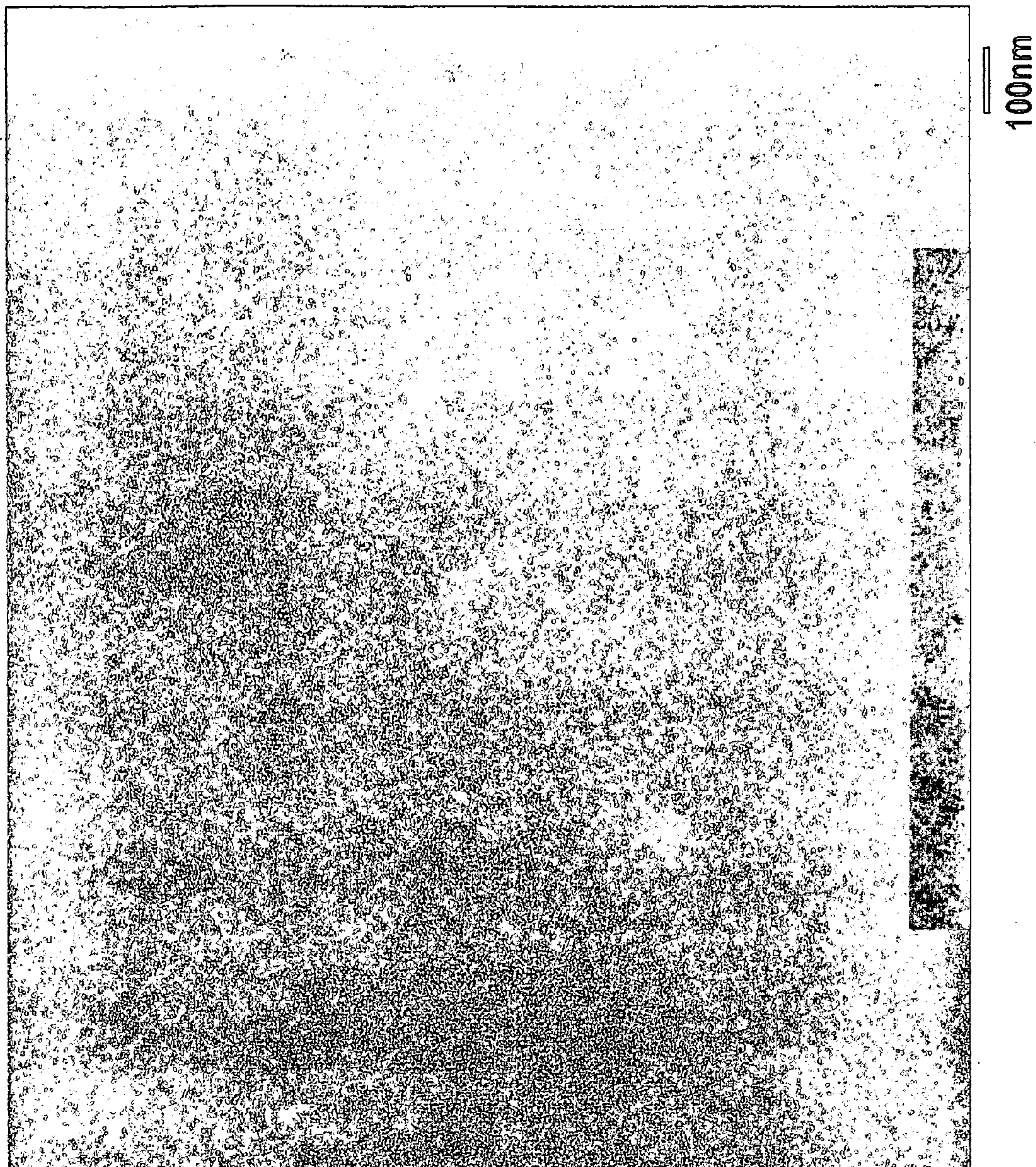
Fig. 1. TEM image of the graft polymer (PMMA-g-EPR) obtained in Example 11.
