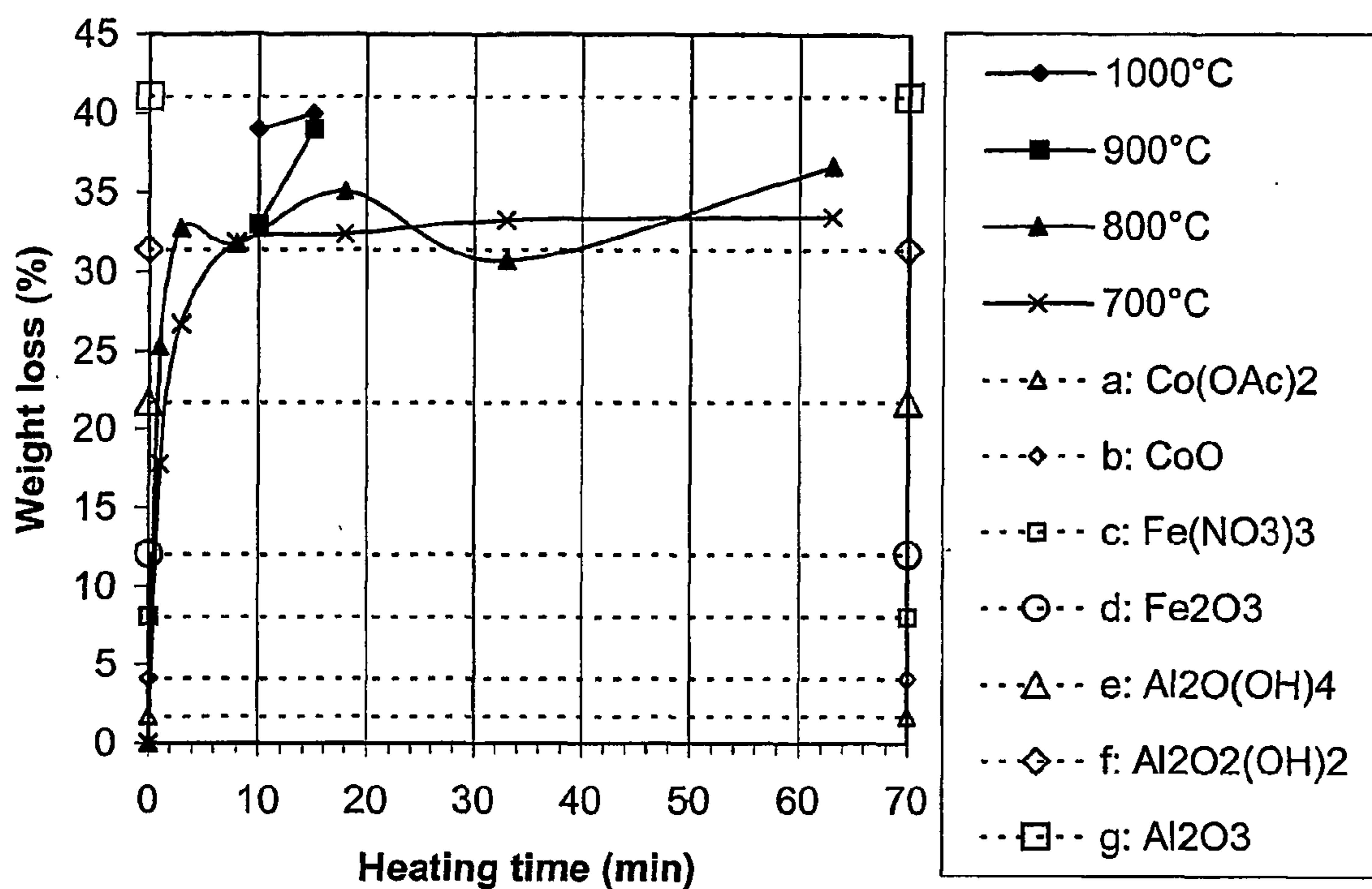
FIG. 1: SCA2/Nitrogen
