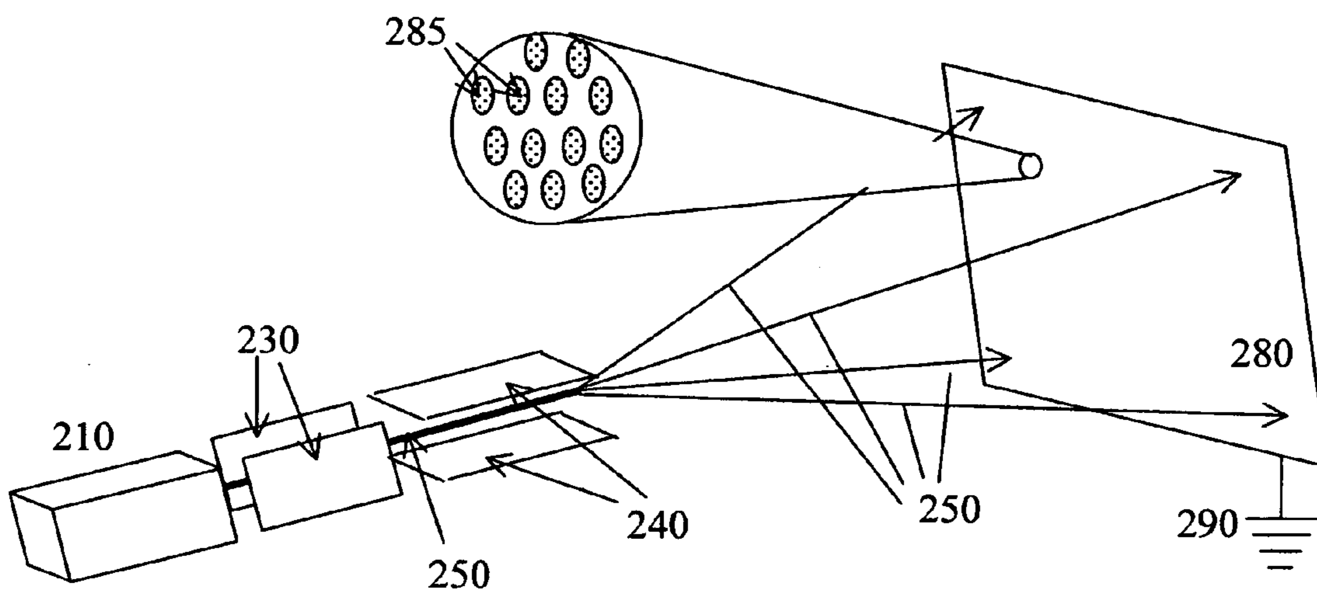
FIG. 2 (PRIOR ART)
