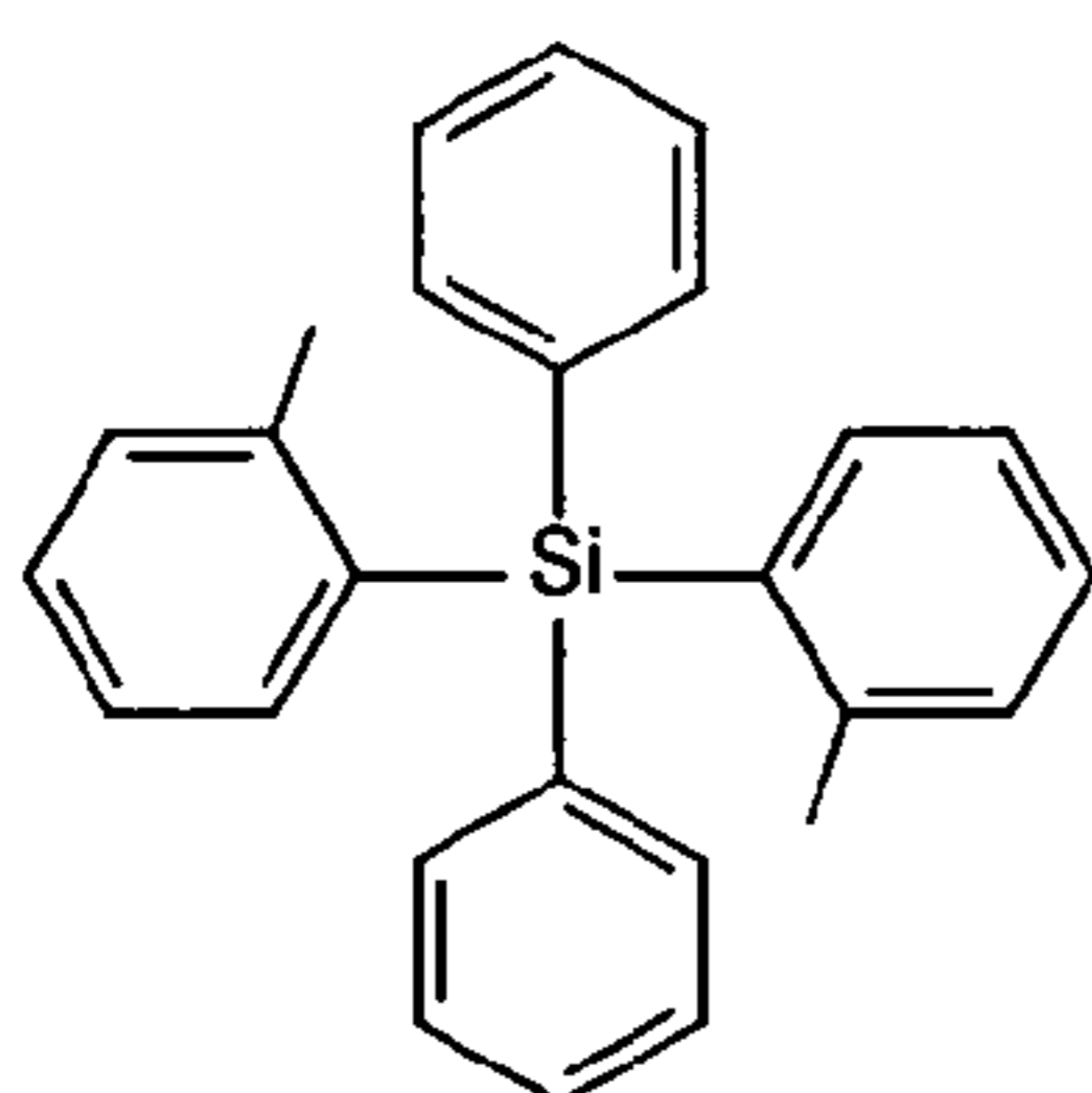
\text{Siph}_2(\text{o-tolyl})_2
