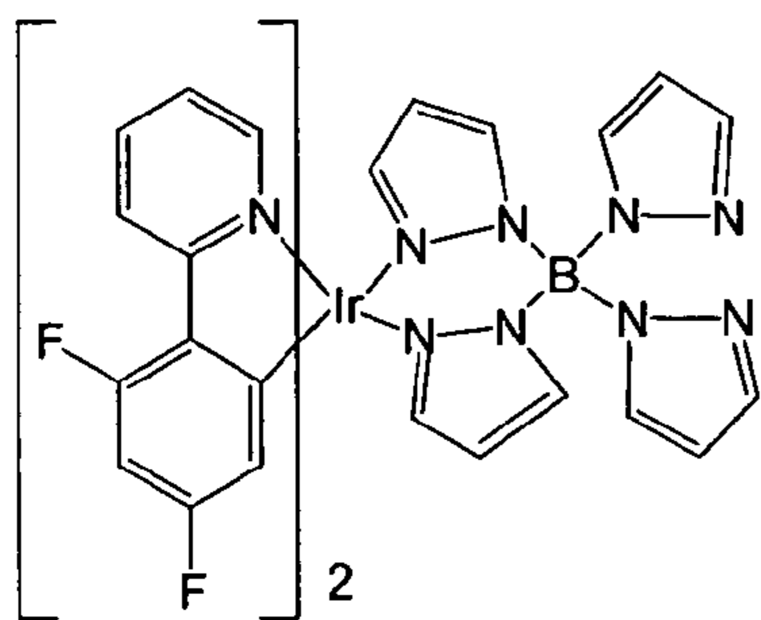
\text{Ir}(4,6\text{-F}_2\text{ppy})_2(\text{BPz}_4)
