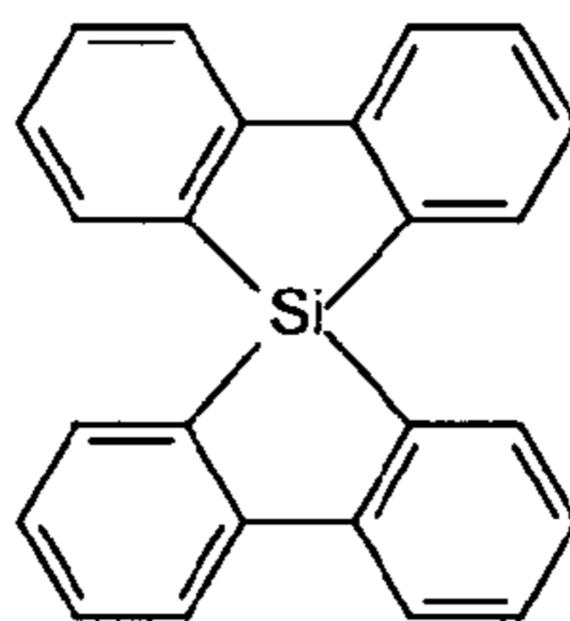
5,5'-Spirobi(dibenzosilole)
