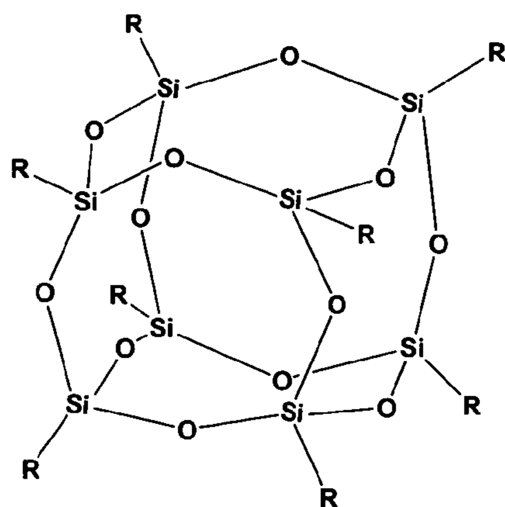
R: Phenyl
