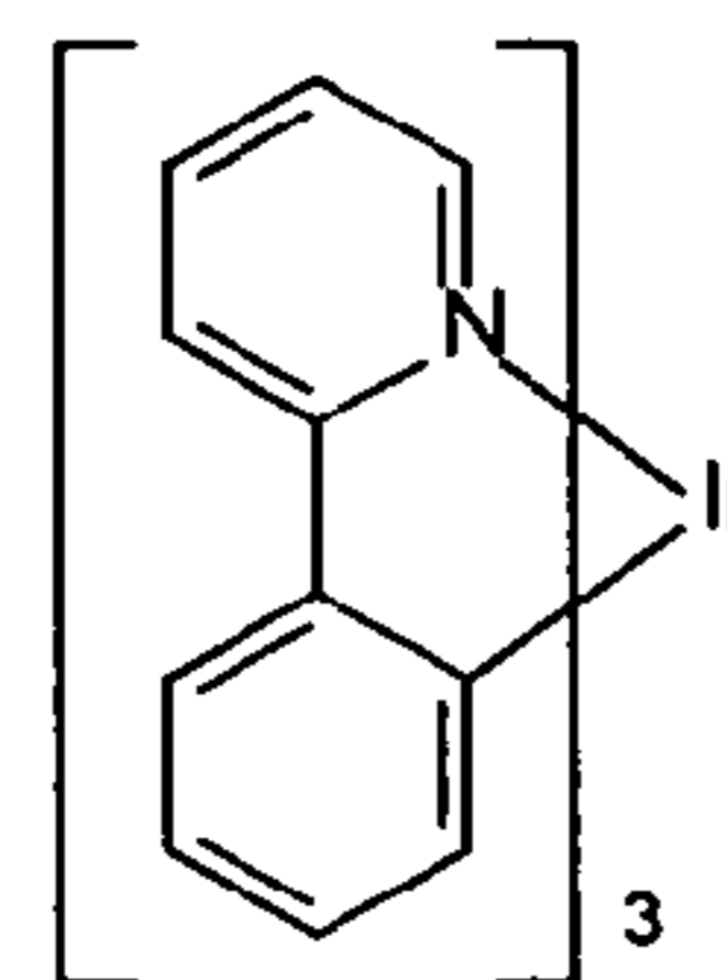
\text{Irppy}
