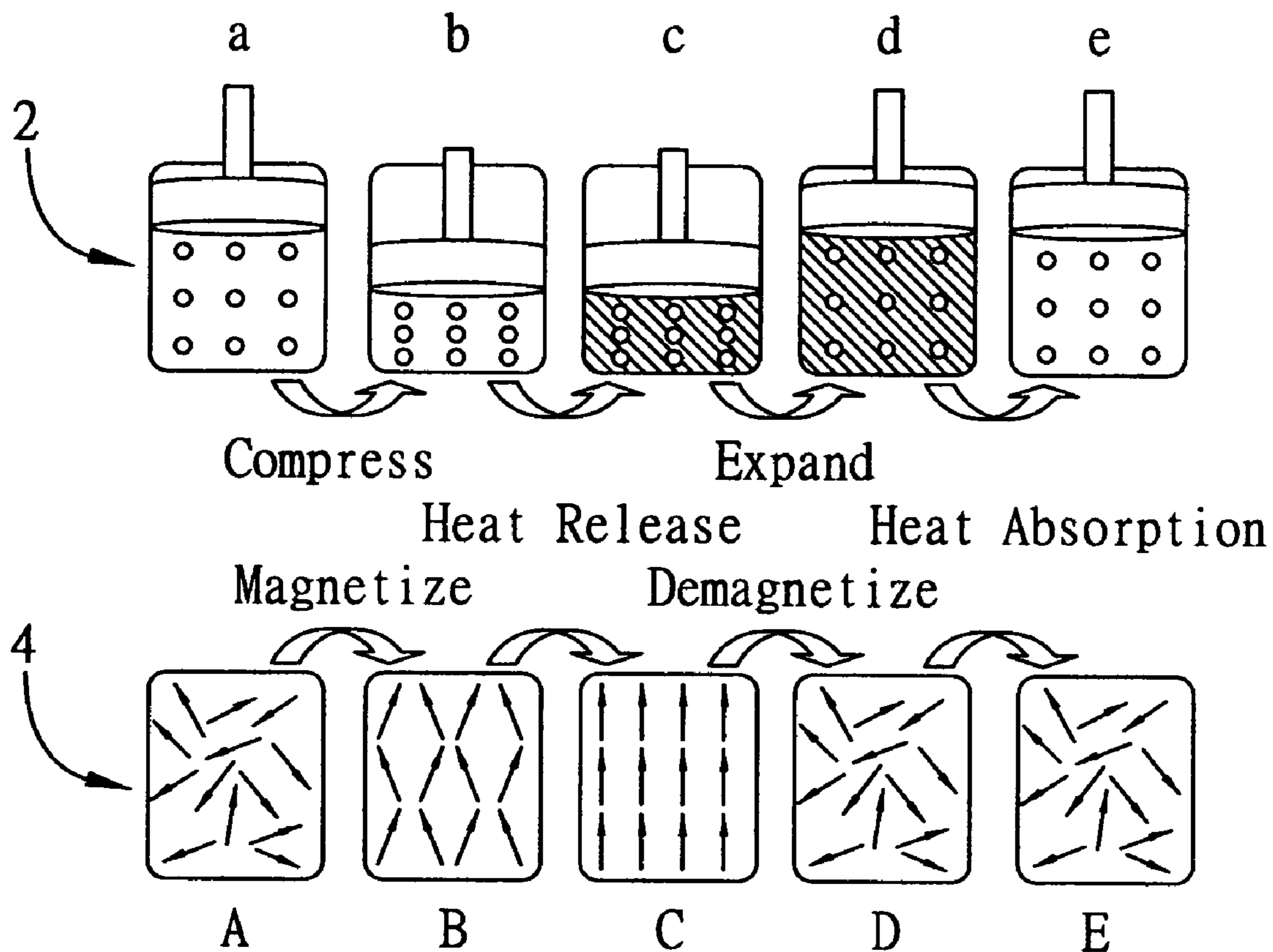
FIG. 10 (PRIOR ART)
