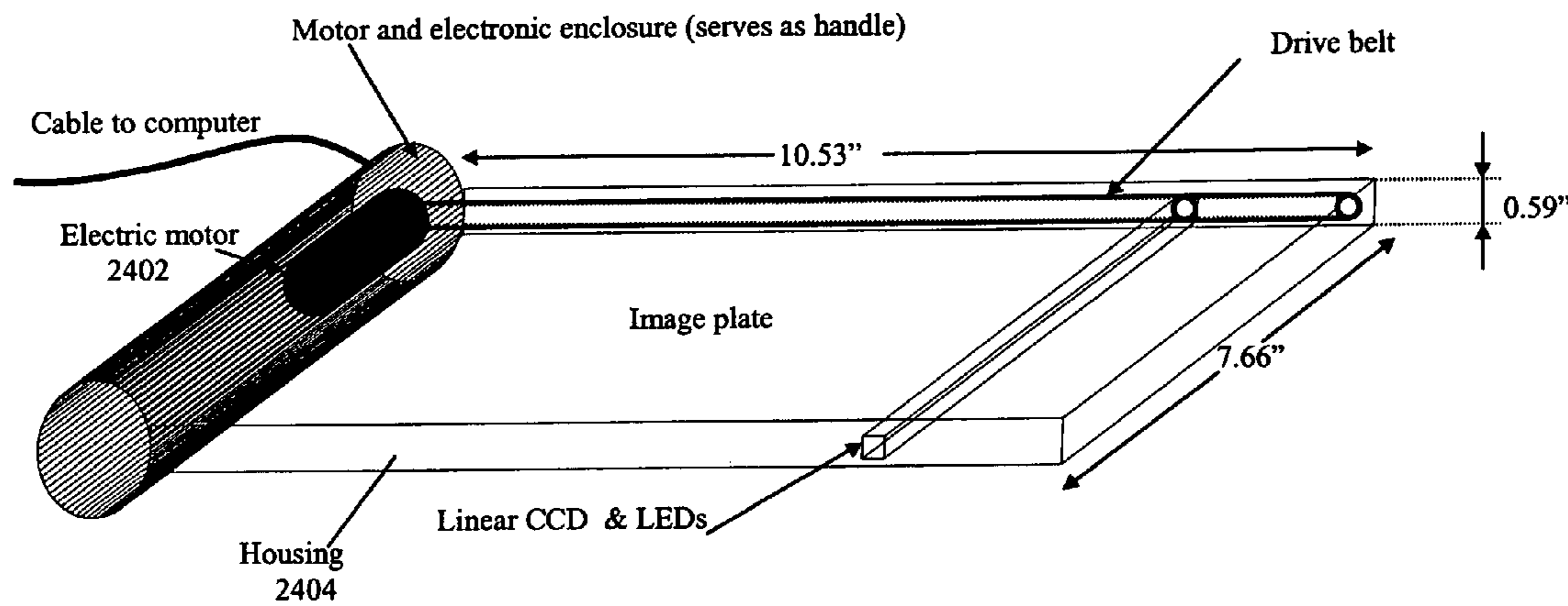
Mammography cassette enclosure (fits in standard 18cm x 24 cm bucky)
