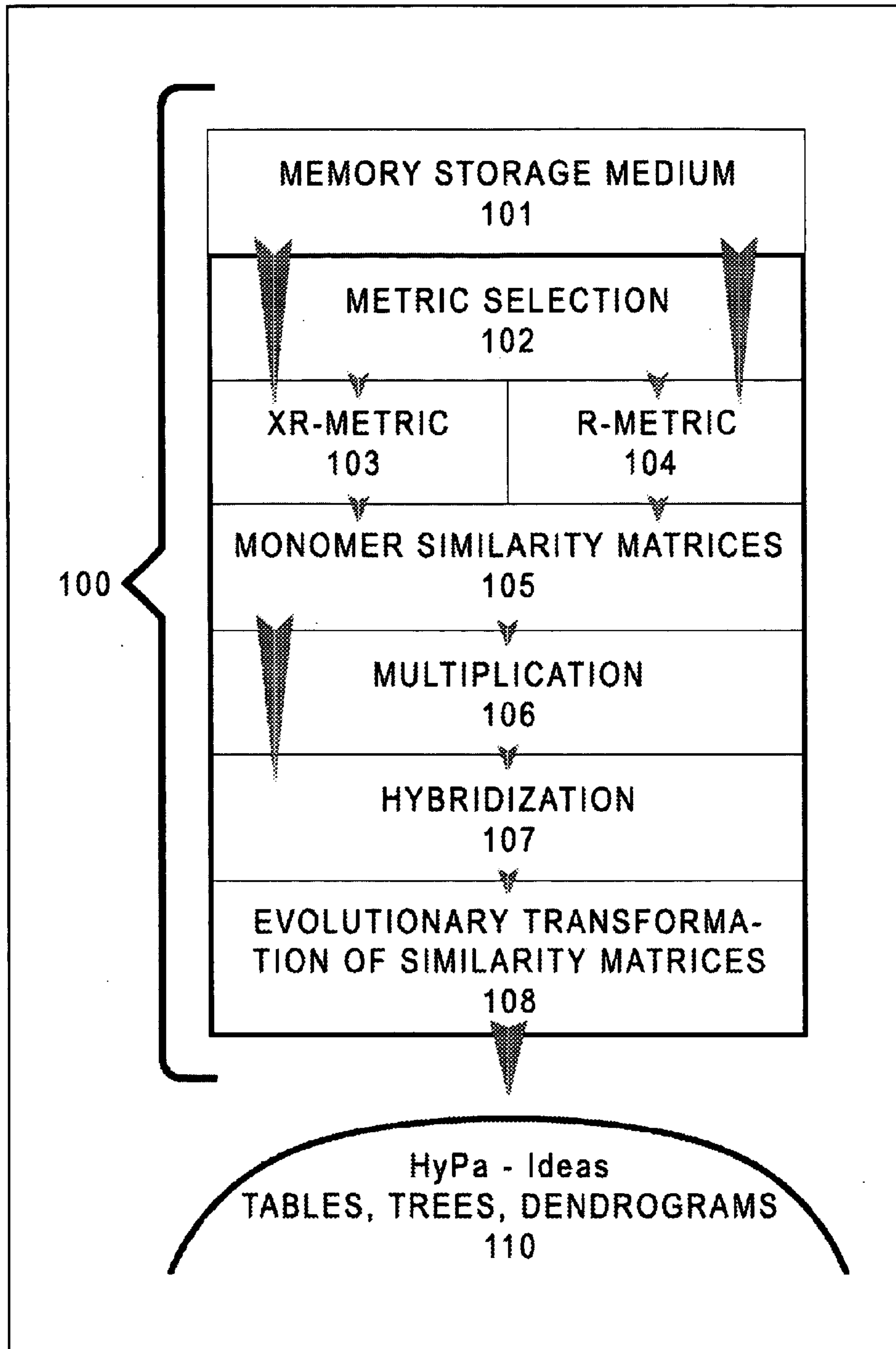
FIG. 1 A flow diagram of MeaningFinder™ algorithmic architecture
