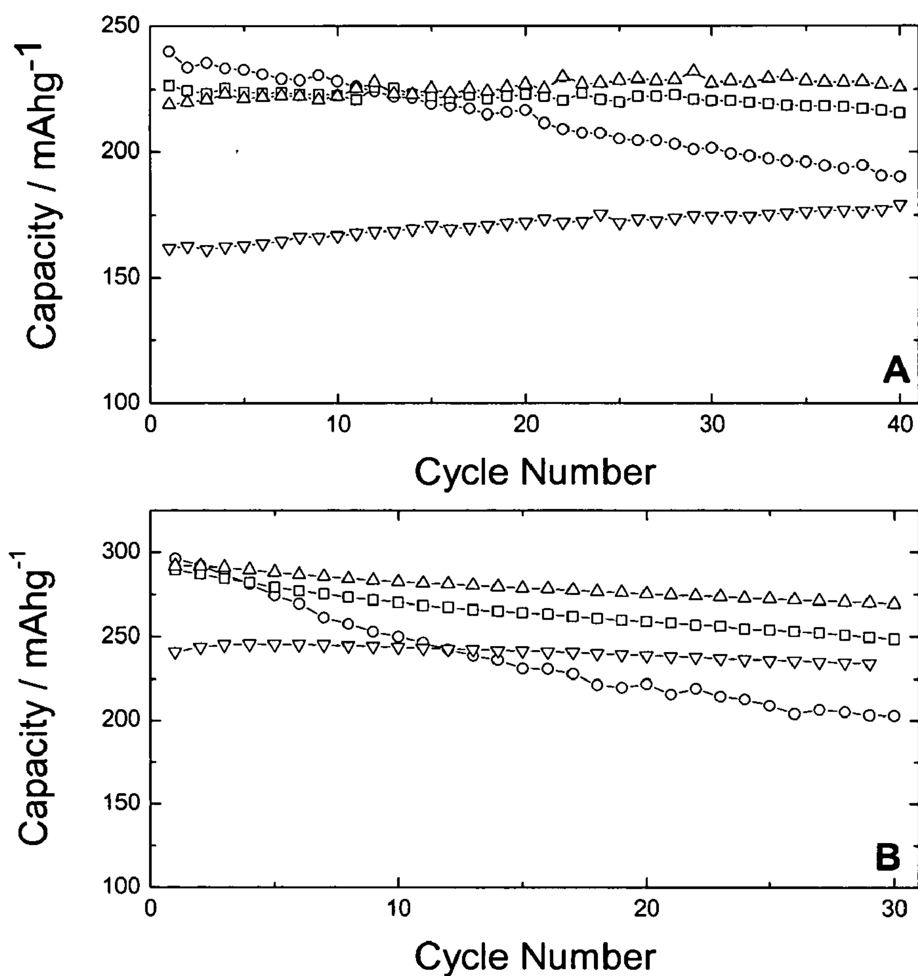
Figure 16. Cycling performance of \text{Li/Li}_{1+x}(\text{Ni}_{\alpha}\text{Mn}_{\beta}\text{Co}_{\gamma})\text{O}_{2-z}\text{F}_z cells at room tempearture (A) and at 55°C (B).
